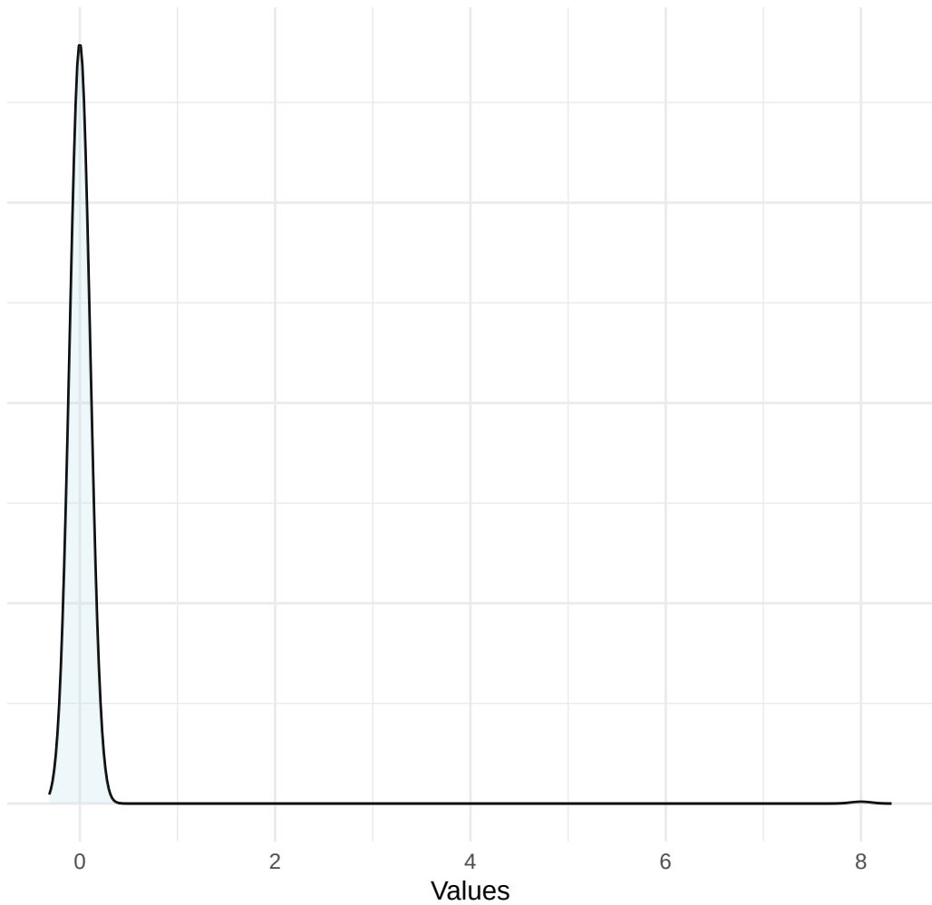
Density Plot for r.
