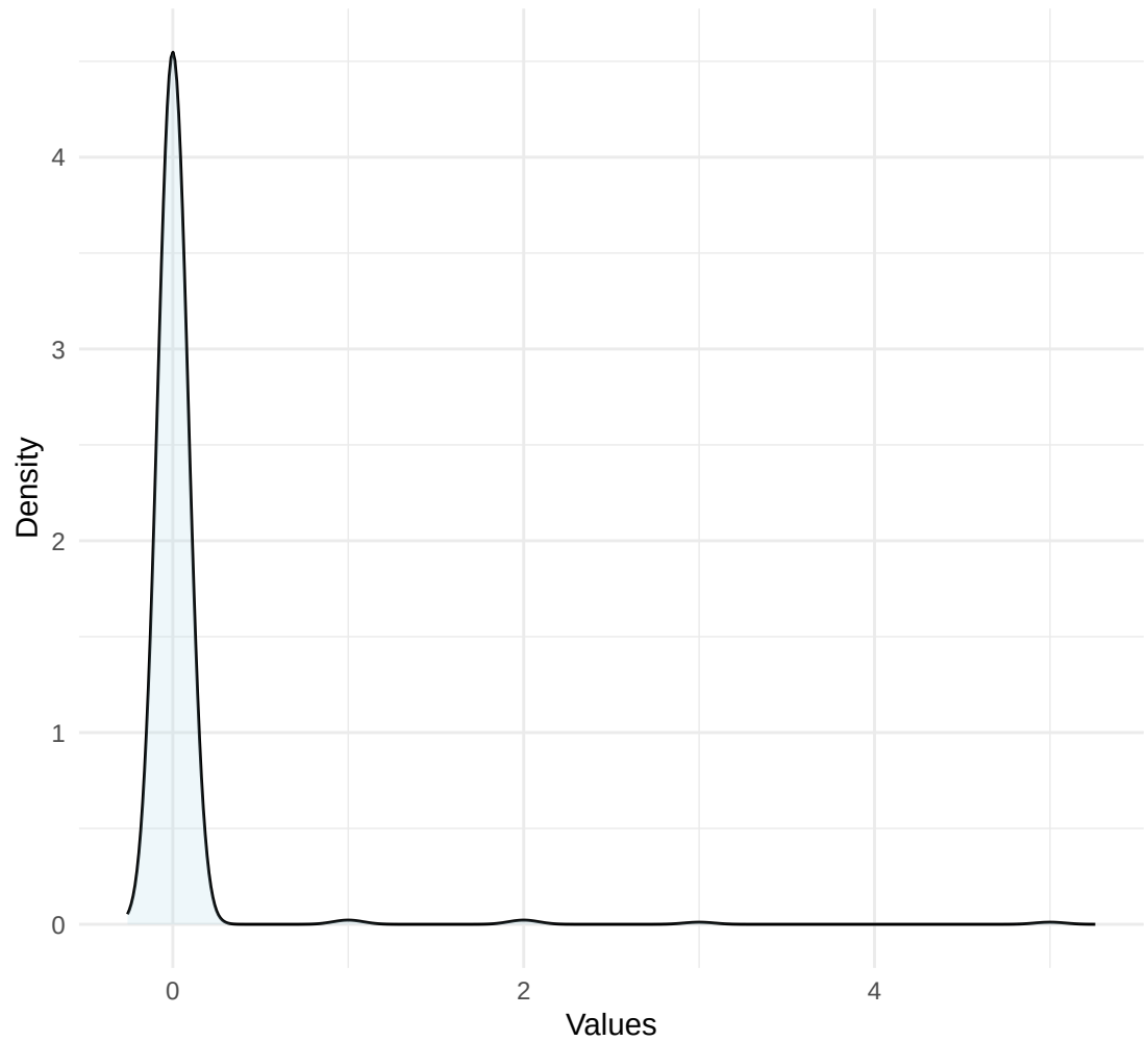
Density Plot for u.
