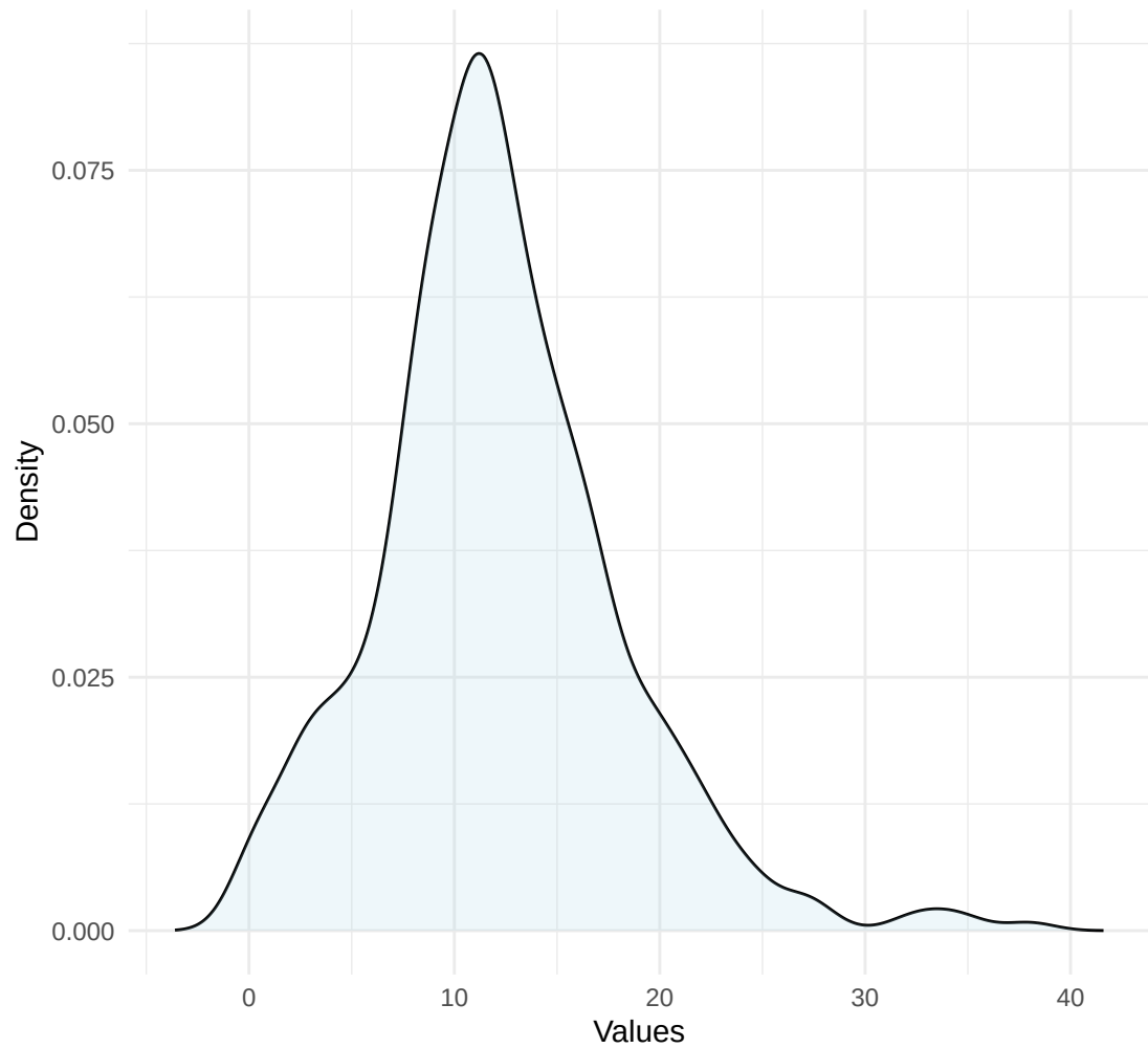
Density Plot for w
