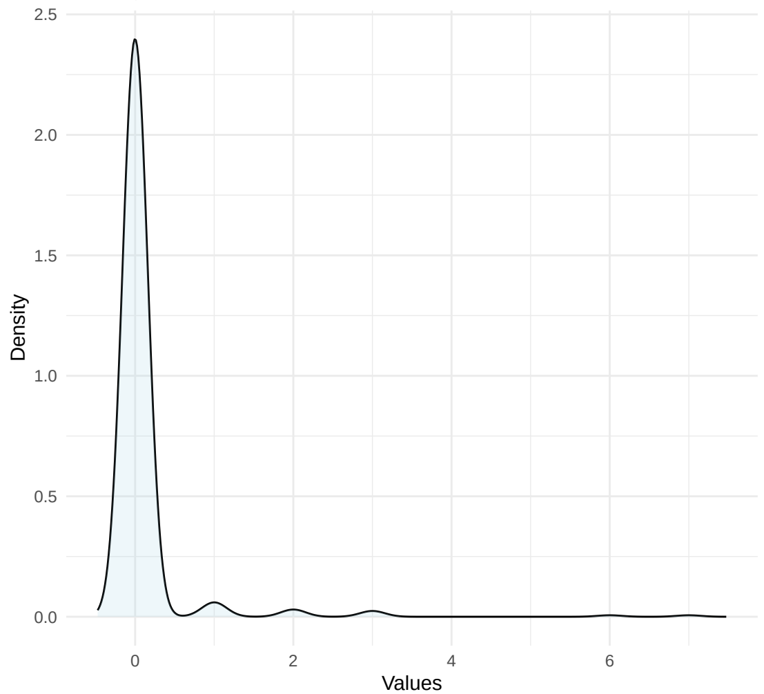
Density Plot for \tilde{a}
