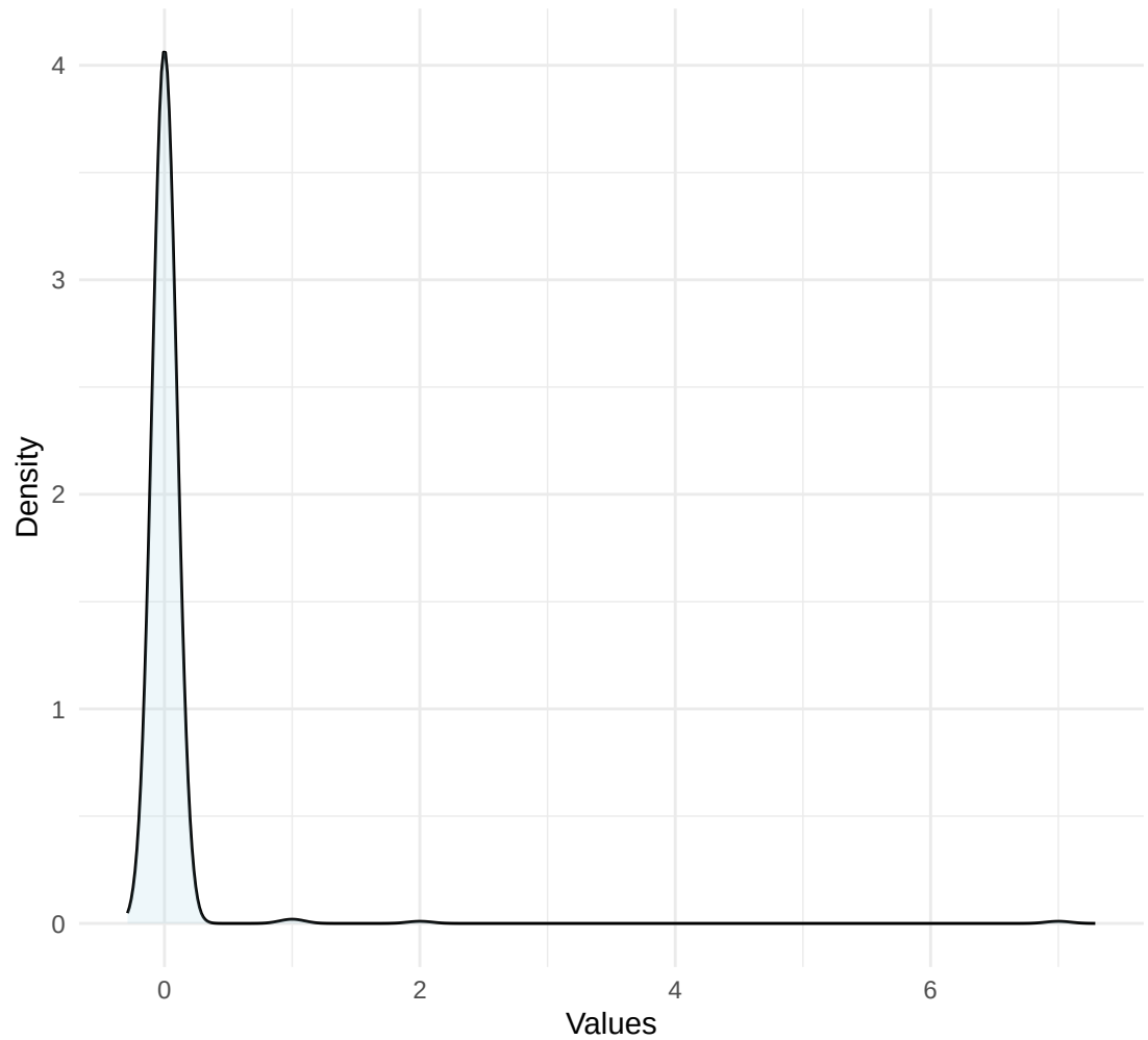
Density Plot for \alpha
