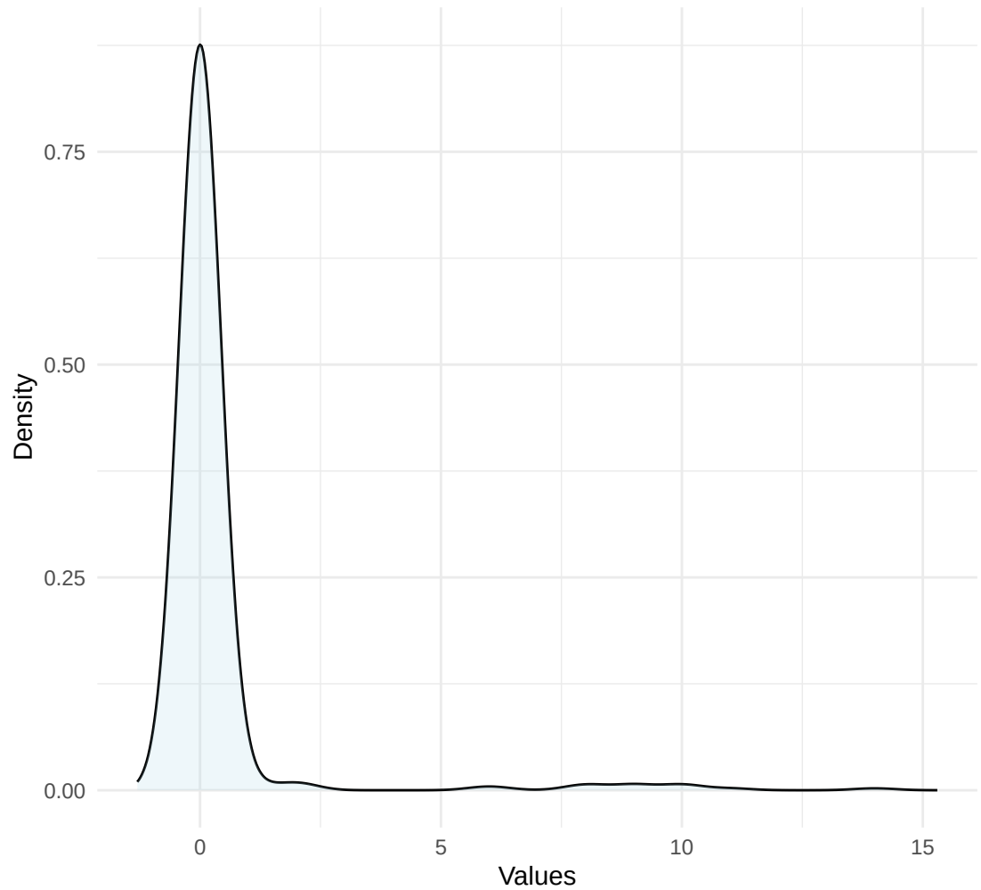
Density Plot for \check{\theta}
