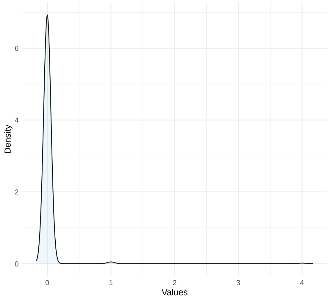
Density Plot for oe
