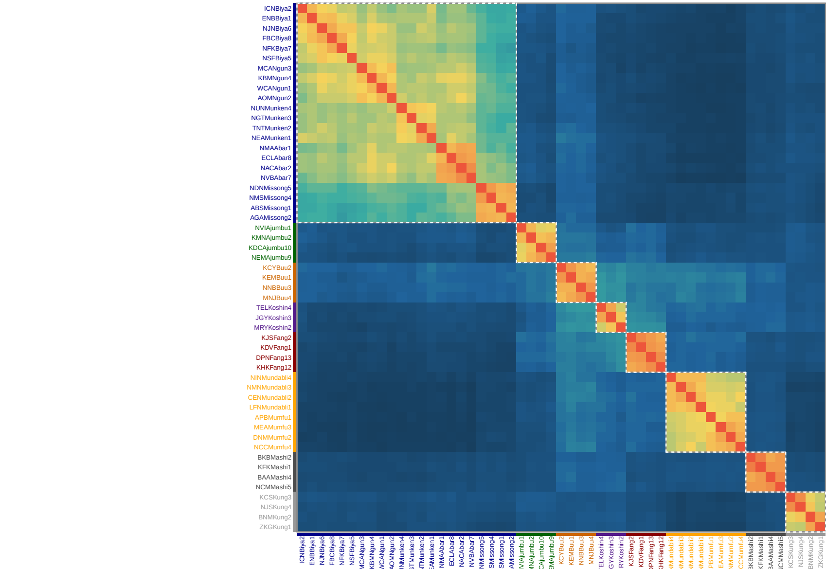
Lower Fungom closeness heatmap (modified full seriation: Kung/Mashi blocks)
