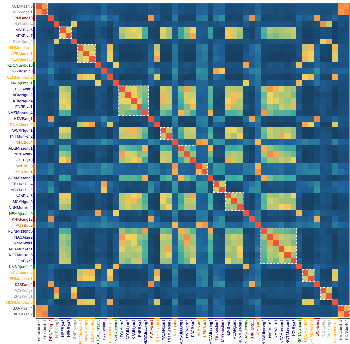
Lower Fungom closeness heatmap (full TSP-style seriation, no hclust)
