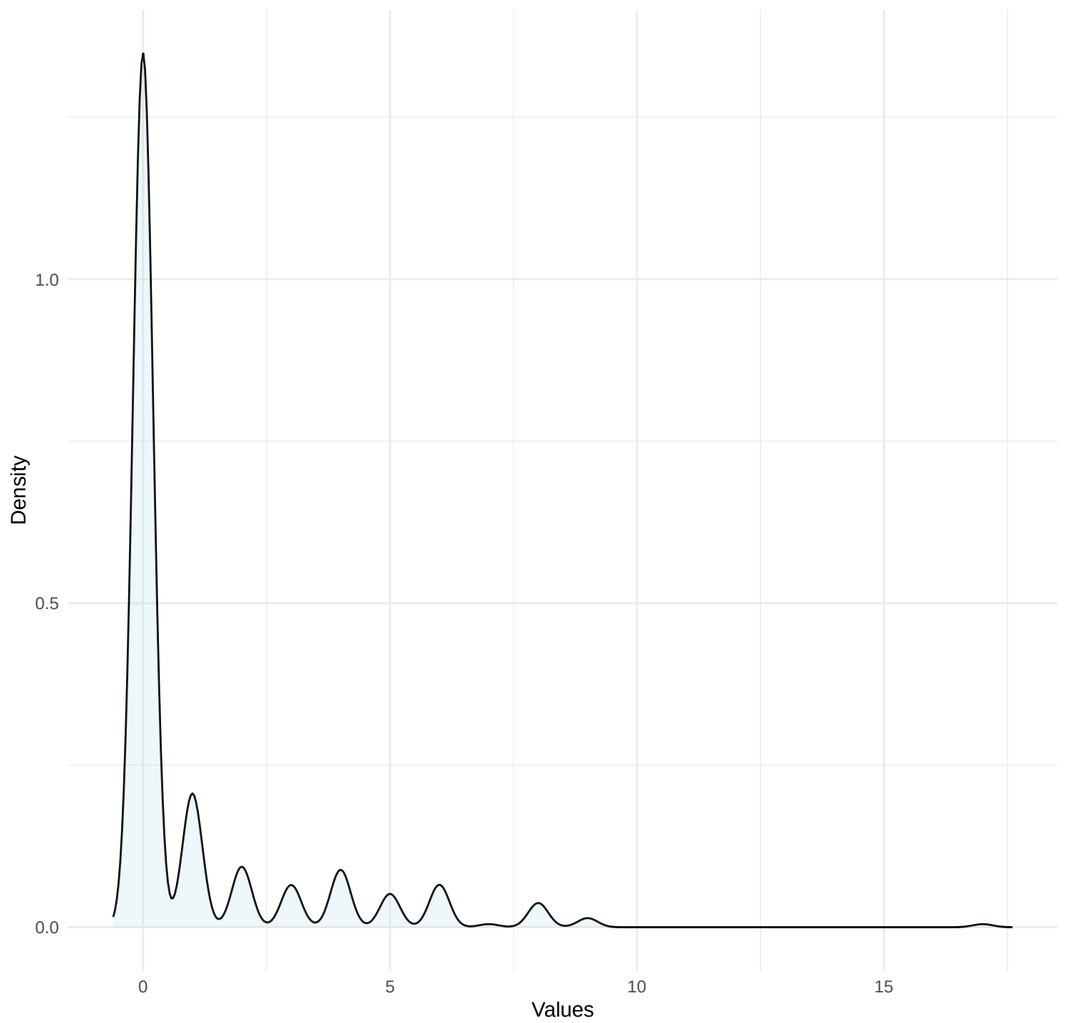
Density Plot for c
