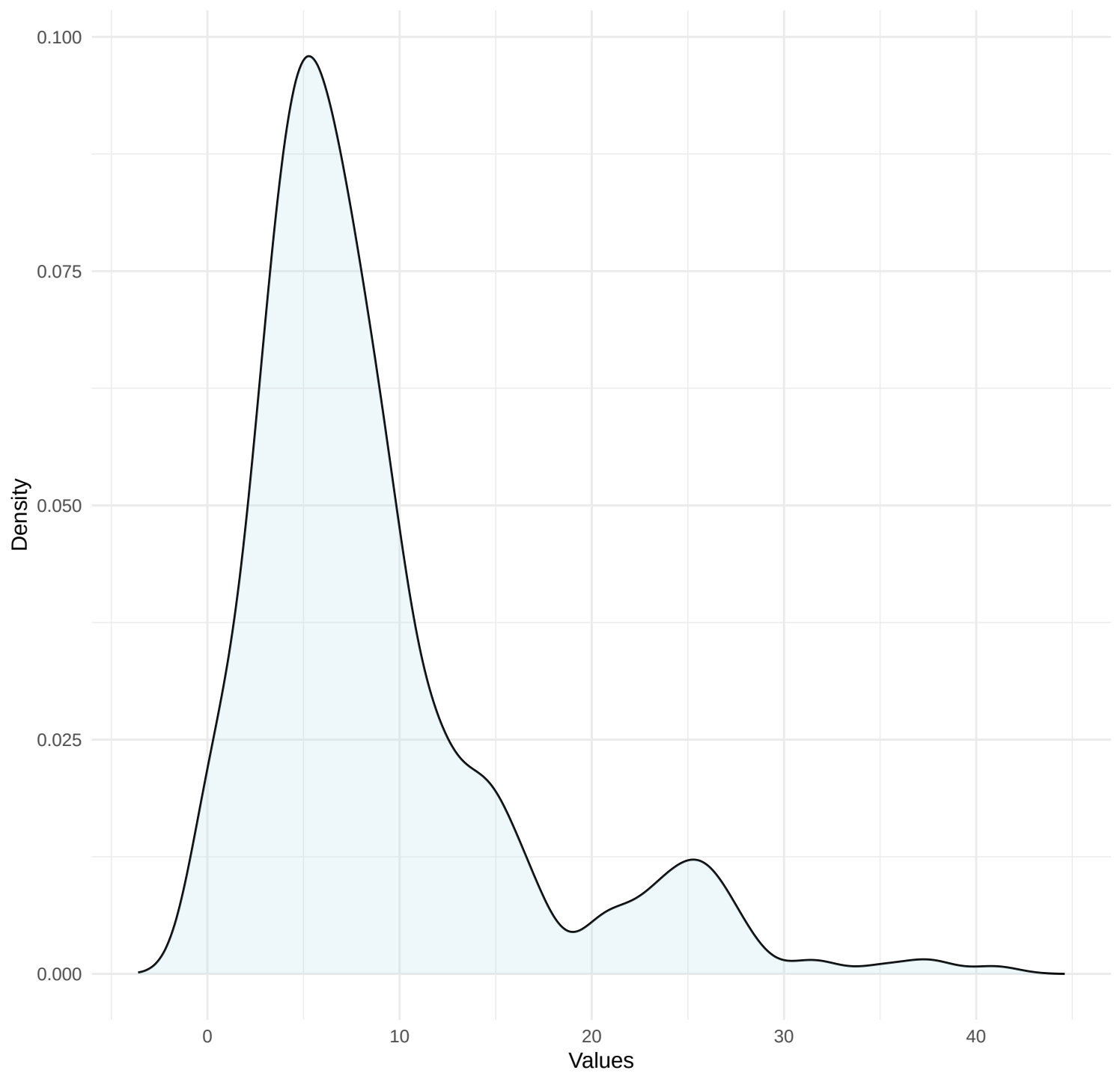
Density Plot for d
