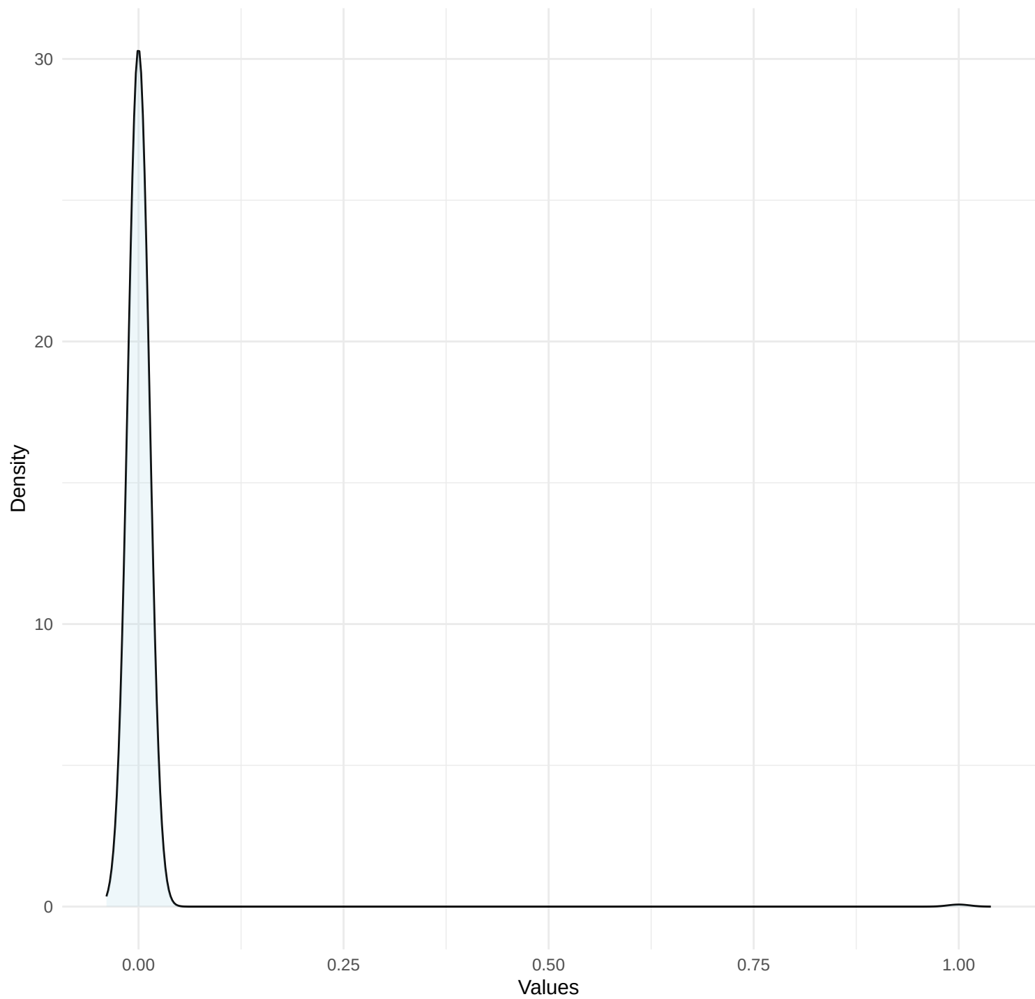
Density Plot for f.
