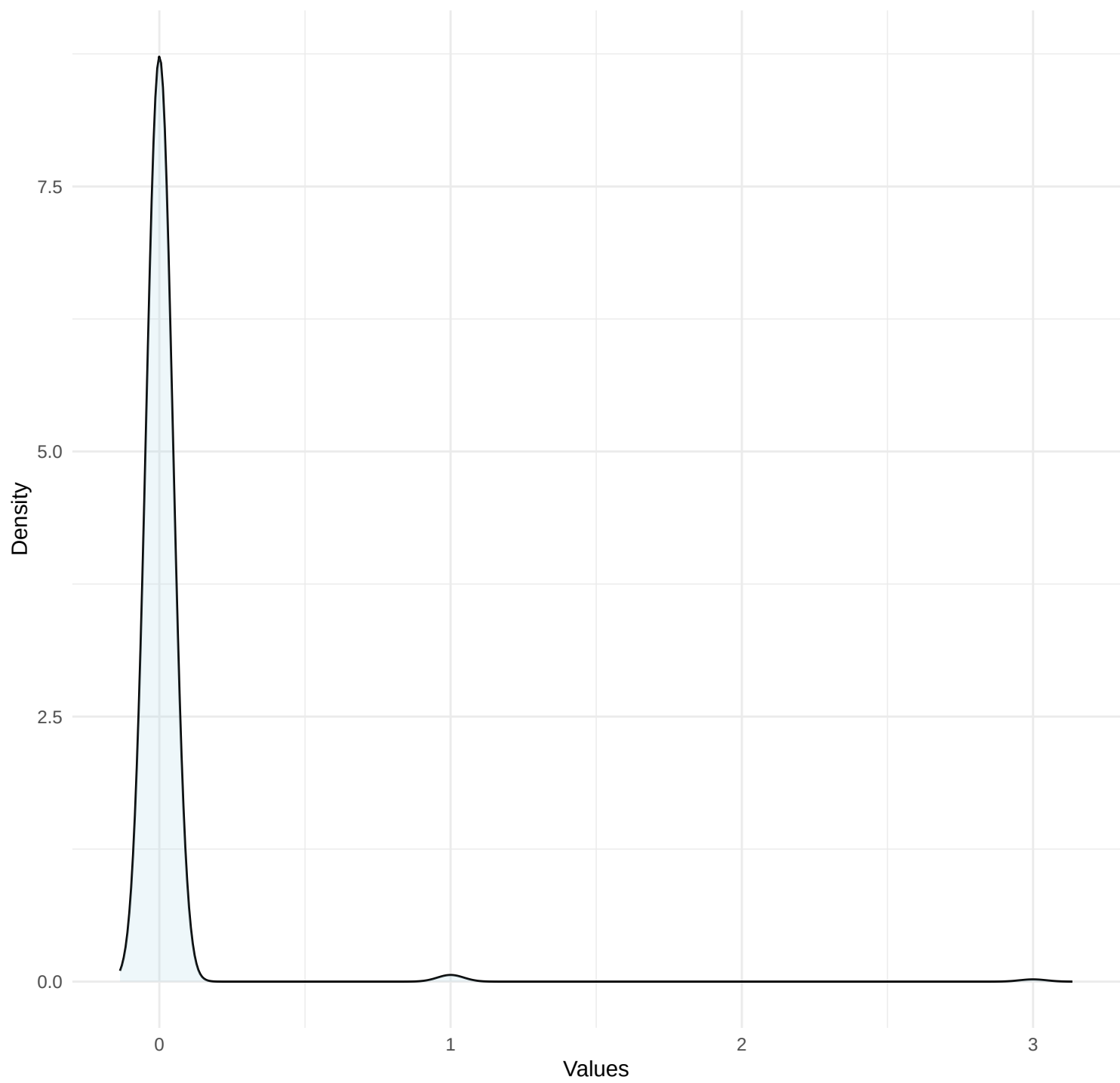
Density Plot for l.
