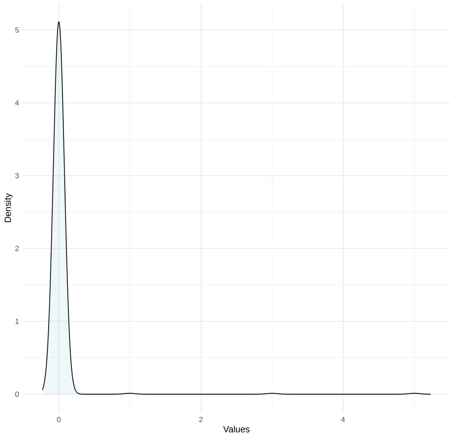
Density Plot for r.
