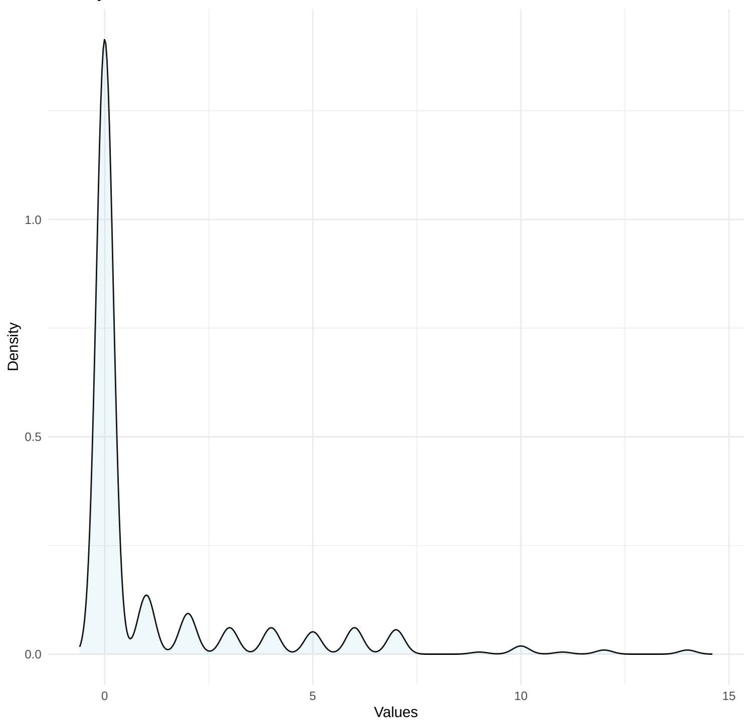
Density Plot for ts
