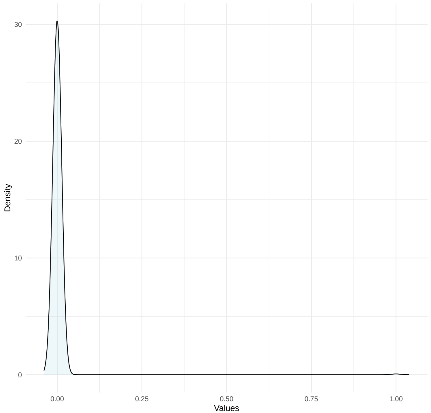
Density Plot for z.
