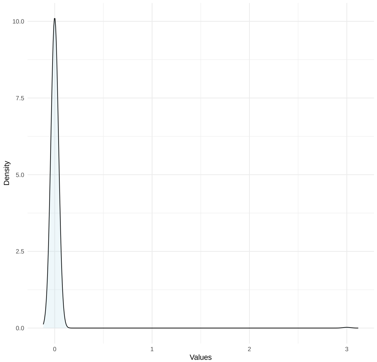
Density Plot for \tilde{a} .
