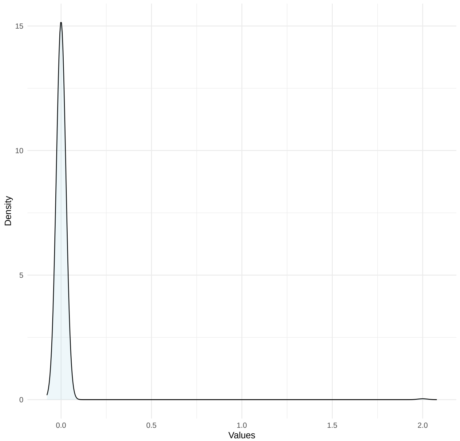
Density Plot for æ.
