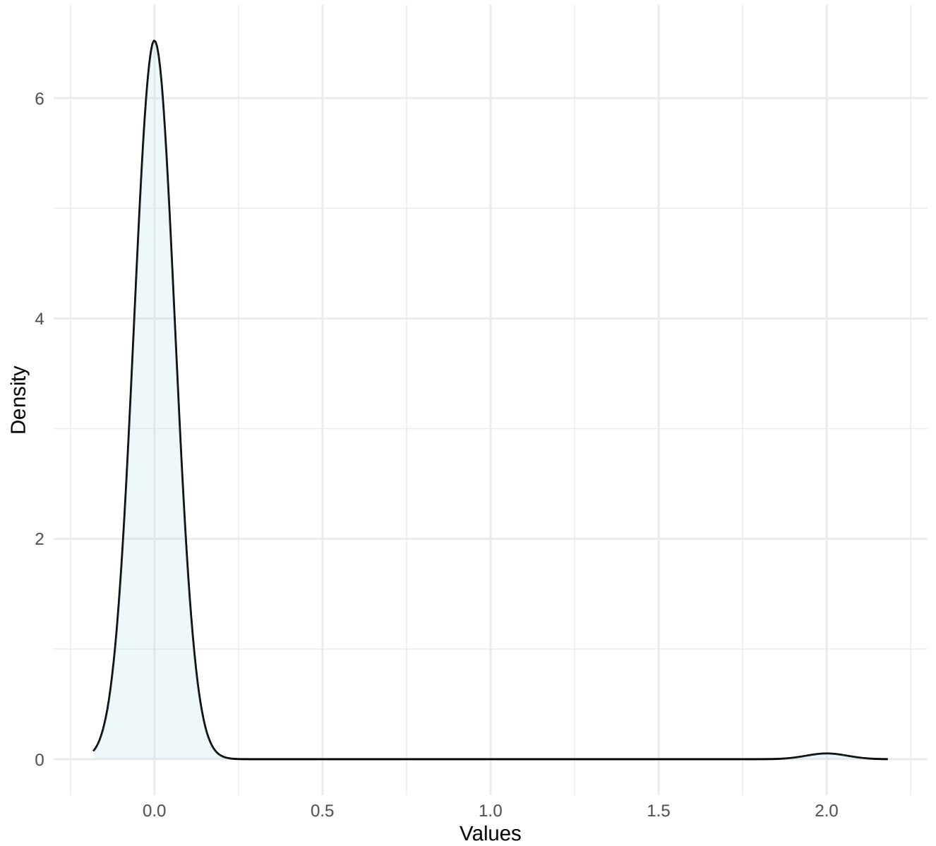
Density Plot for oi
