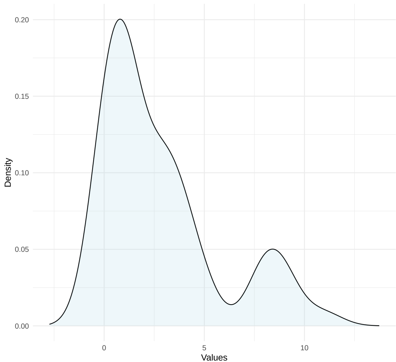
Density Plot for p
