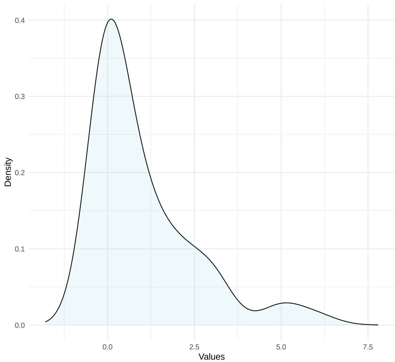
Density Plot for r
