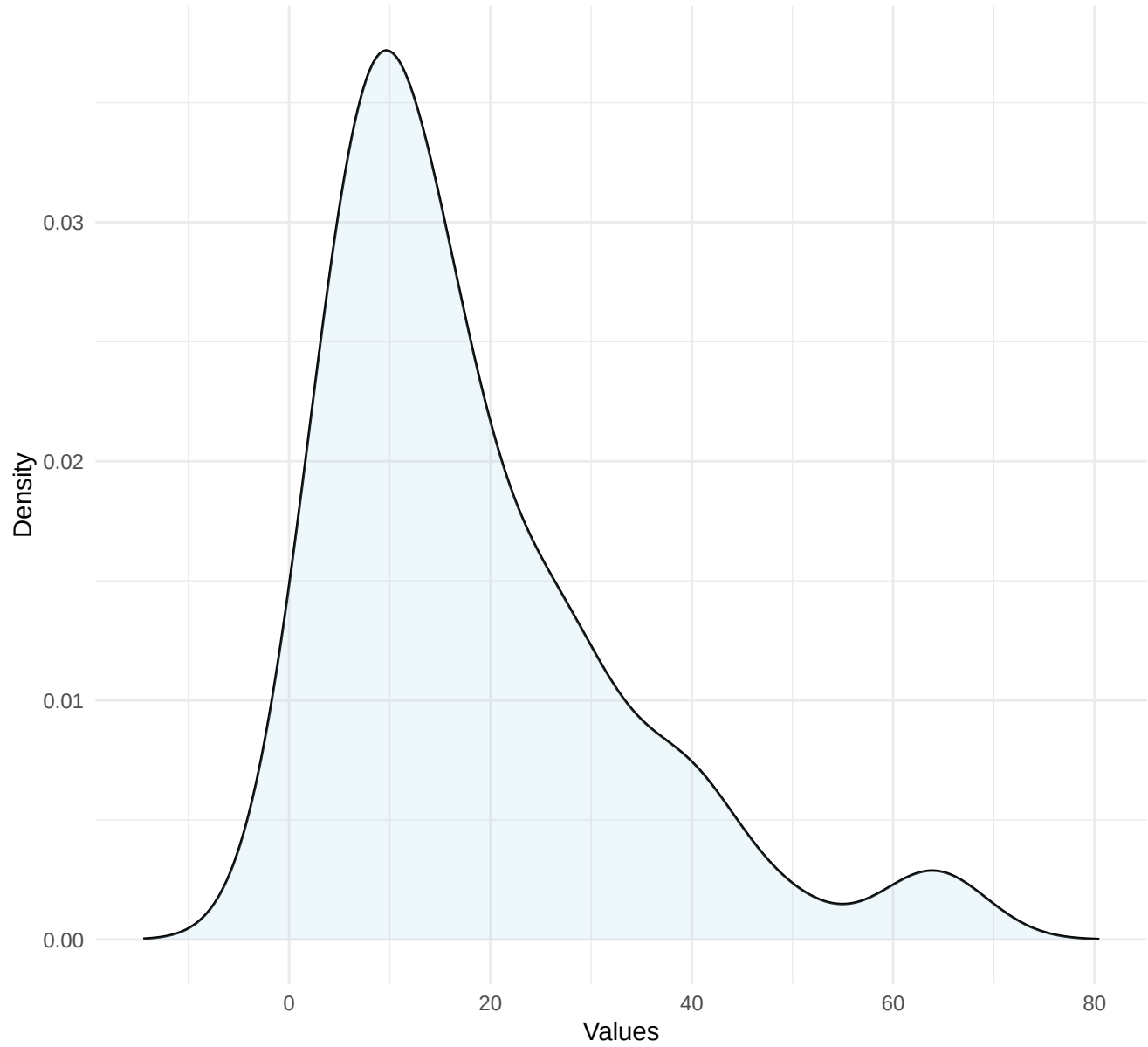
Density Plot for ts
