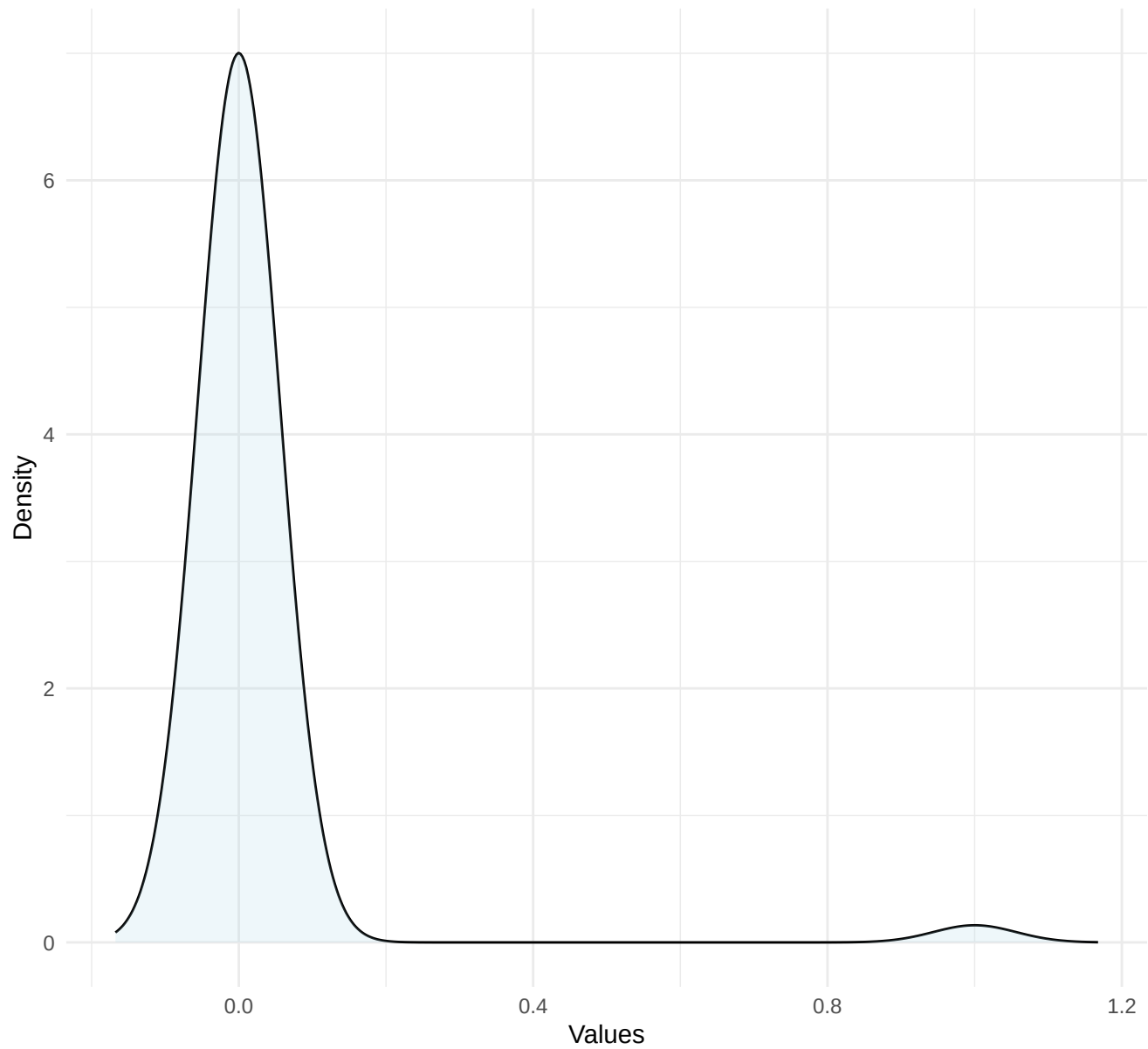
Density Plot for z.
