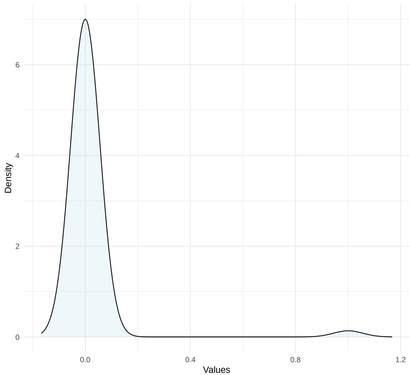
Density Plot for ^{21}
