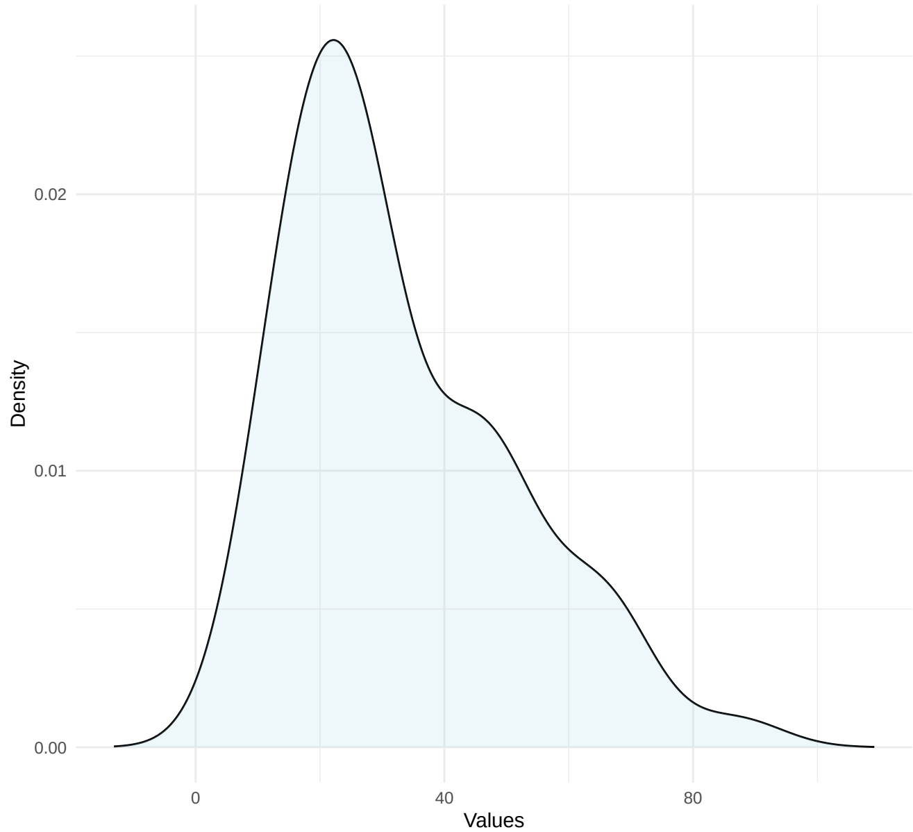
Density Plot for 1 .
