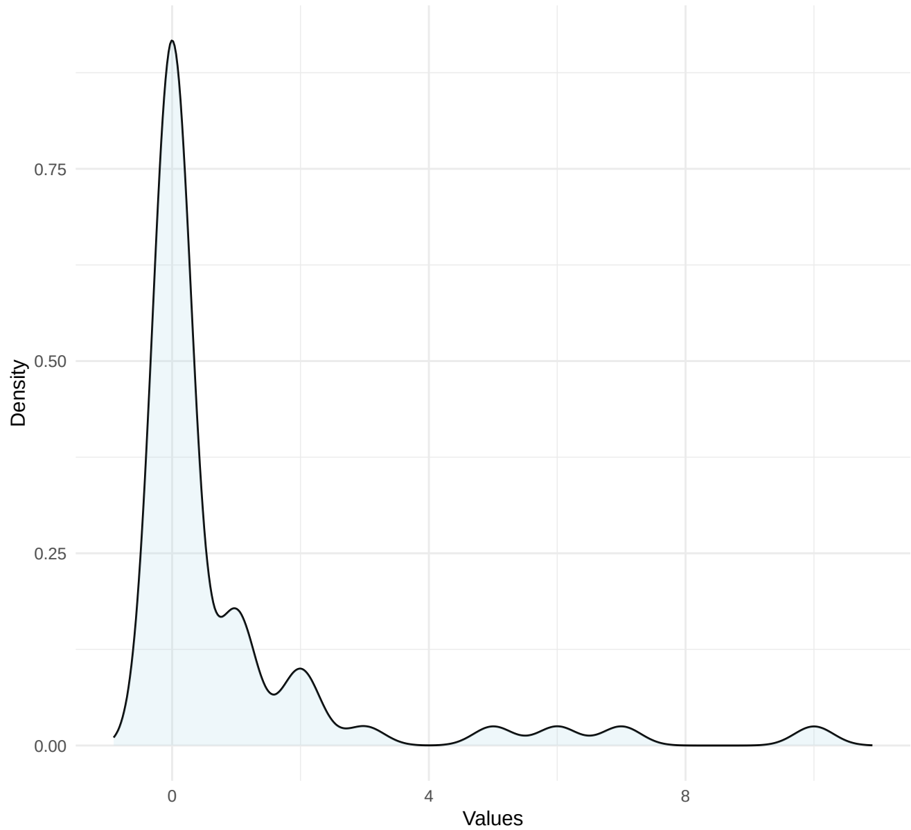
Density Plot for \tilde{a}
