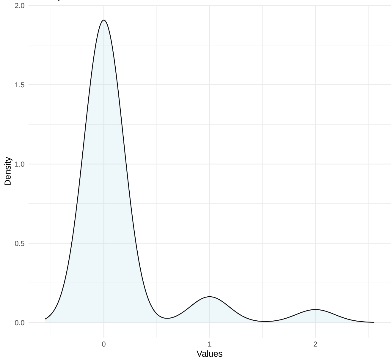
Density Plot for \hat{a} .
