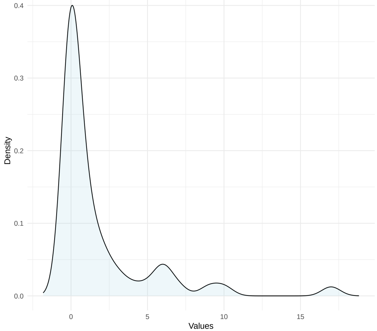
Density Plot for \varnothing
