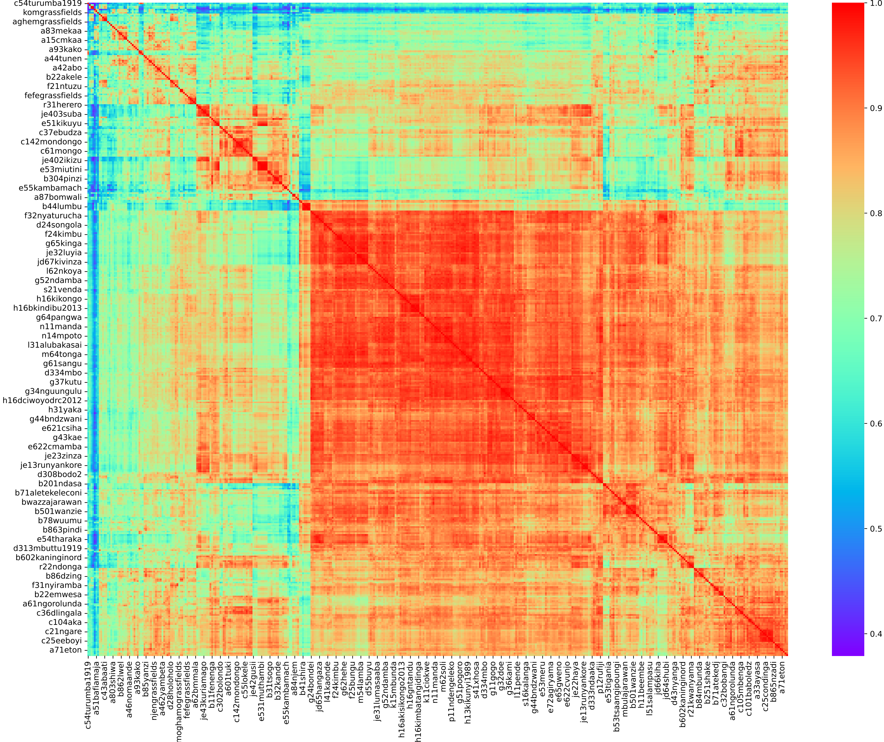
Reordered Heatmap of segmentProfiles-TLS.tsv (Similarities)
