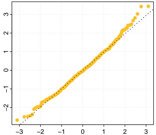
Theoretical Q. vs Std. Residuals
