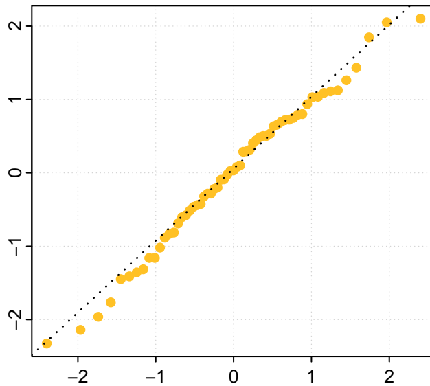
Theoretical Q. vs Std. Residuals
