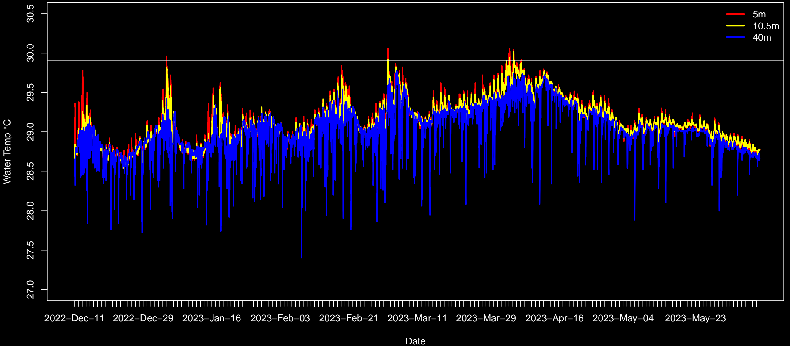
Fagatele Temperature Data
