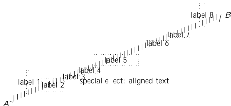
Figure 10: Rotations, scalings and clips
