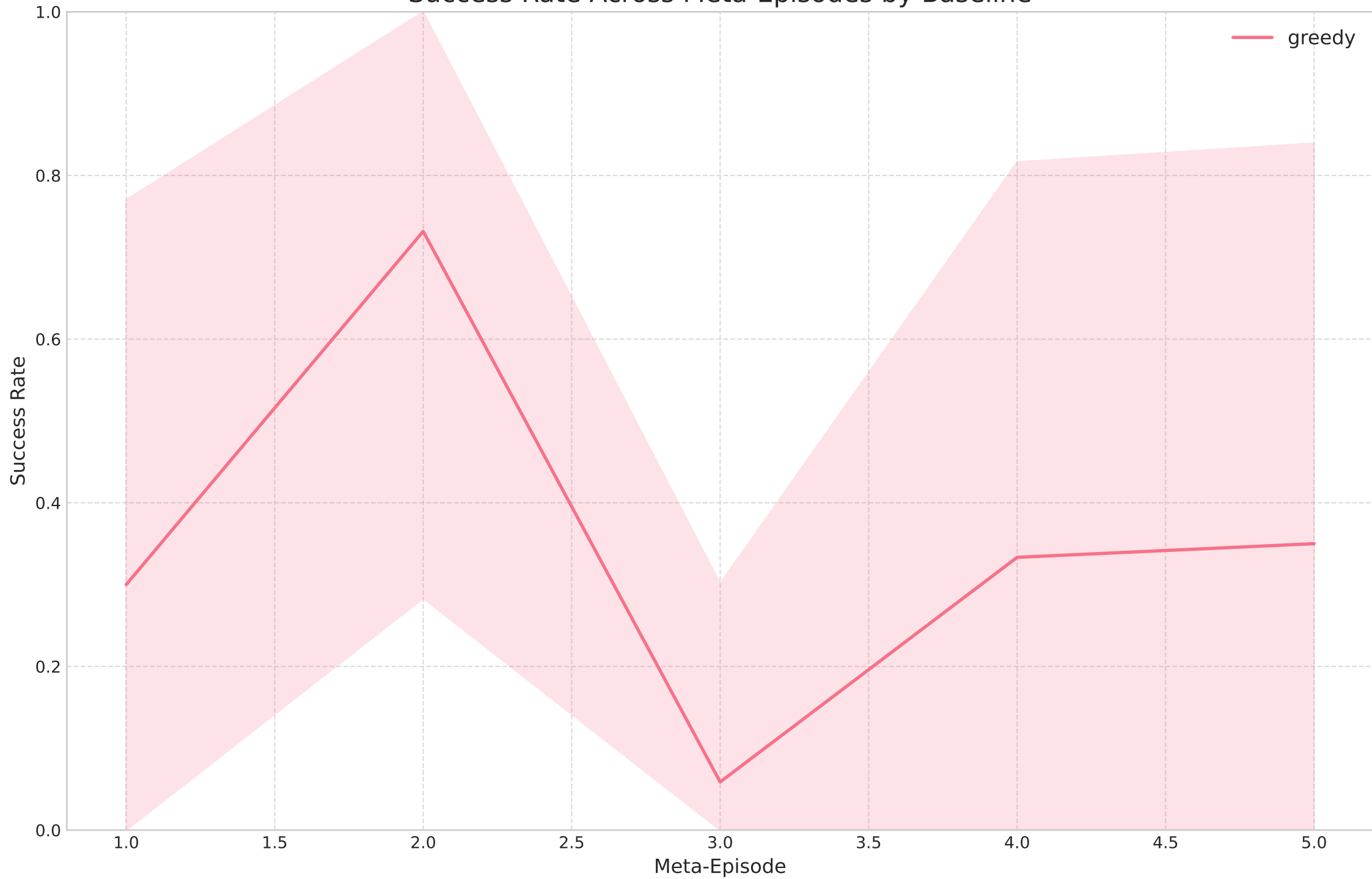
Success Rate Across Meta-Episodes by Baseline
