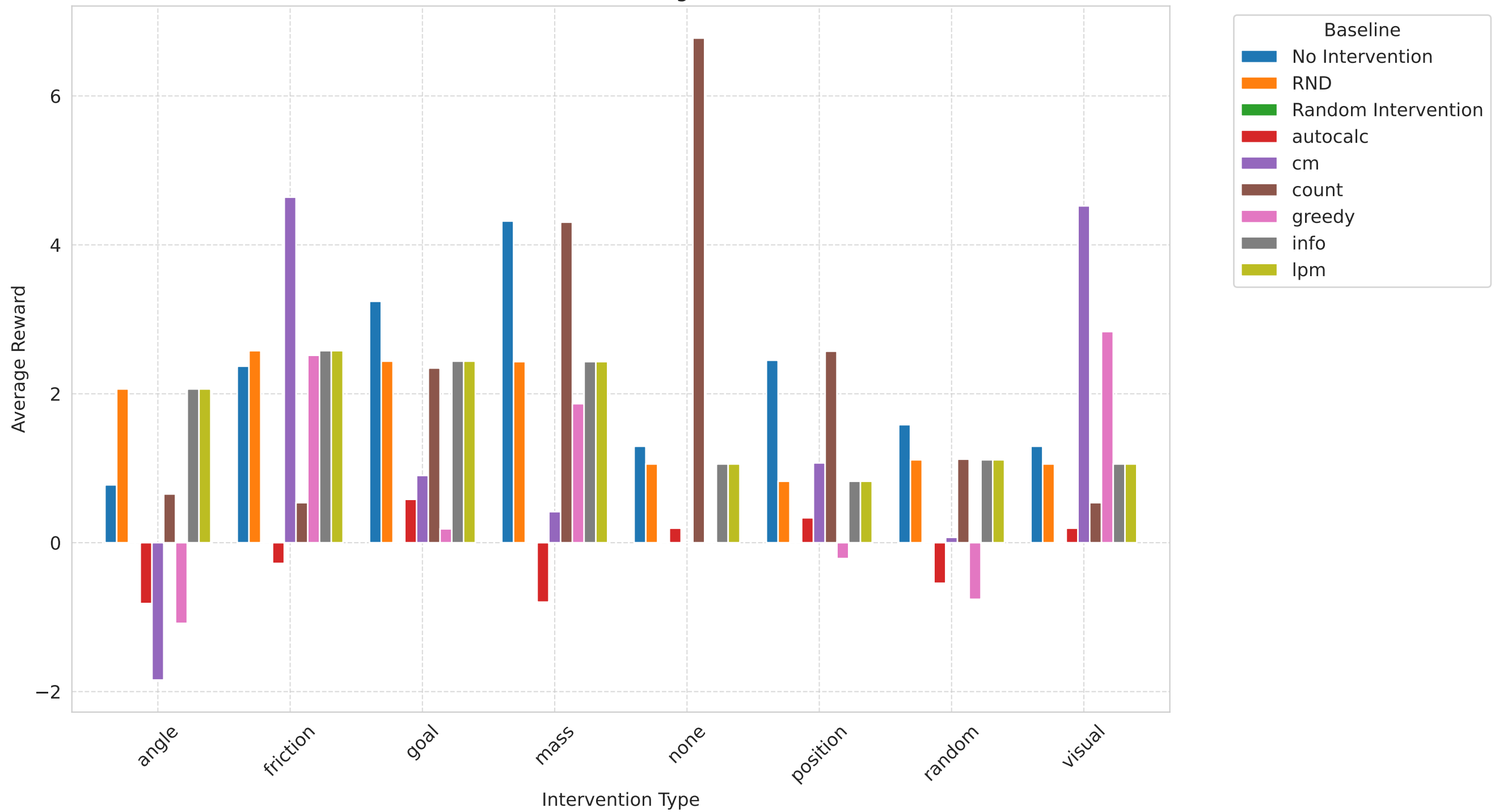
Intervention Test Effectiveness: Average Reward Across Baselines
