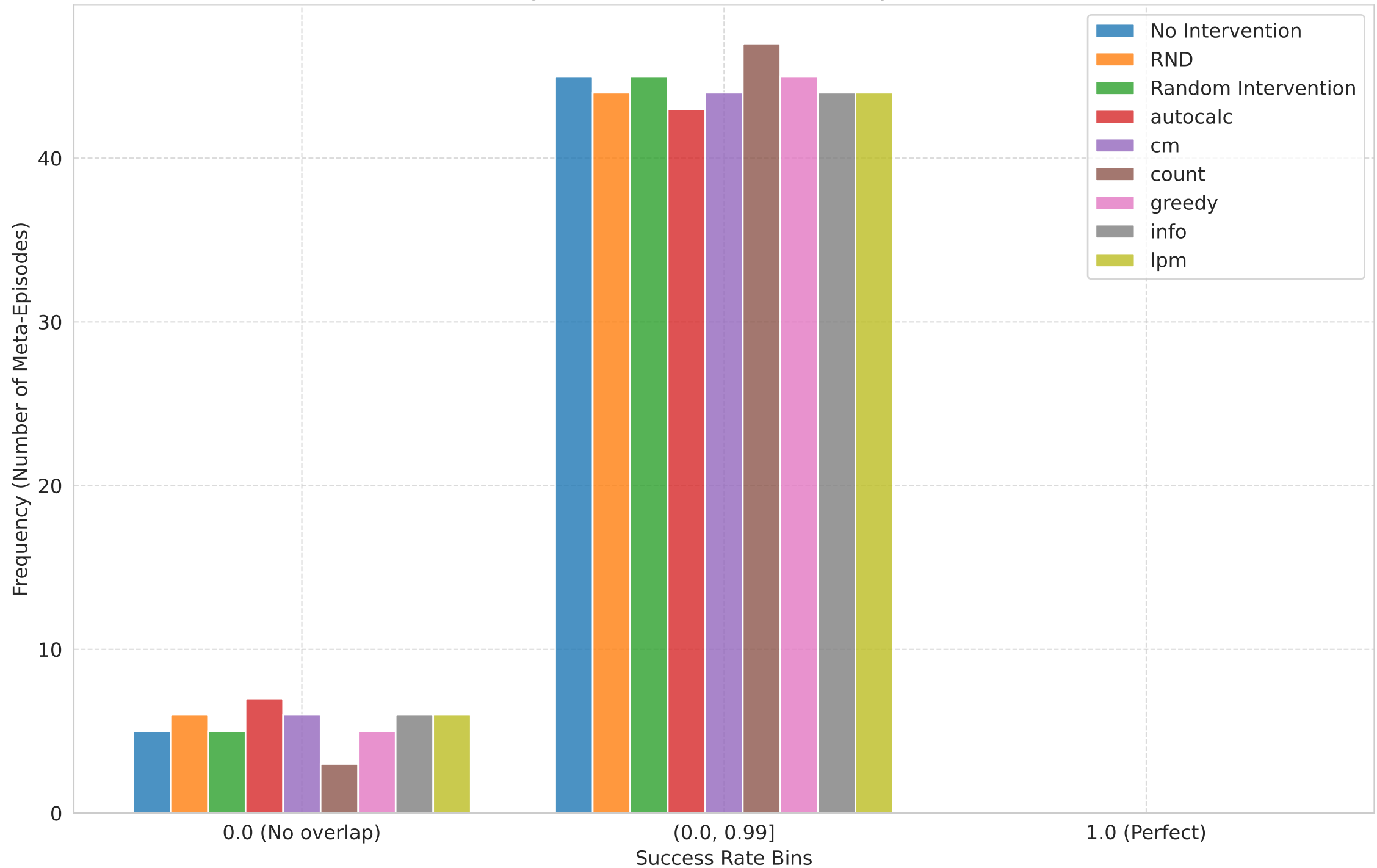
Training: Success Rate Distribution by Baseline
