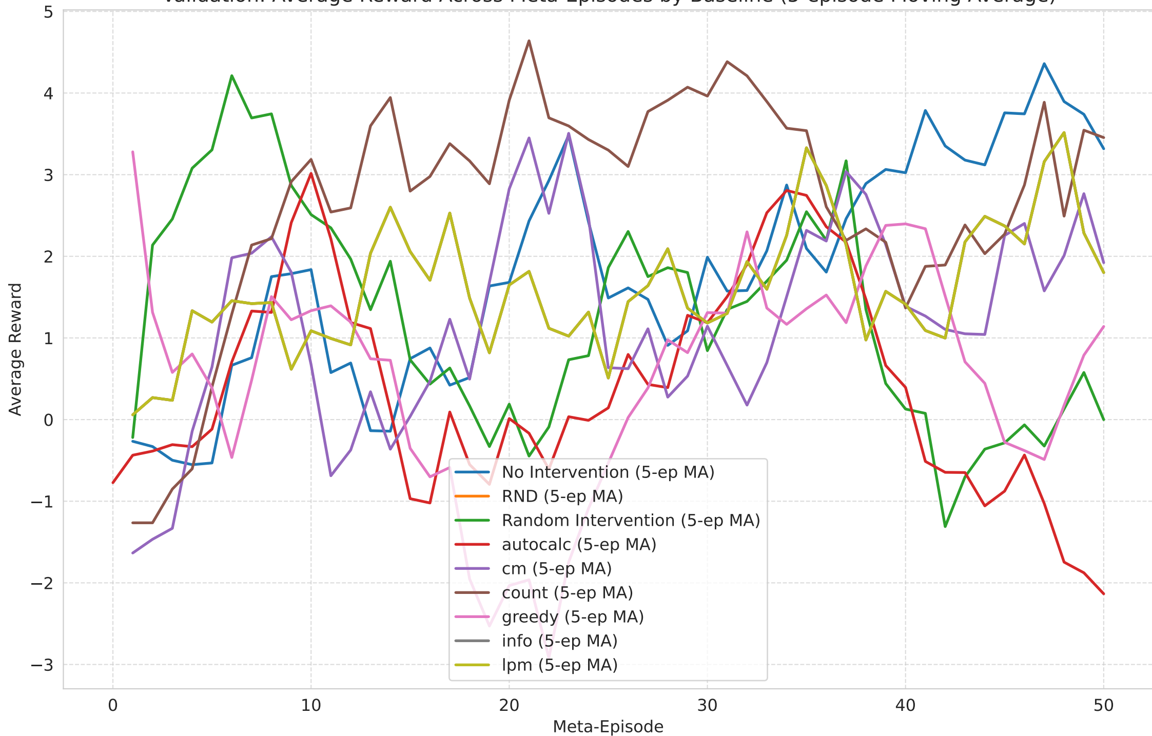
Validation: Average Reward Across Meta-Episodes by Baseline (5-episode Moving Average)
