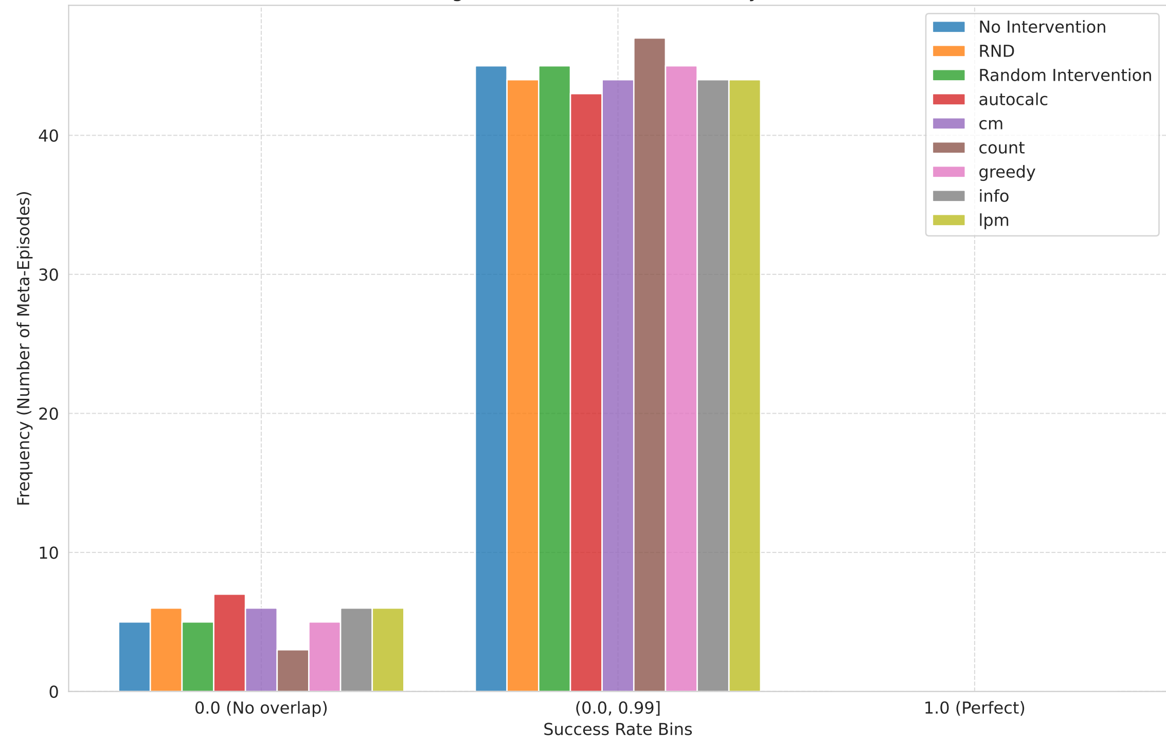
Training: Success Rate Distribution by Baseline
