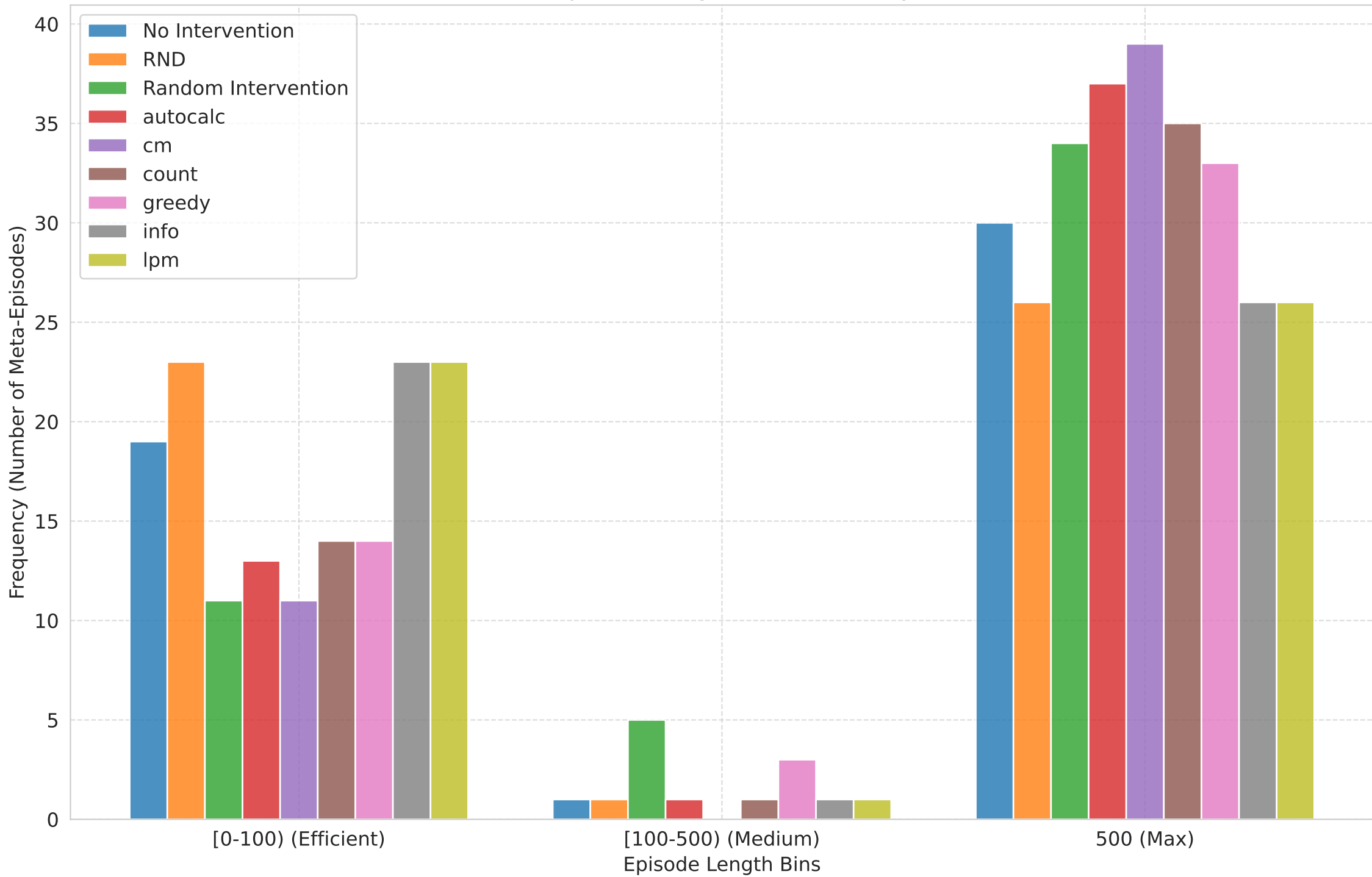
Validation: Episode Length Distribution by Baseline
