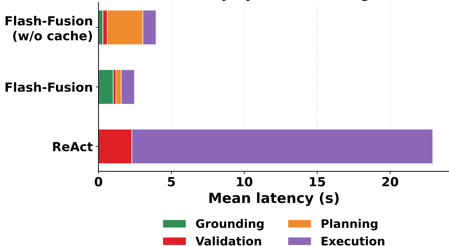
Latency by semantic stage
