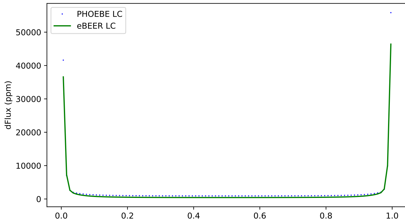
270 - ecc:0.8, incl:30, \omega :0, Porb:1, q:1
