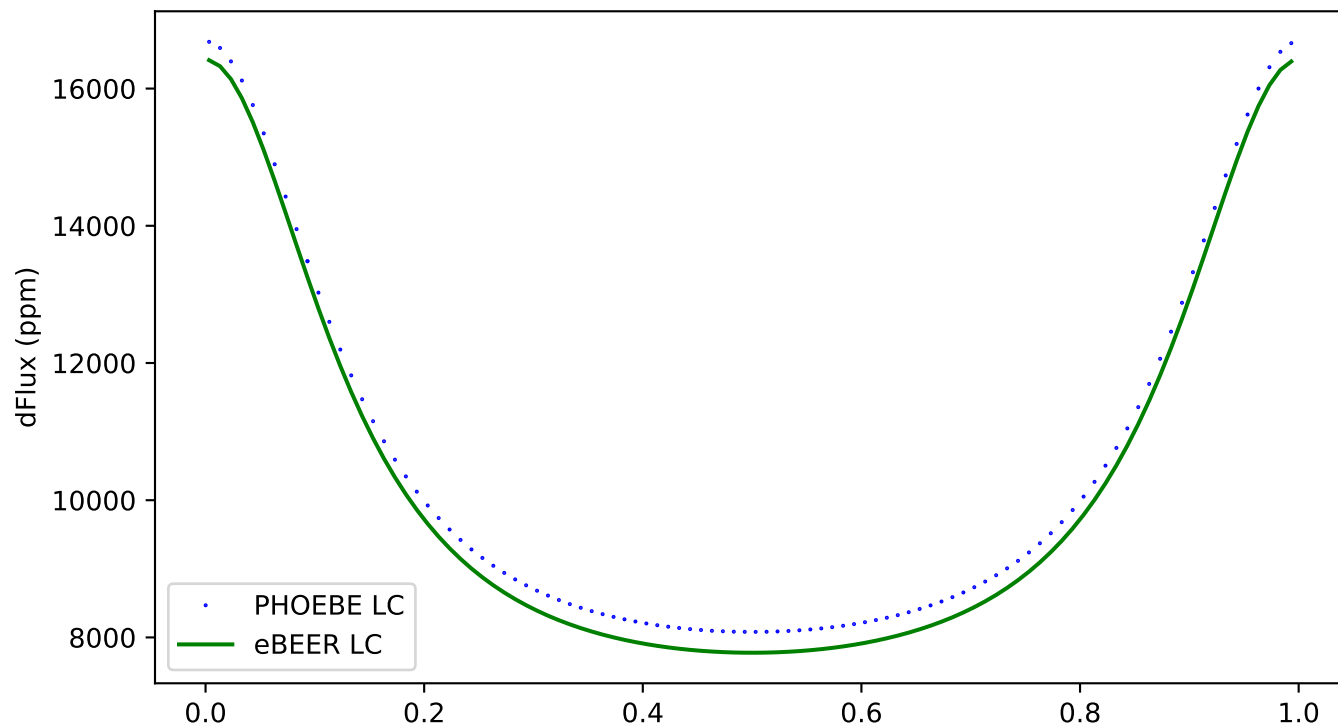
238 - ecc:0.3, incl:180, \omega :30, Porb:1, q:0.5
