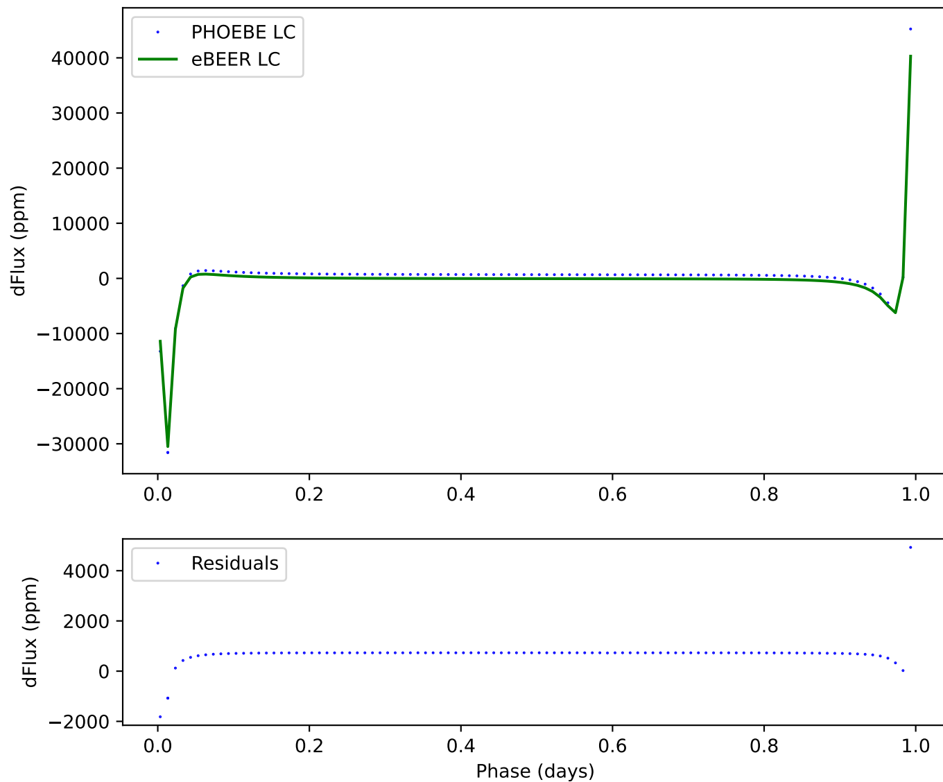
292 - ecc:0.8, incl:60, \omega :30, Porb:1, q:0.5
