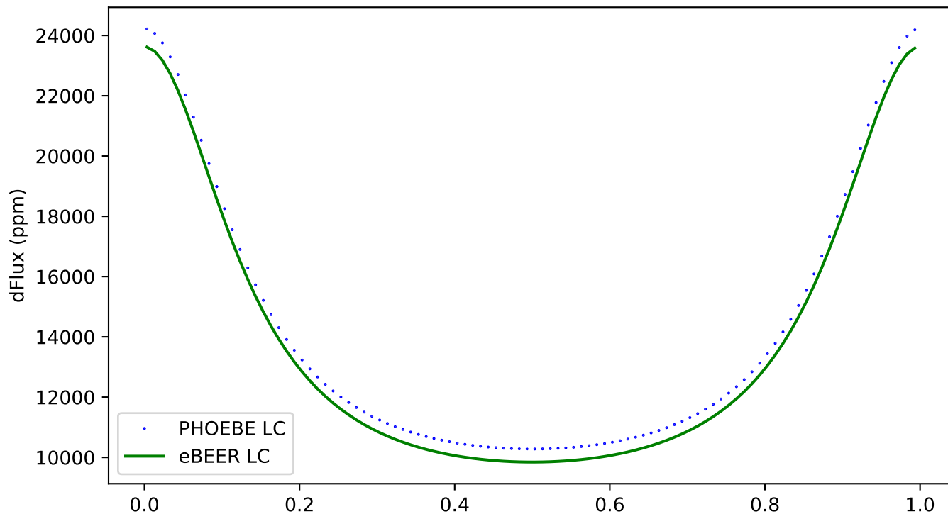
129 - ecc:0.3, incl:0, \omega :30, Porb:1, q:1
