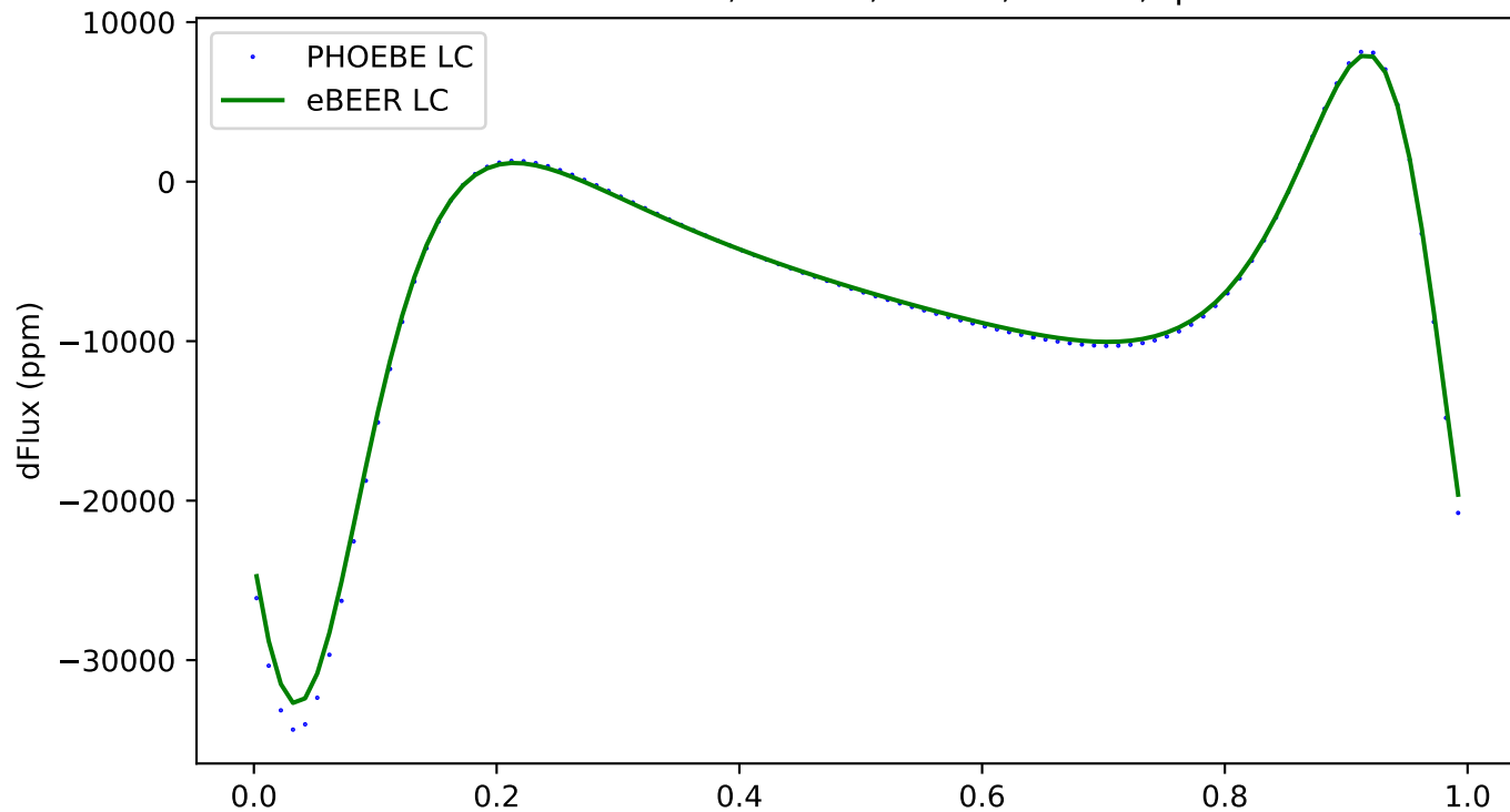
195 - ecc:0.3, incl:90, \omega :240, Porb:1, q:1
