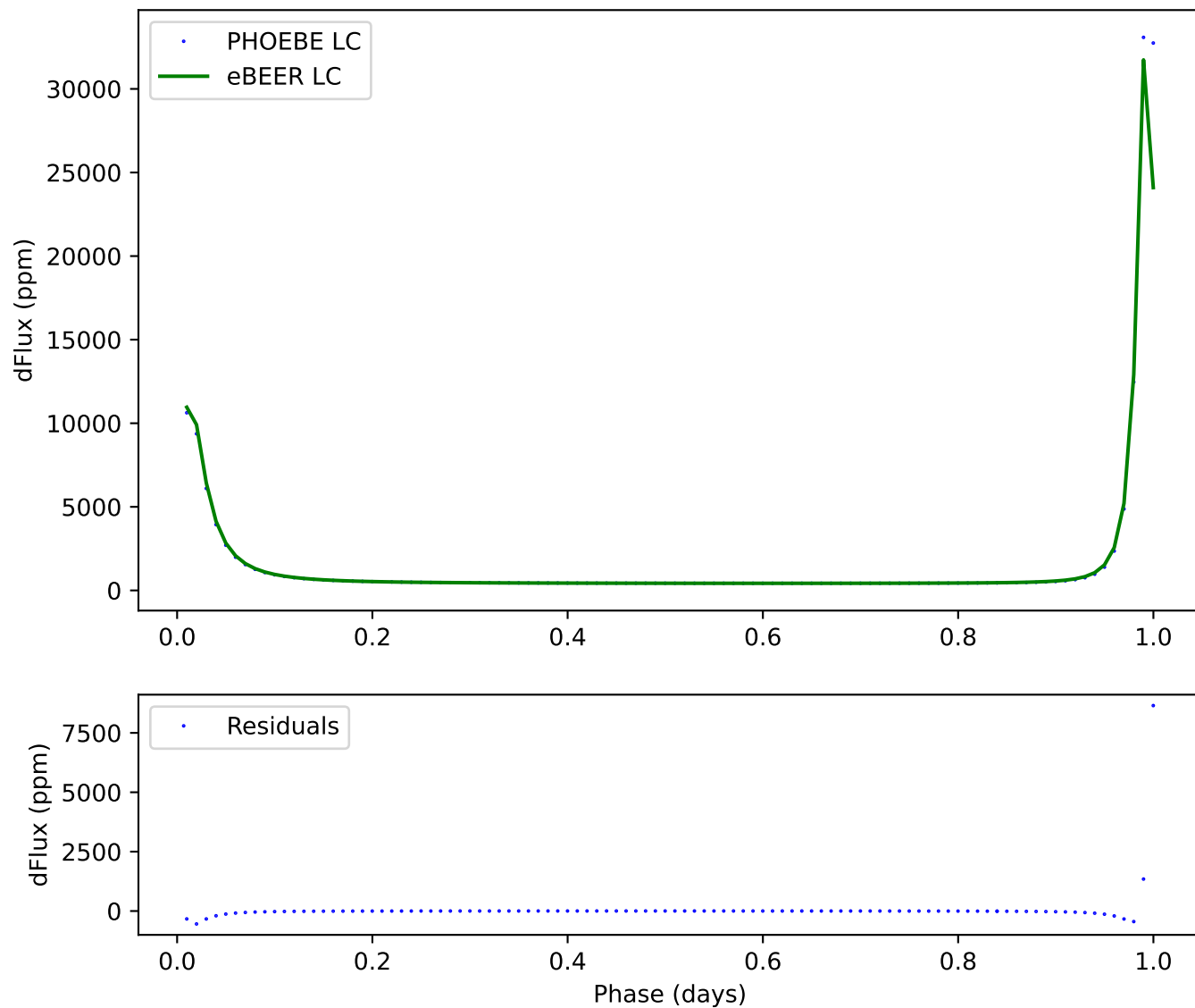
287 - ecc:0.8, incl:30, \omega :240, Porb:1, q:2
