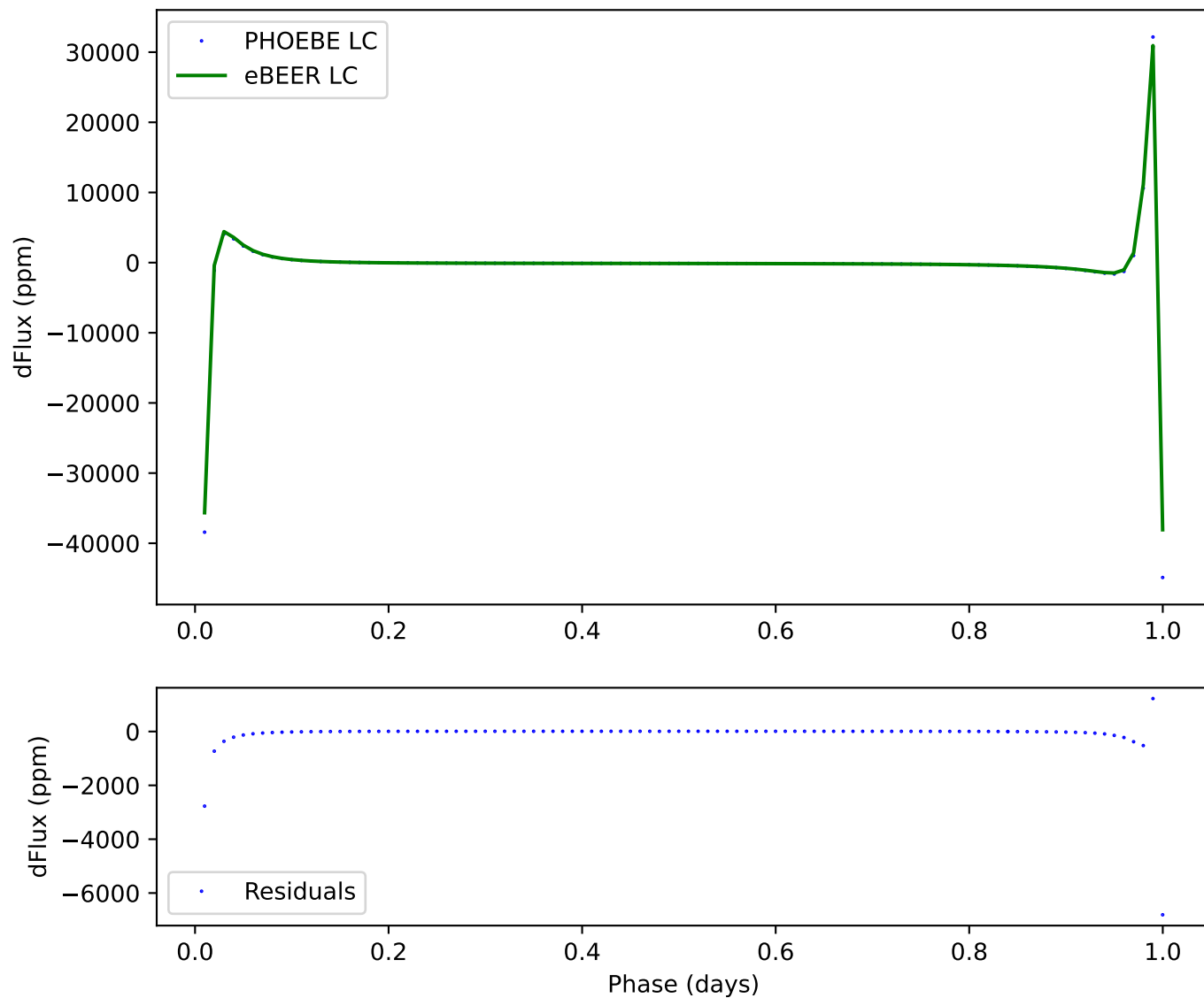
339 - ecc:0.8, incl:120, \omega :240, Porb:1, q:1
