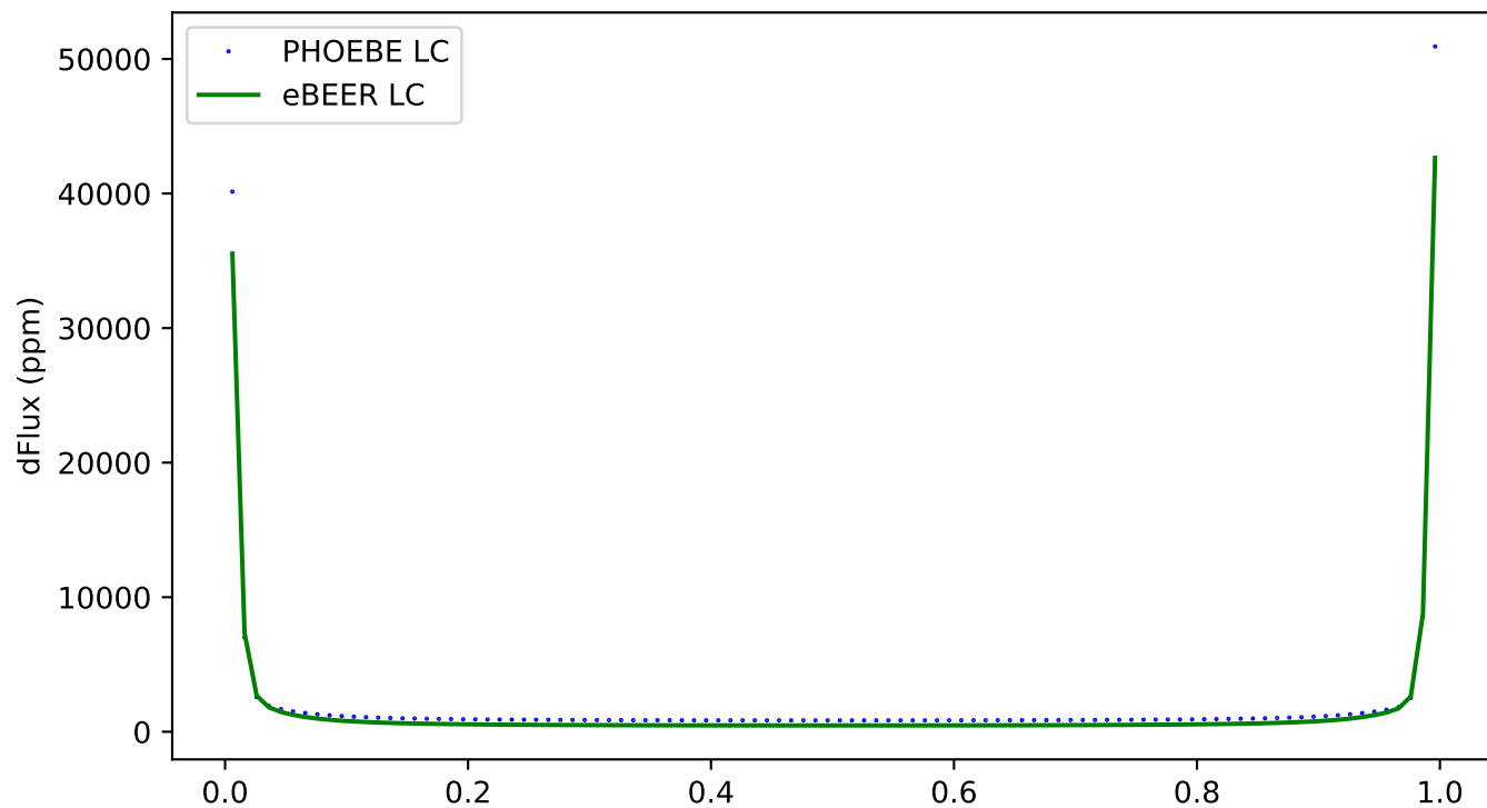
271 - ecc:0.8, incl:30, \omega :0, Porb:1, q:0.5
