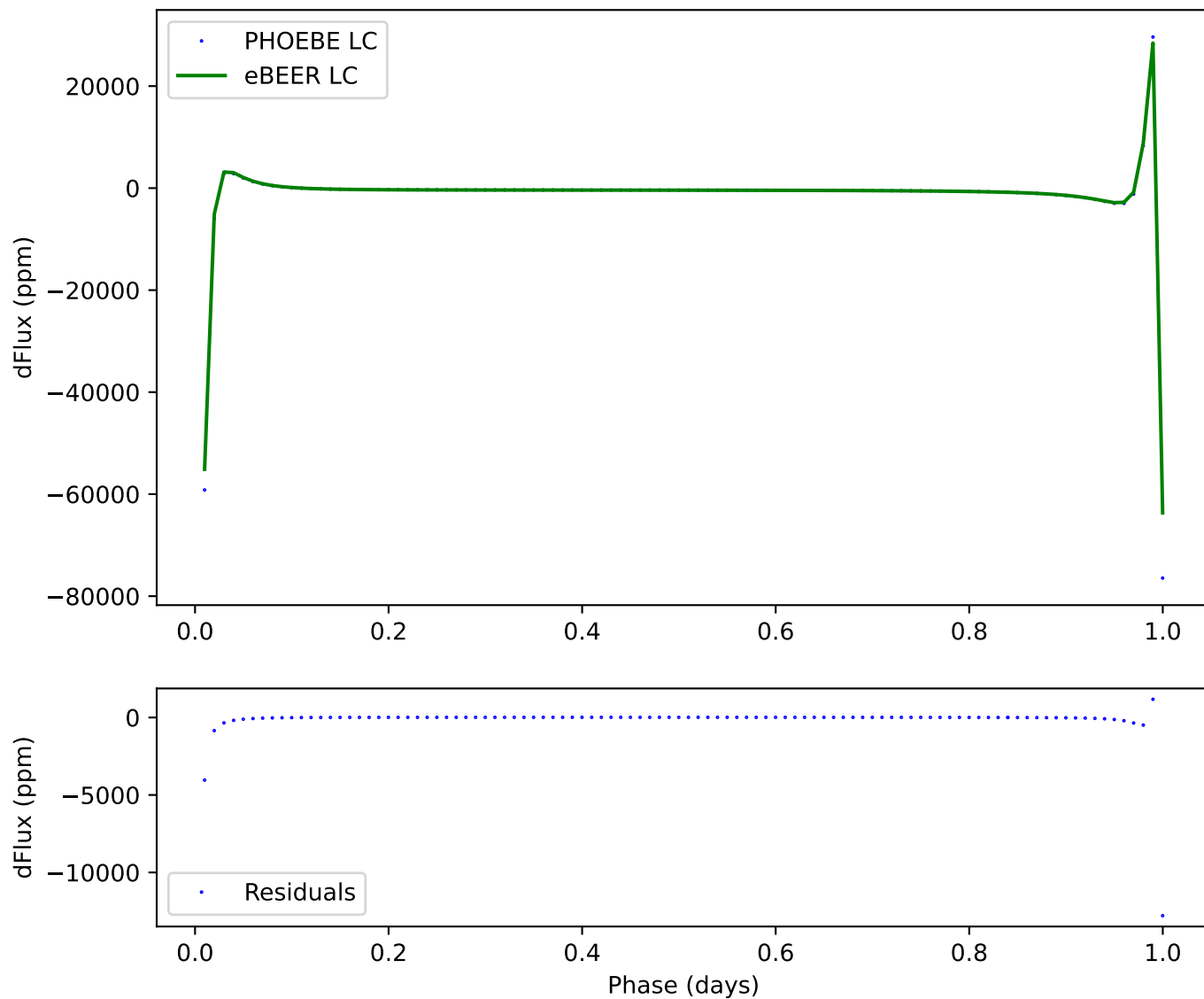
323 - ecc:0.8, incl:90, \omega :240, Porb:1, q:2
