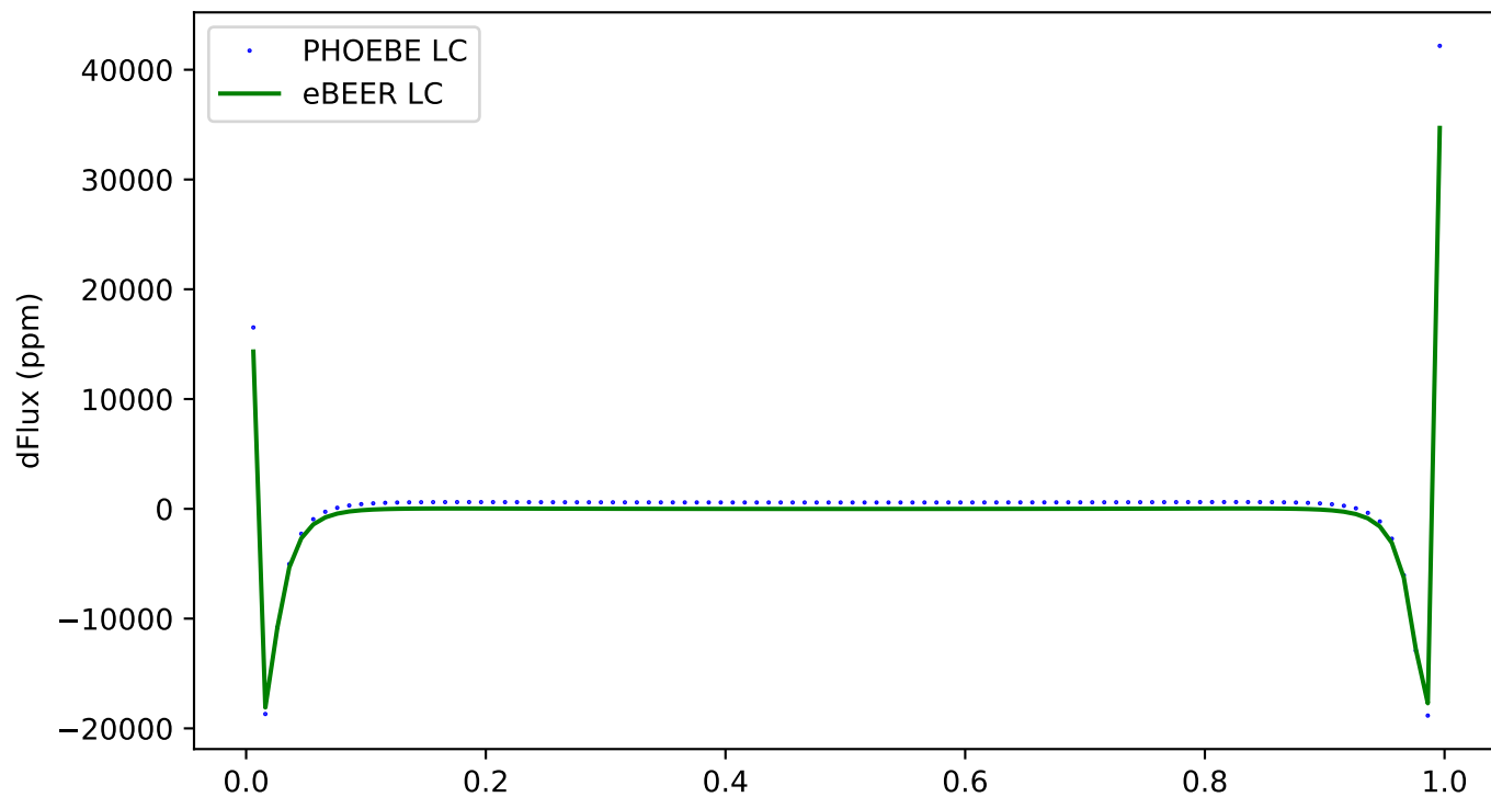
290 - ecc:0.8, incl:60, \omega :0, Porb:1, q:2
