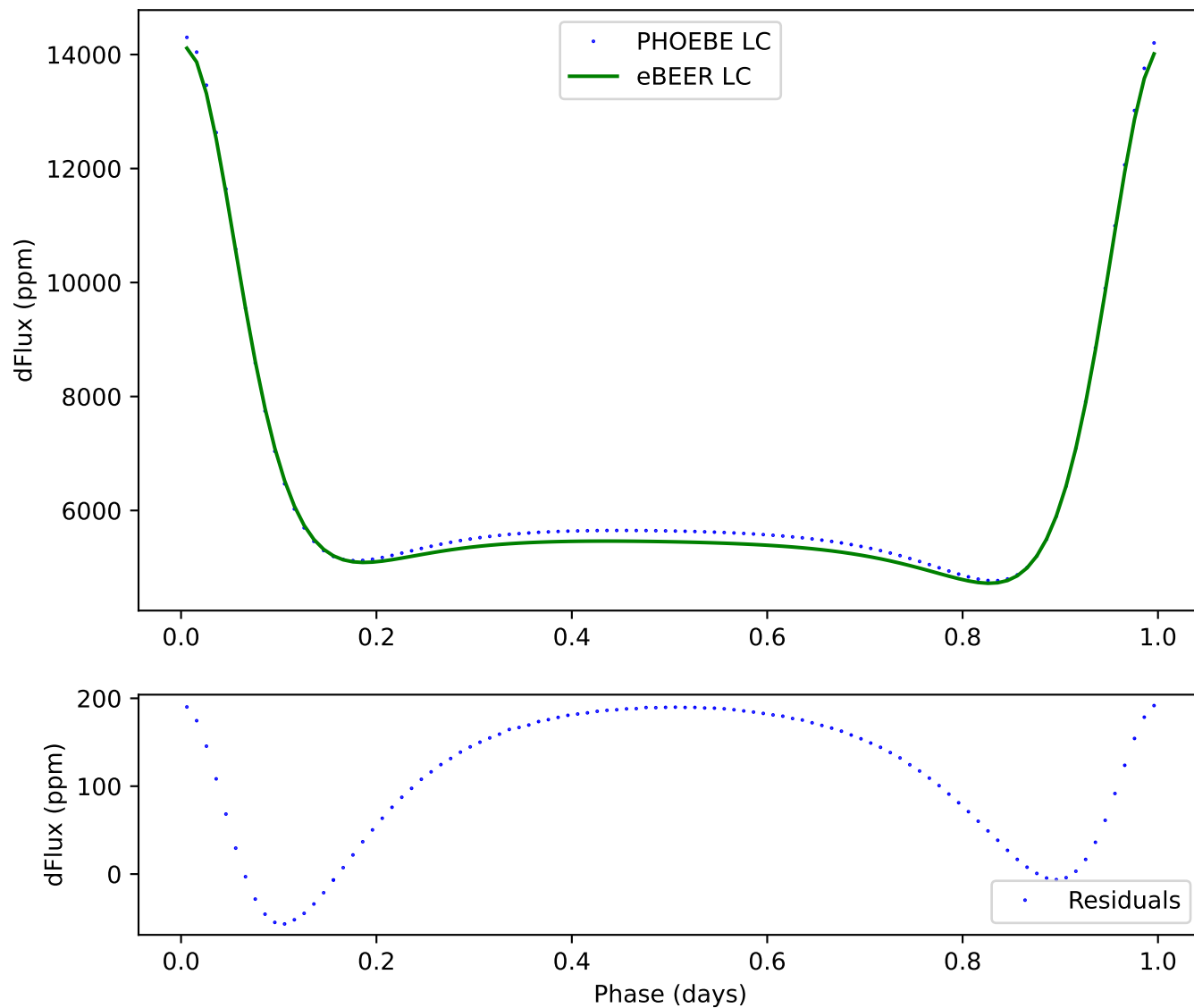
145 - ecc:0.3, incl:30, \omega :0, Porb:1, q:0.5
