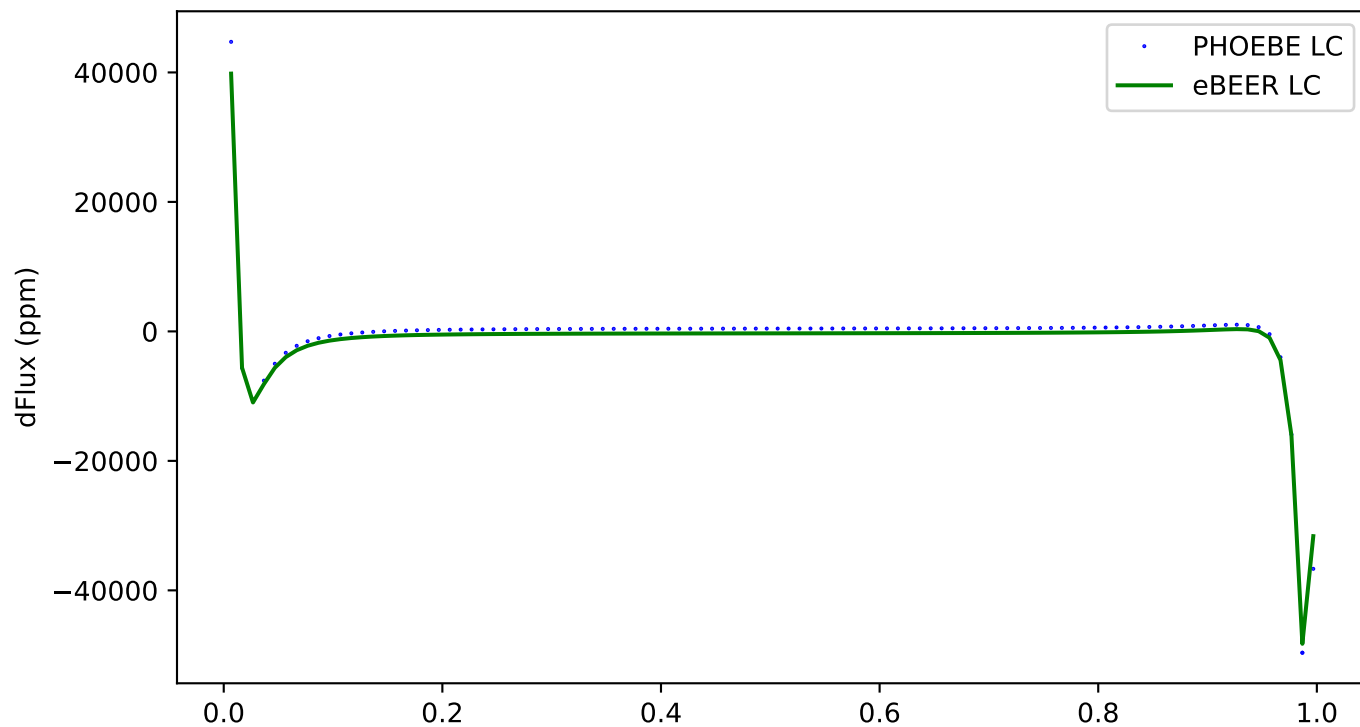
316 - ecc:0.8, incl:90, \omega :150, Porb:1, q:0.5
