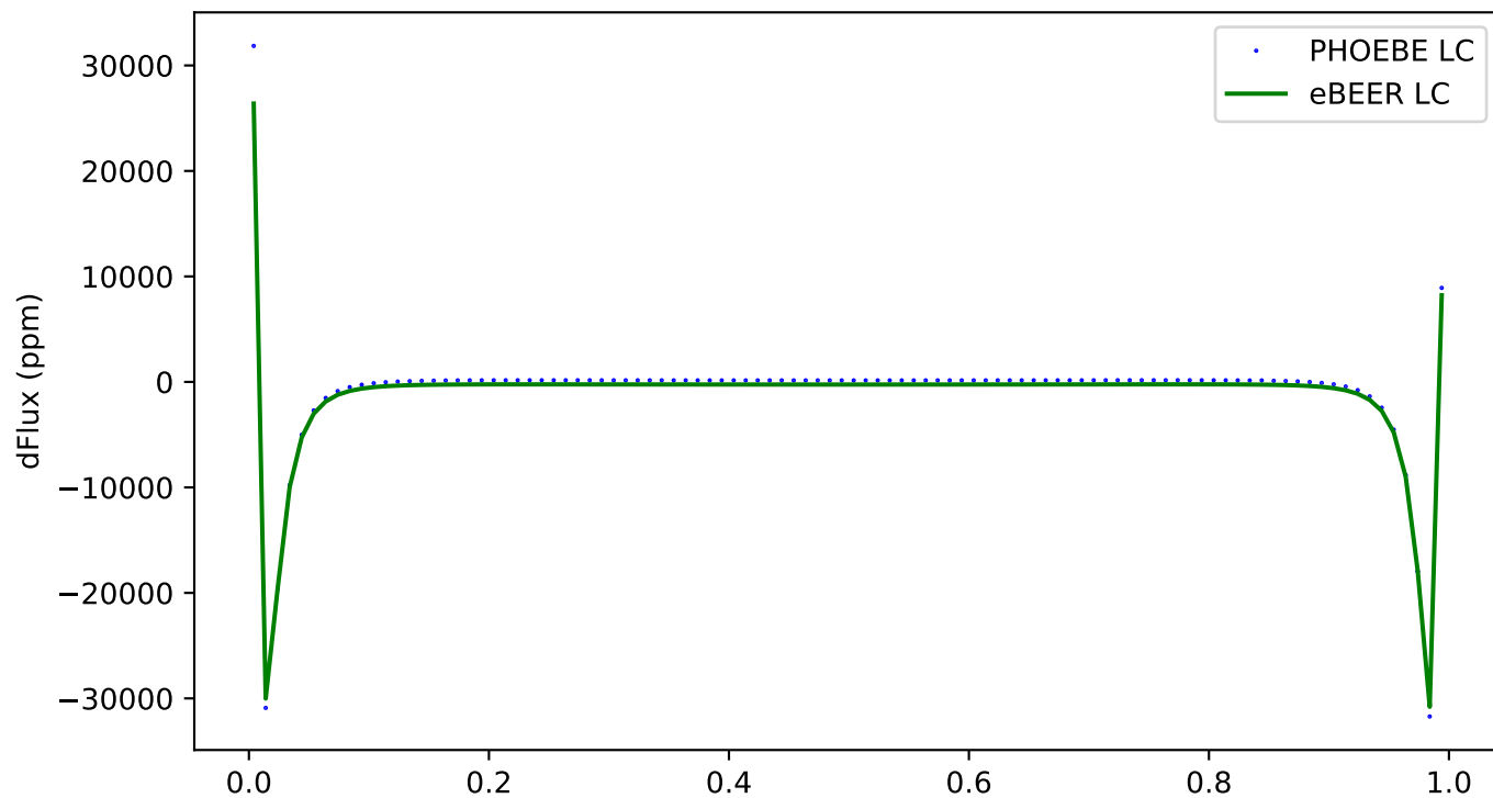
319 - ecc:0.8, incl:90, \omega :180, Porb:1, q:0.5
