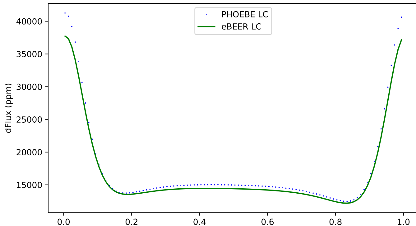
158 - ecc:0.3, incl:30, \omega :180, Porb:1, q:2
