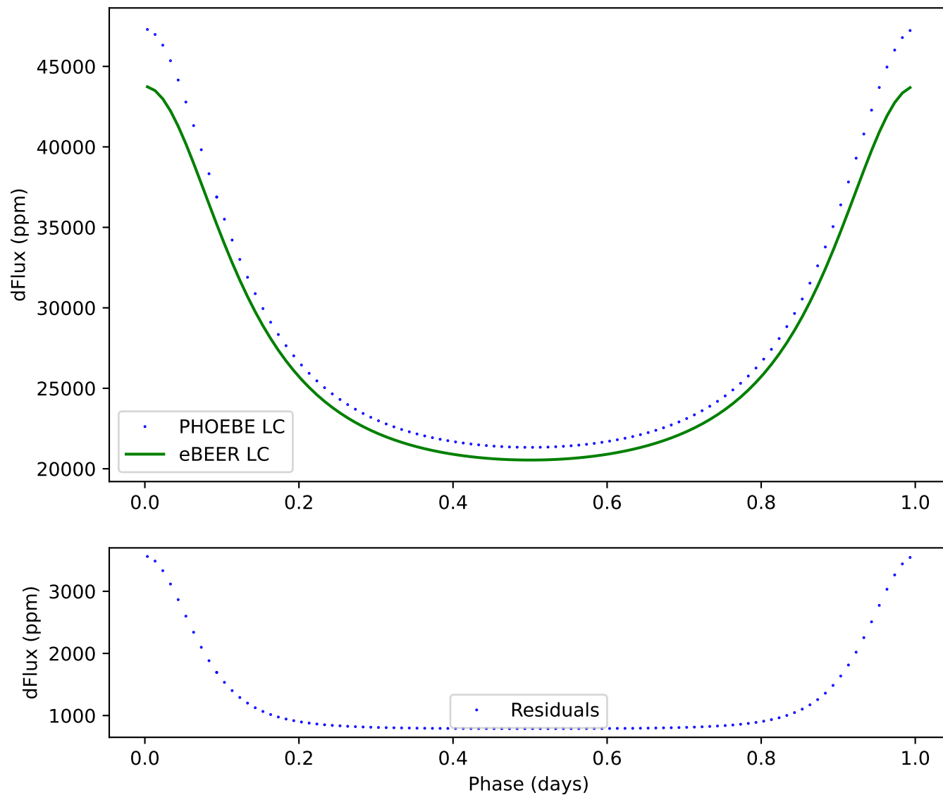
239 - ecc:0.3, incl:180, \omega :30, Porb:1, q:2
