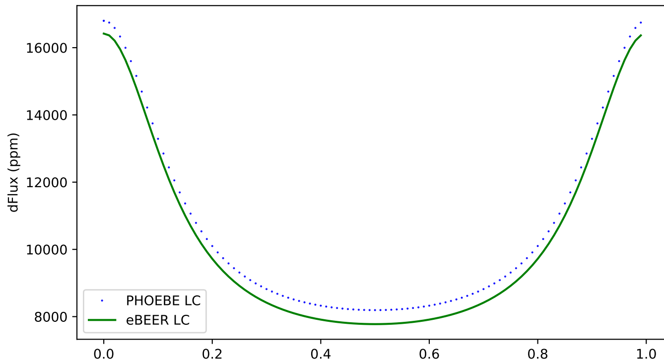
133 - ecc:0.3, incl:0, \omega :90, Porb:1, q:0.5
