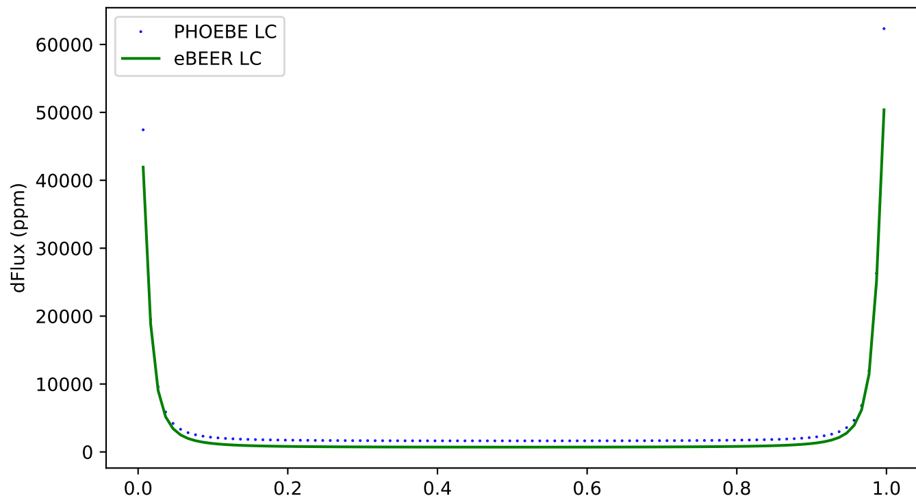
371 - ecc:0.8, incl:180, \omega :150, Porb:1, q:2
