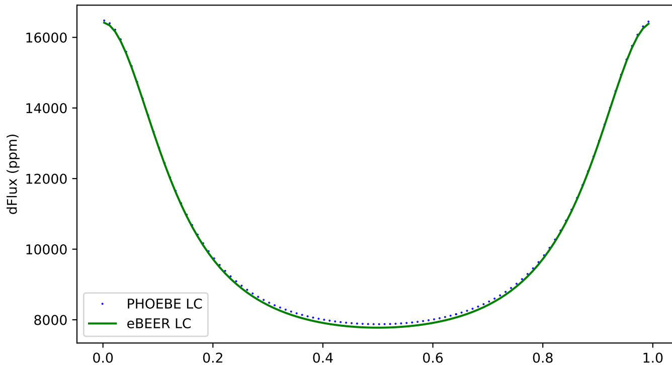
142 - ecc:0.3, incl:0, \omega :240, Porb:1, q:0.5
