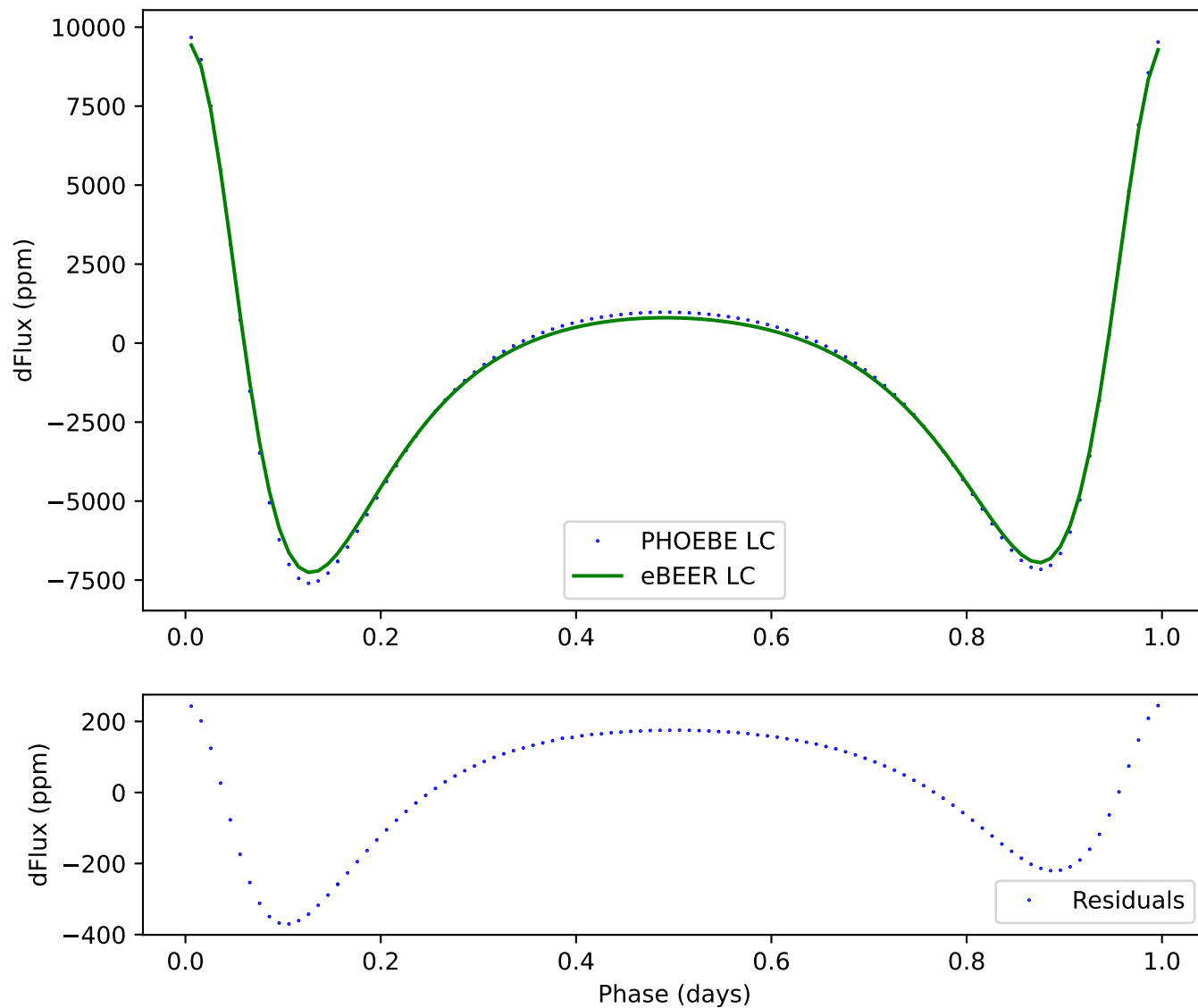
199 - ecc:0.3, incl:120, \omega :0, Porb:1, q:0.5
