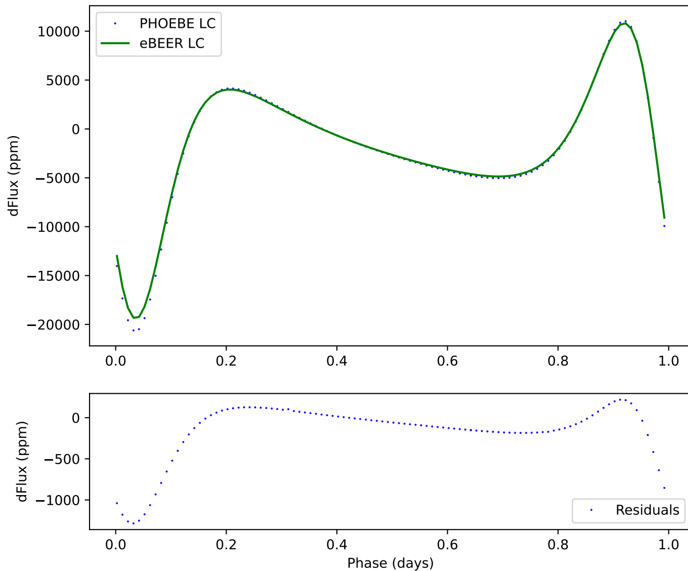
177 - ecc:0.3, incl:60, \omega :240, Porb:1, q:1
