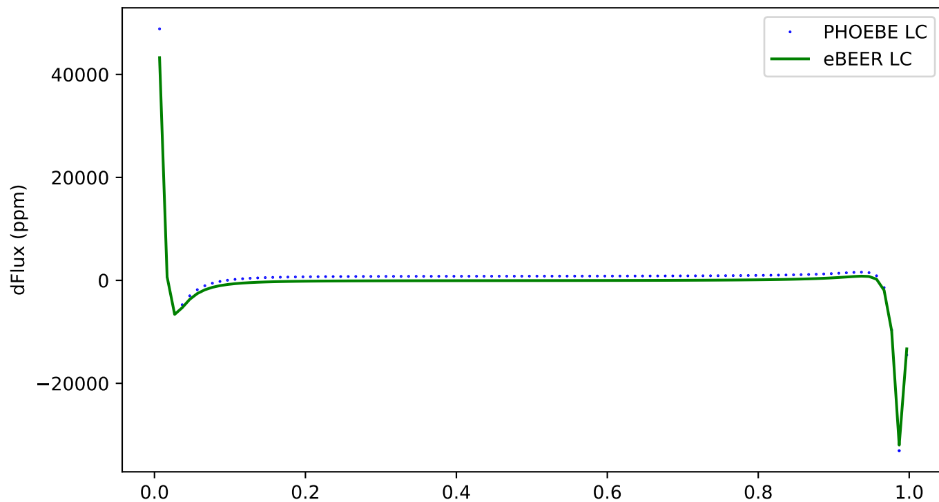
297 - ecc:0.8, incl:60, \omega :150, Porb:1, q:1
