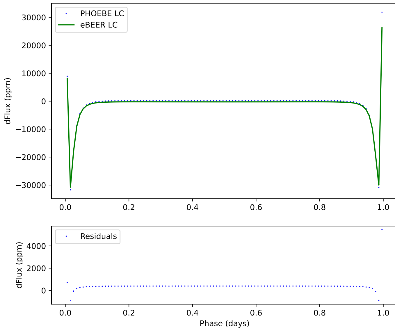
307 - ecc:0.8, incl:90, \omega :0, Porb:1, q:0.5
