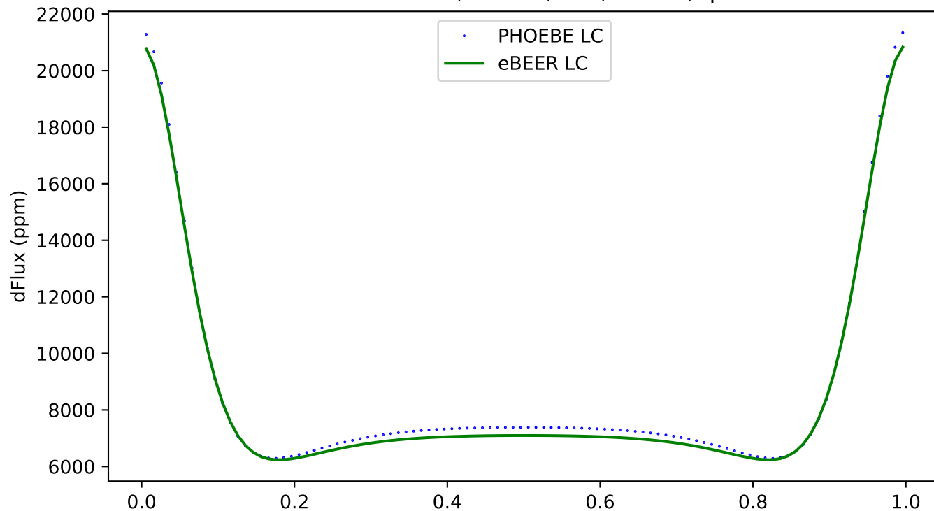
144 - ecc:0.3, incl:30, \omega :0, Porb:1, q:1
