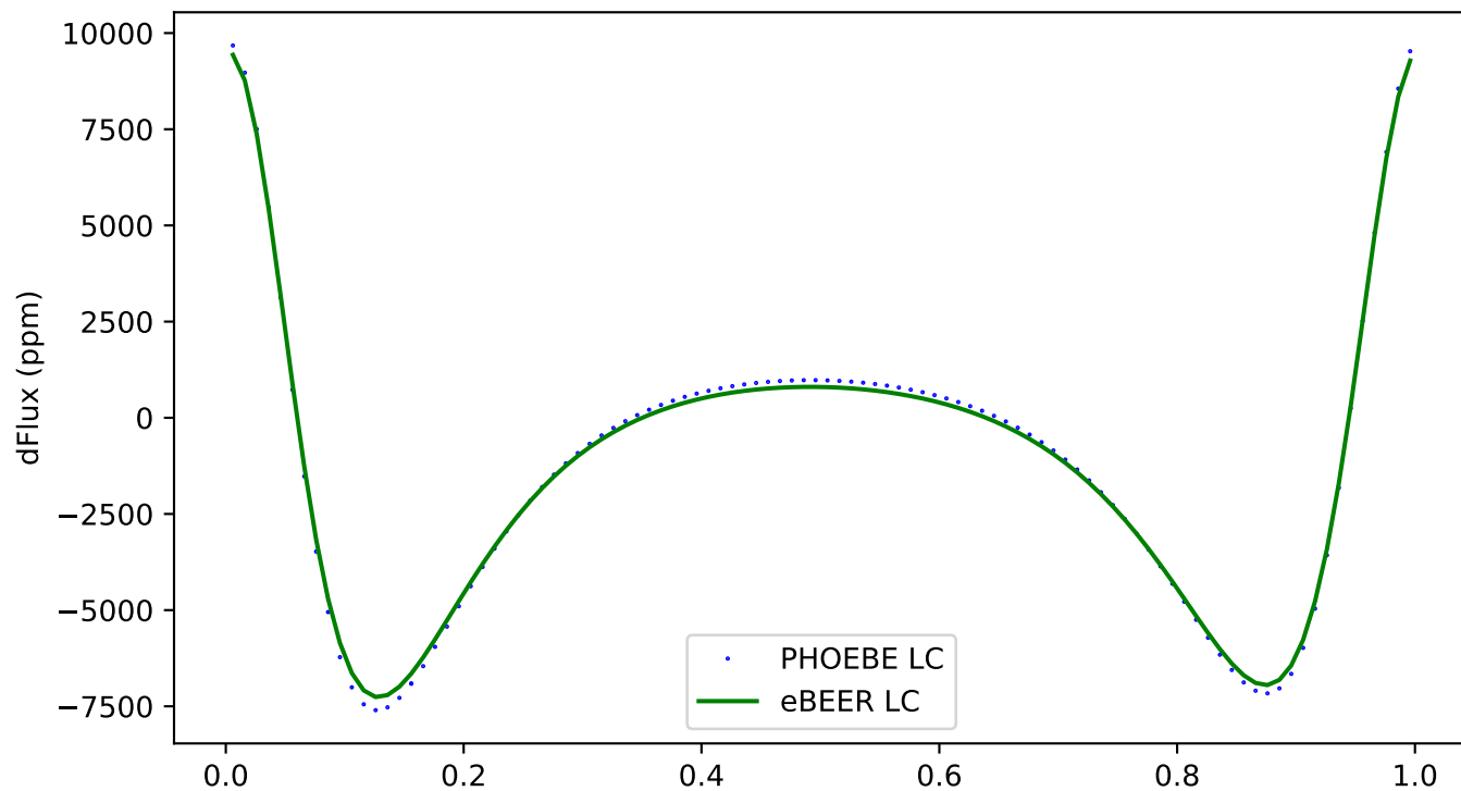
163 - ecc:0.3, incl:60, \omega :0, Porb:1, q:0.5
