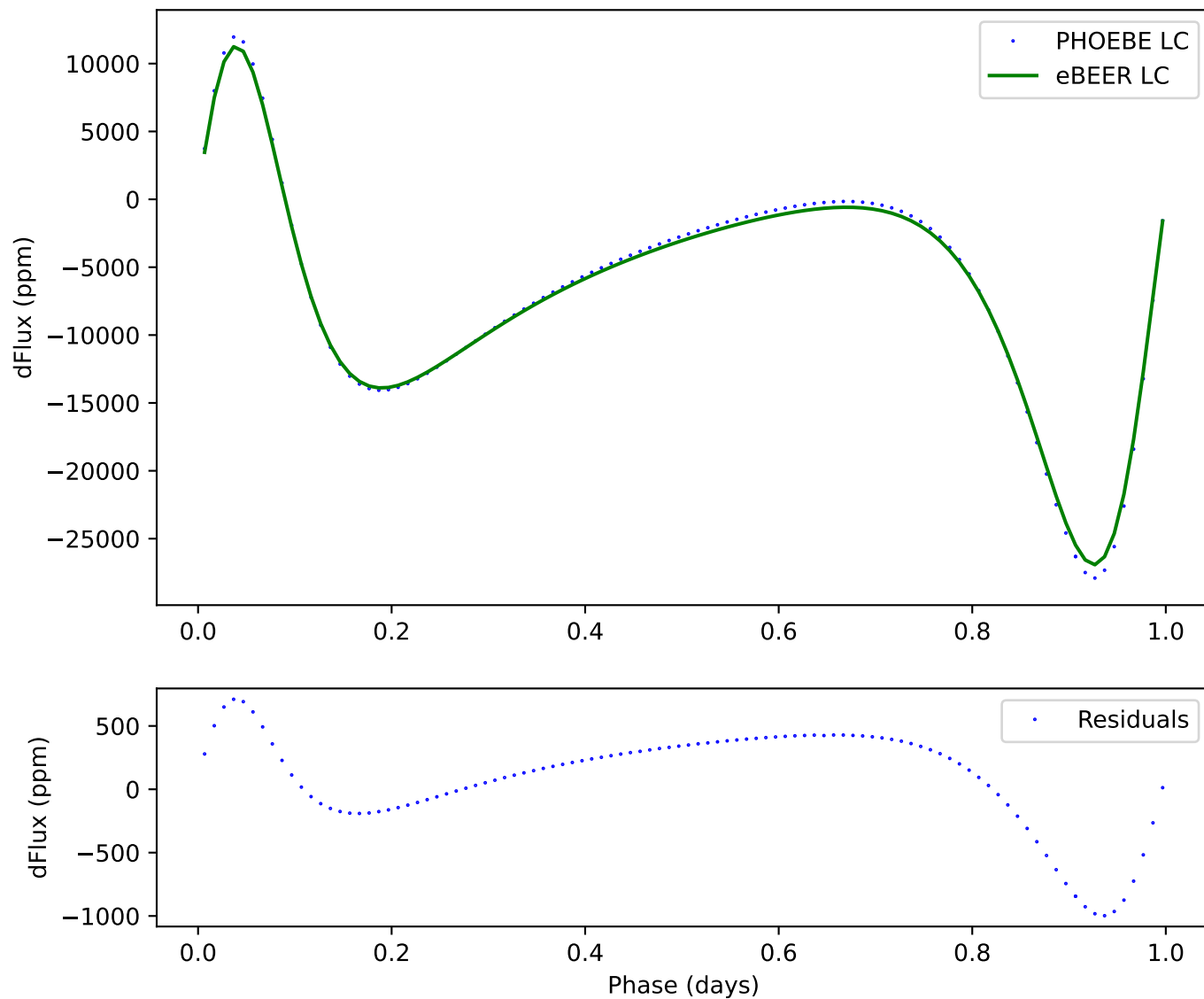
189 - ecc:0.3, incl:90, \omega :150, Porb:1, q:1
