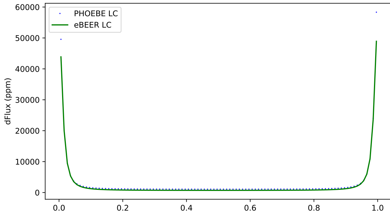
253 - ecc:0.8, incl:0, \omega :0, Porb:1, q:0.5
