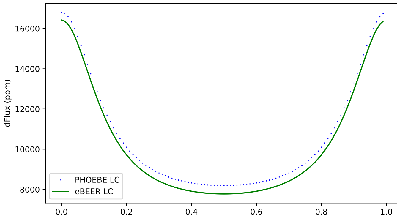
241 - ecc:0.3, incl:180, \omega :90, Porb:1, q:0.5
