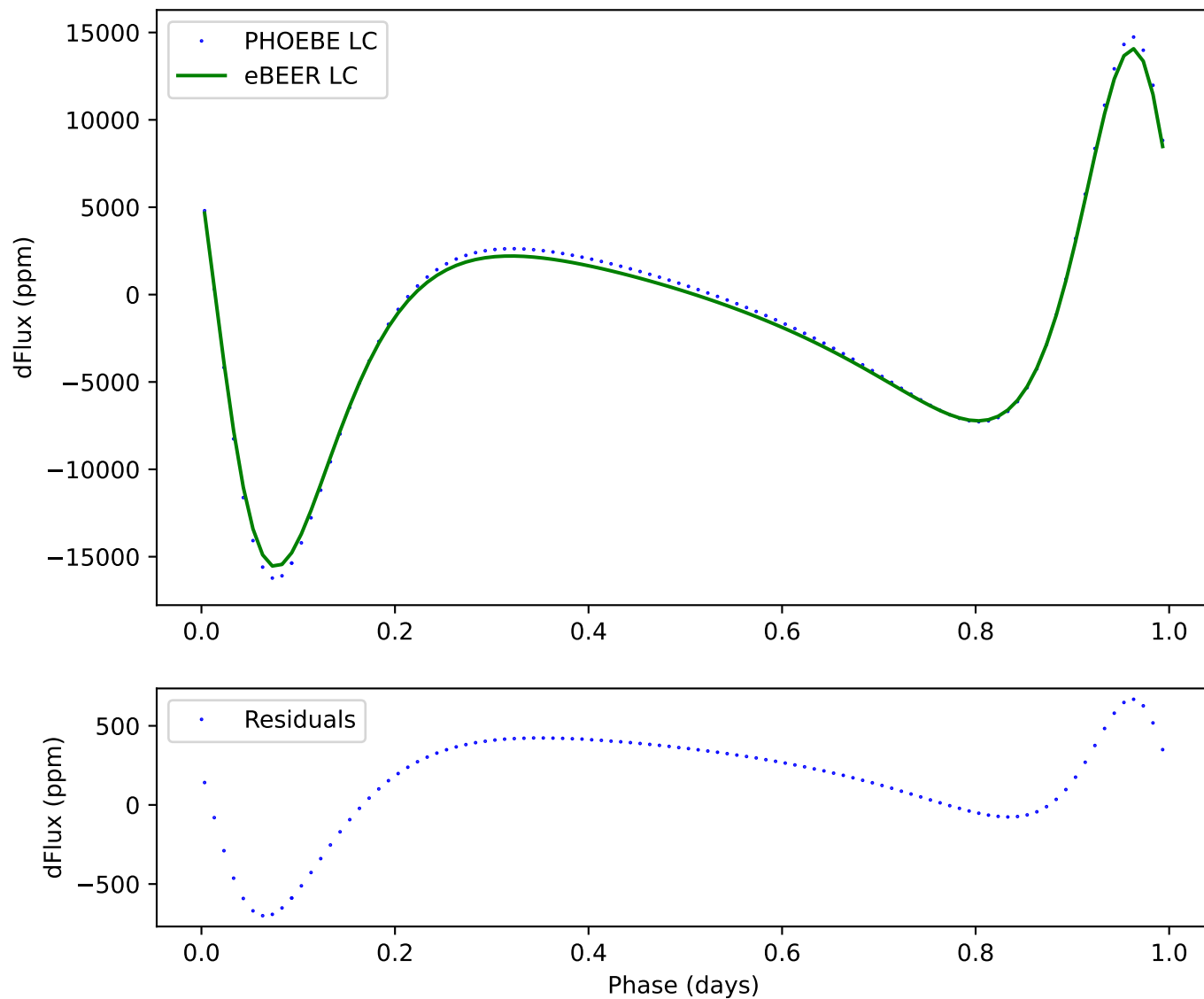
201 - ecc:0.3, incl:120, \omega :30, Porb:1, q:1
