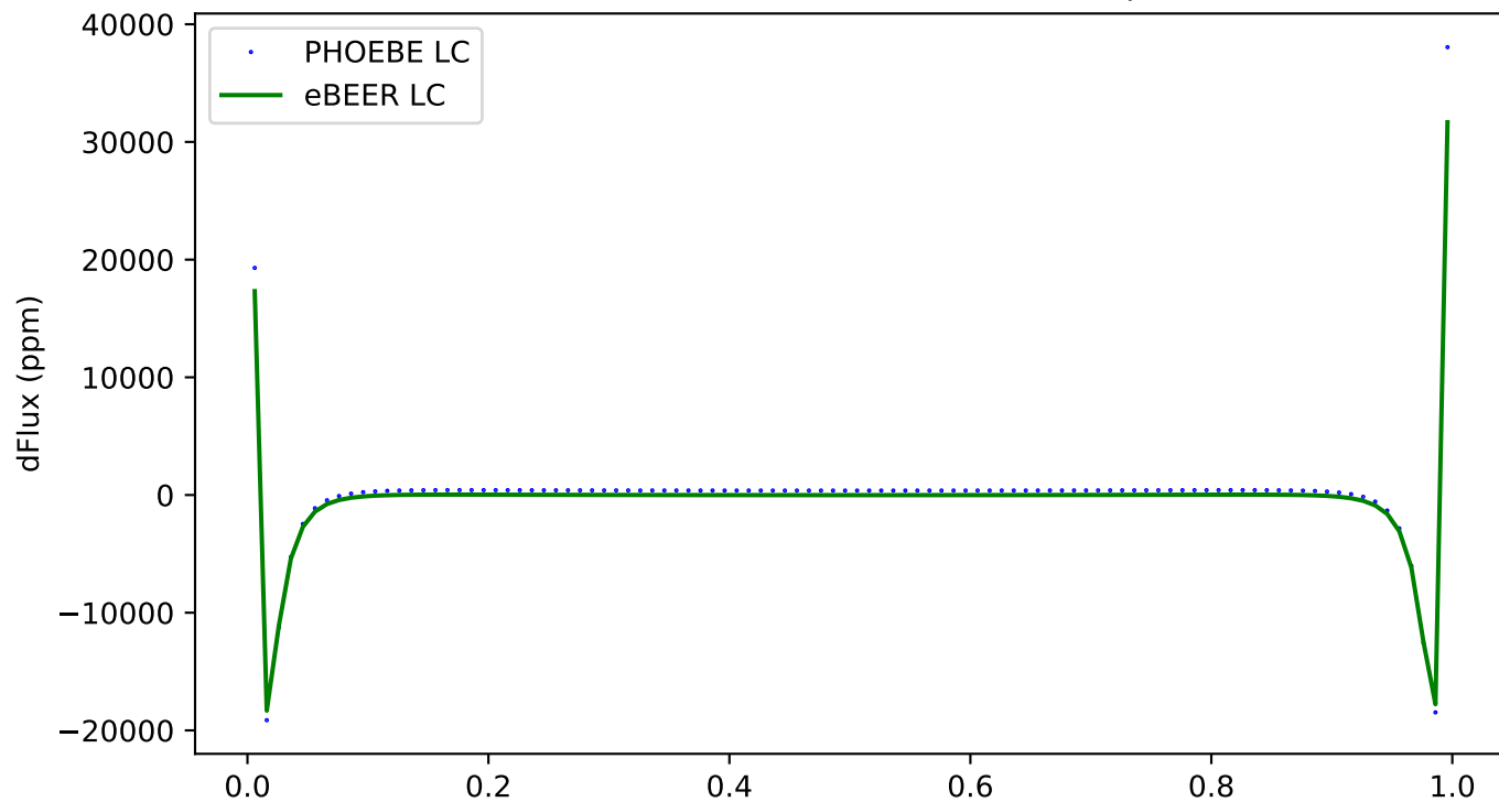
289 - ecc:0.8, incl:60, \omega :0, Porb:1, q:0.5
