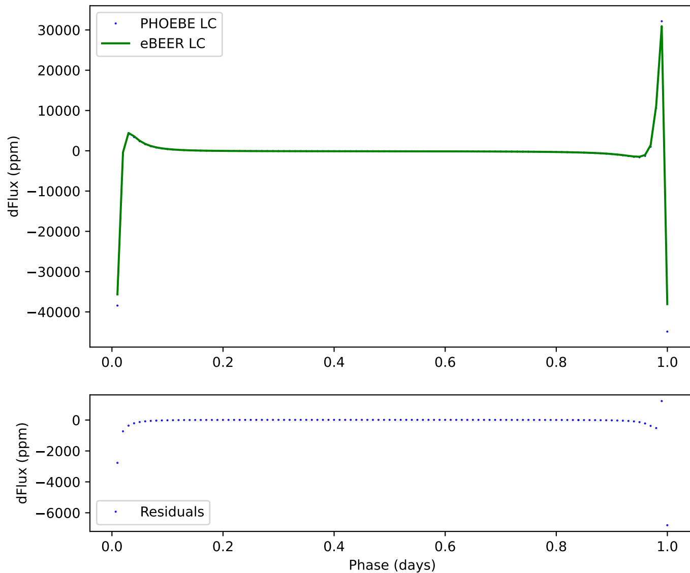
303 - ecc:0.8, incl:60, \omega :240, Porb:1, q:1
