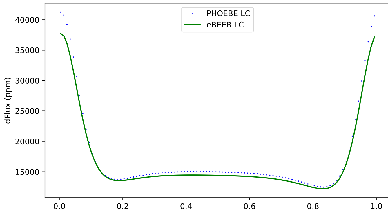
230 - ecc:0.3, incl:150, \omega :180, Porb:1, q:2
