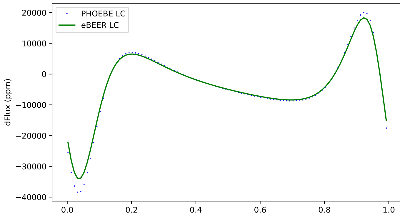
215 - ecc:0.3, incl:120, \omega :240, Porb:1, q:2
