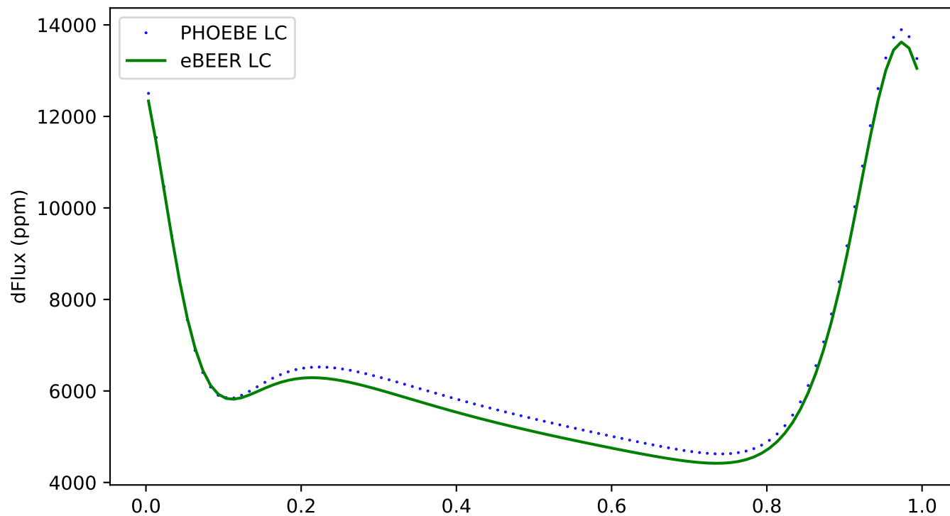
148 - ecc:0.3, incl:30, \omega :30, Porb:1, q:0.5
