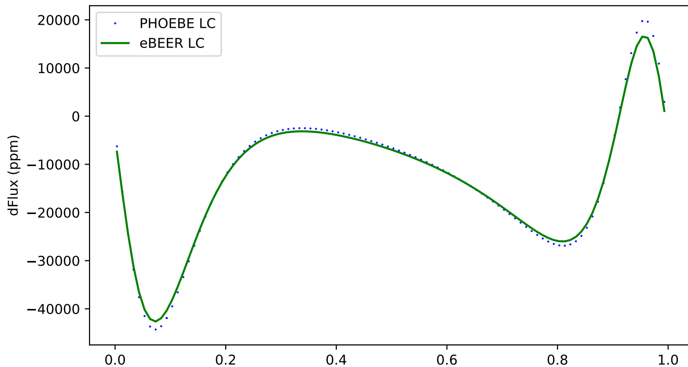
185 - ecc:0.3, incl:90, \omega :30, Porb:1, q:2
