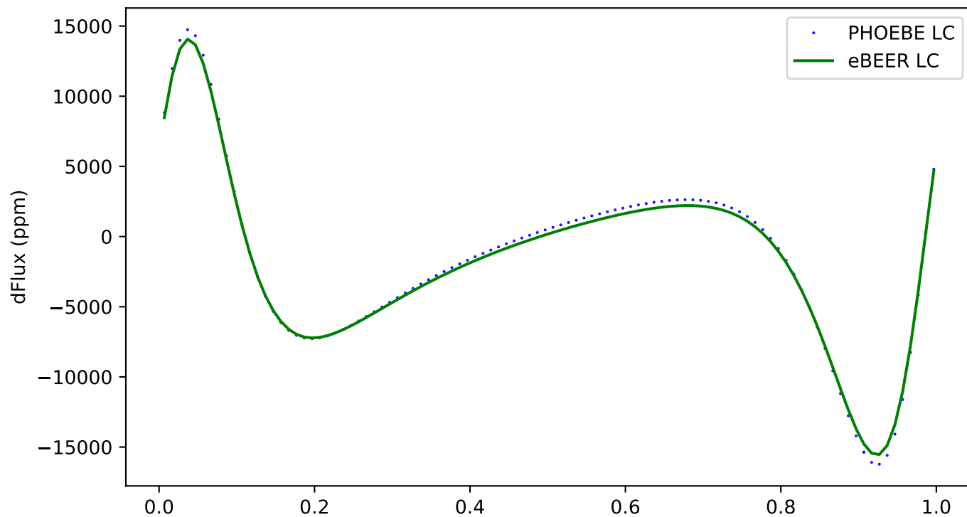
171 - ecc:0.3, incl:60, \omega :150, Porb:1, q:1
