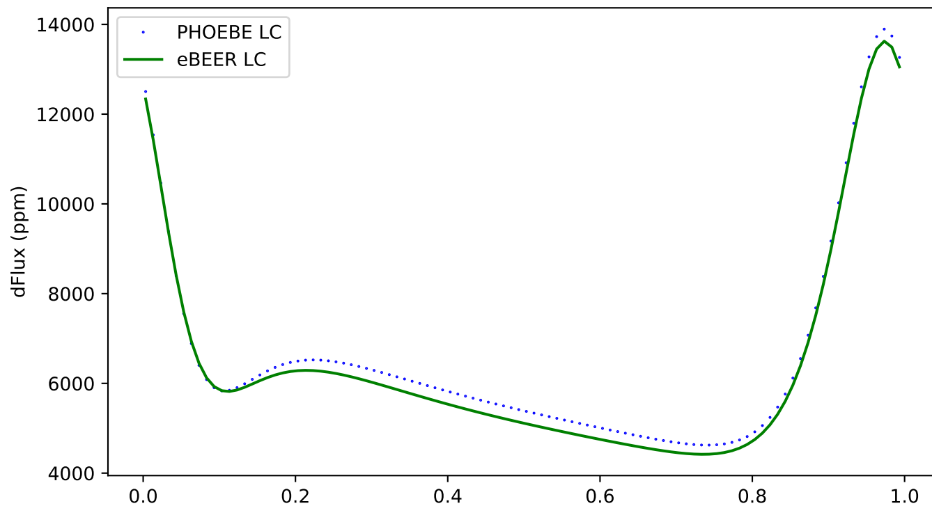
220 - ecc:0.3, incl:150, \omega :30, Porb:1, q:0.5
