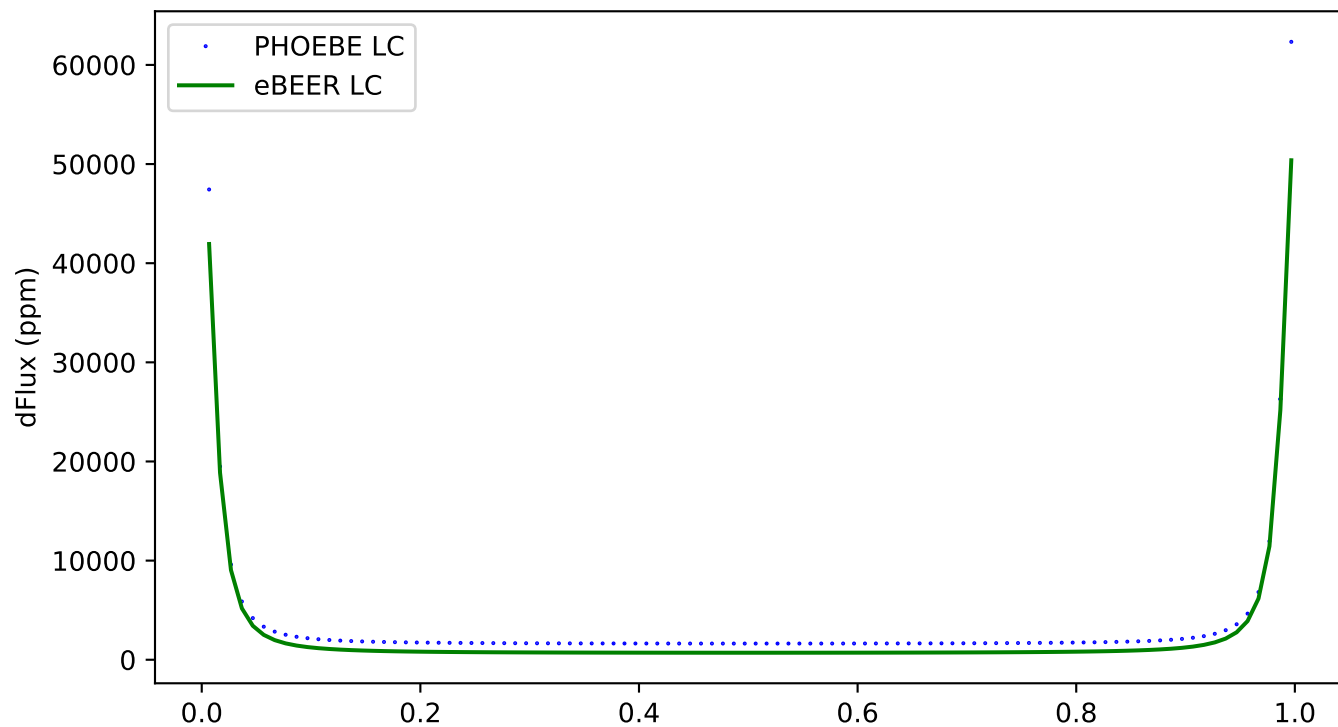
263 - ecc:0.8, incl:0, \omega :150, Porb:1, q:2
