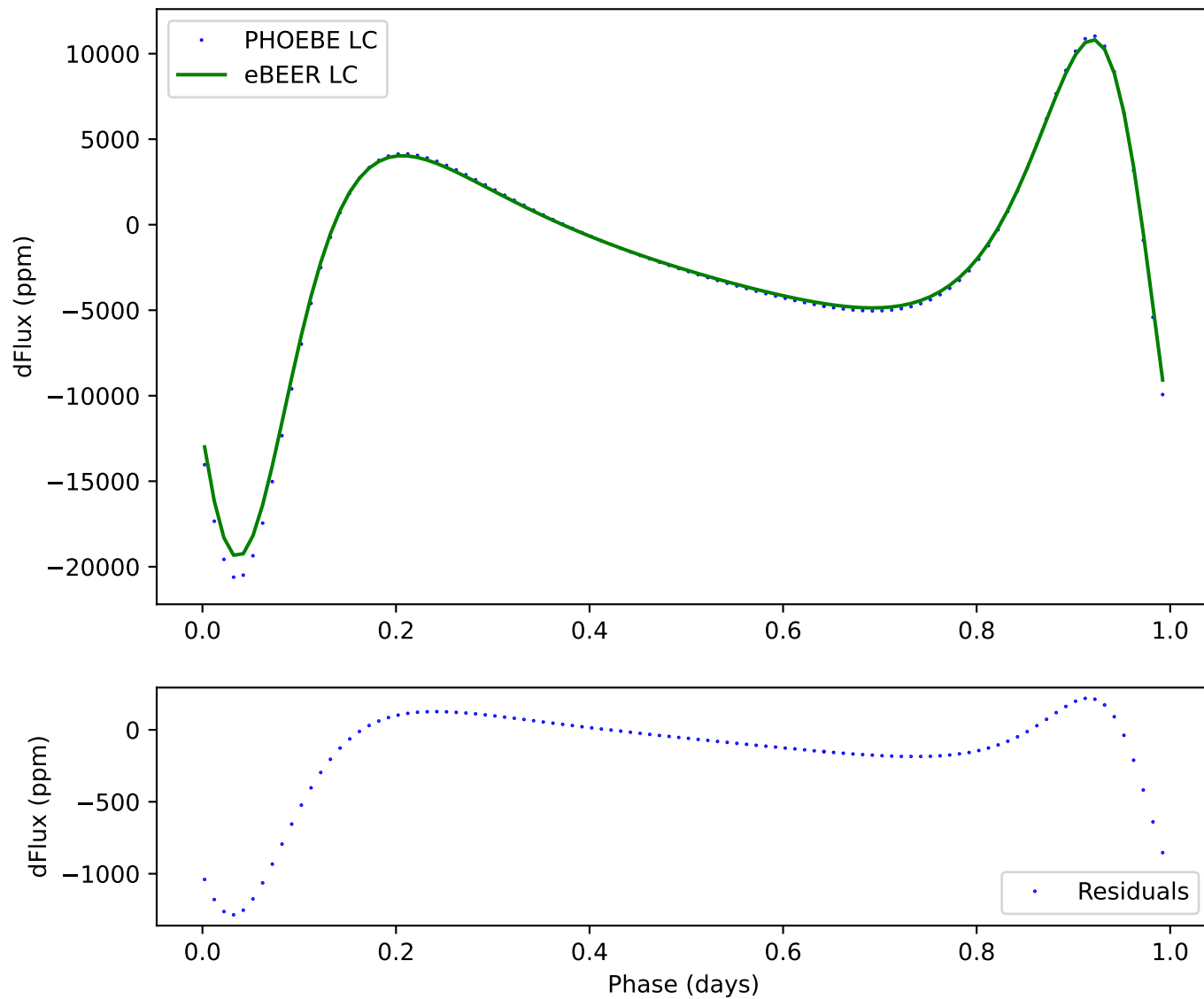
213 - ecc:0.3, incl:120, \omega :240, Porb:1, q:1
