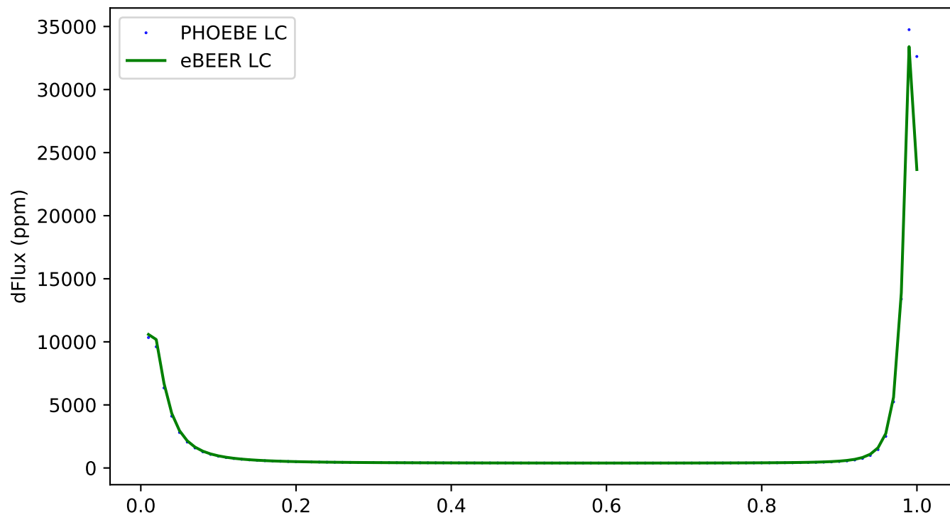
357 - ecc:0.8, incl:150, \omega :240, Porb:1, q:1
