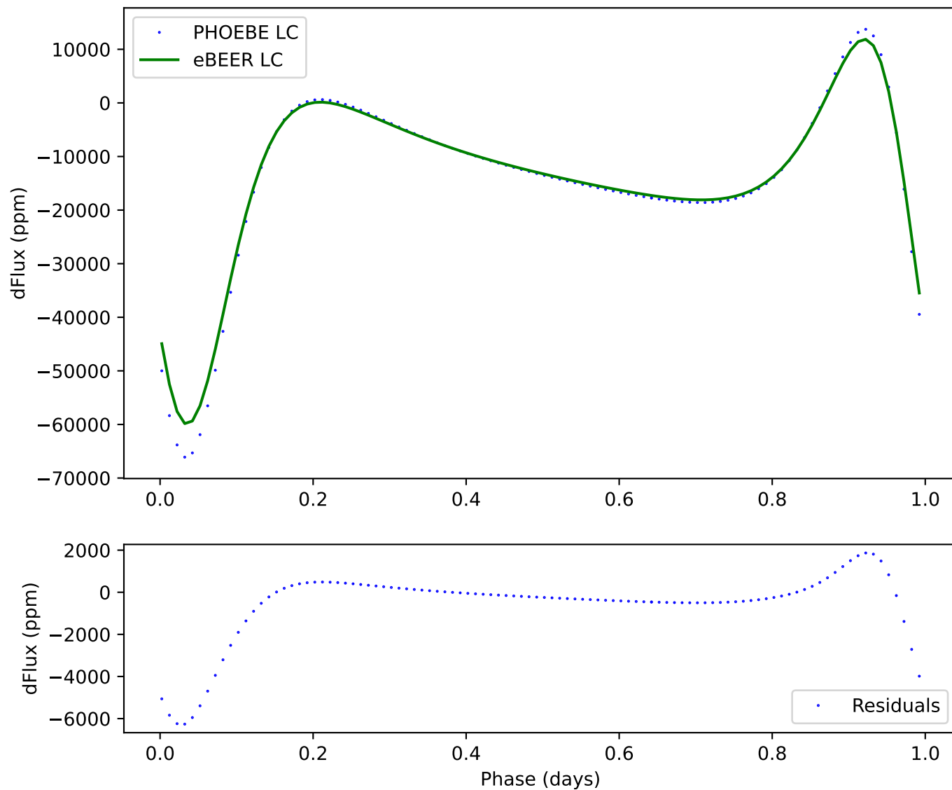
197 - ecc:0.3, incl:90, \omega :240, Porb:1, q:2
