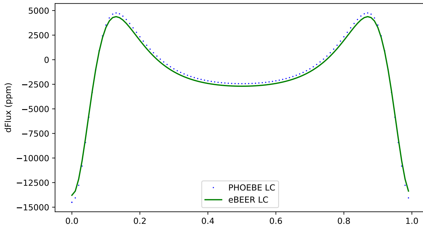
205 - ecc:0.3, incl:120, \omega :90, Porb:1, q:0.5
