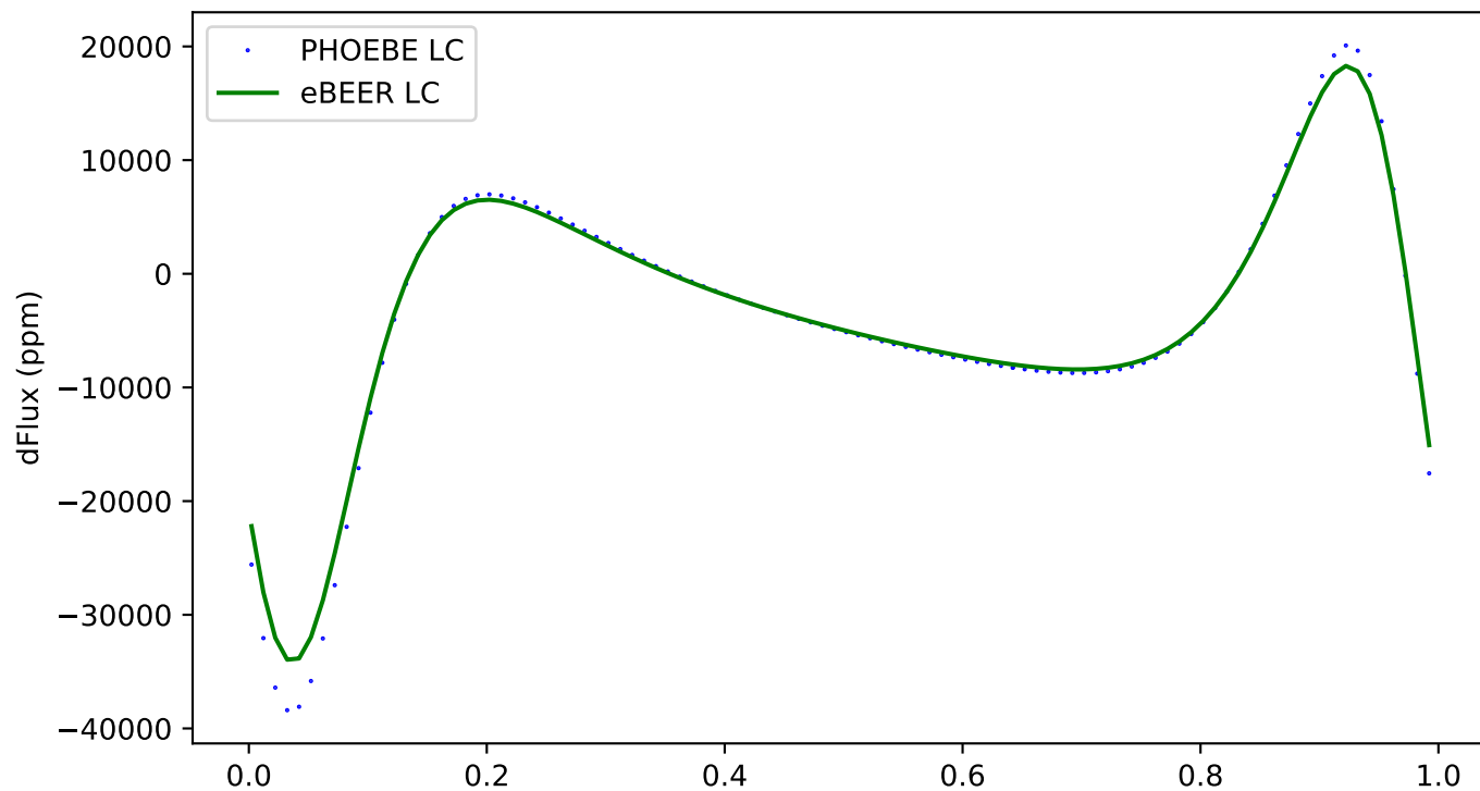
179 - ecc:0.3, incl:60, \omega :240, Porb:1, q:2
