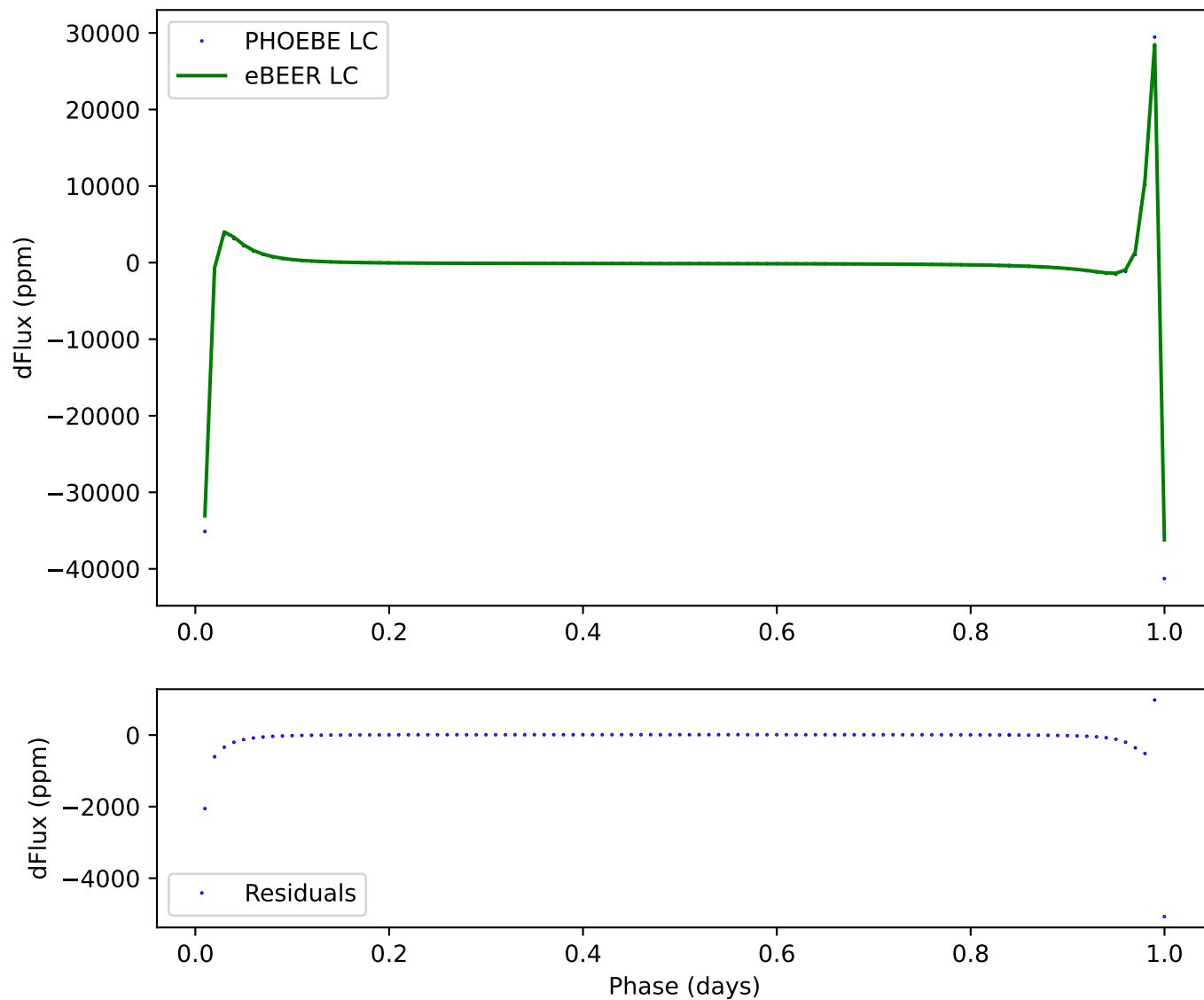
304 - ecc:0.8, incl:60, \omega :240, Porb:1, q:0.5
