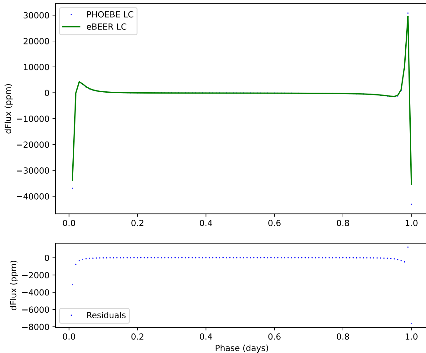
305 - ecc:0.8, incl:60, \omega :240, Porb:1, q:2
