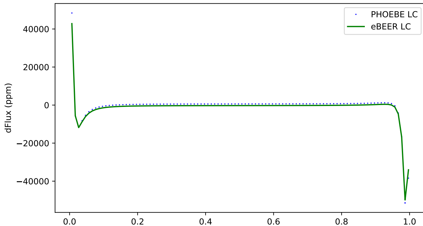
315 - ecc:0.8, incl:90, \omega :150, Porb:1, q:1
