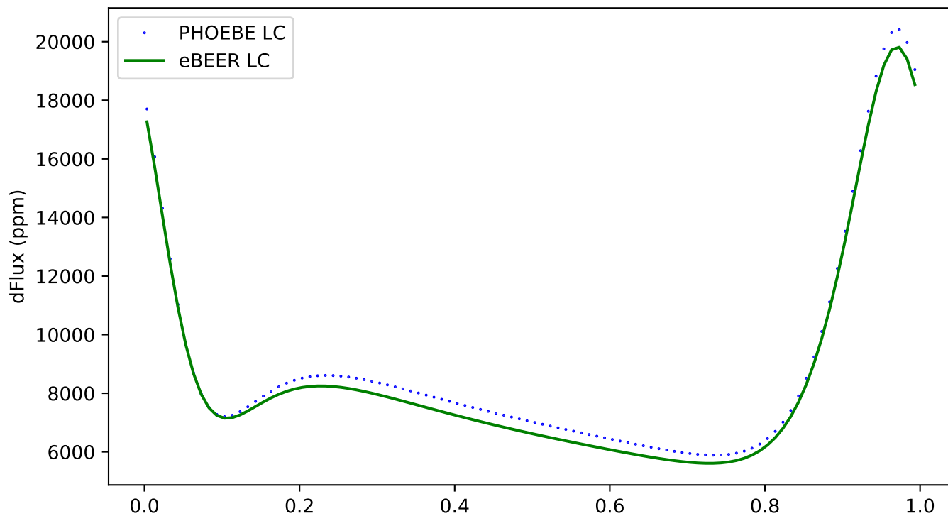
219 - ecc:0.3, incl:150, \omega :30, Porb:1, q:1
