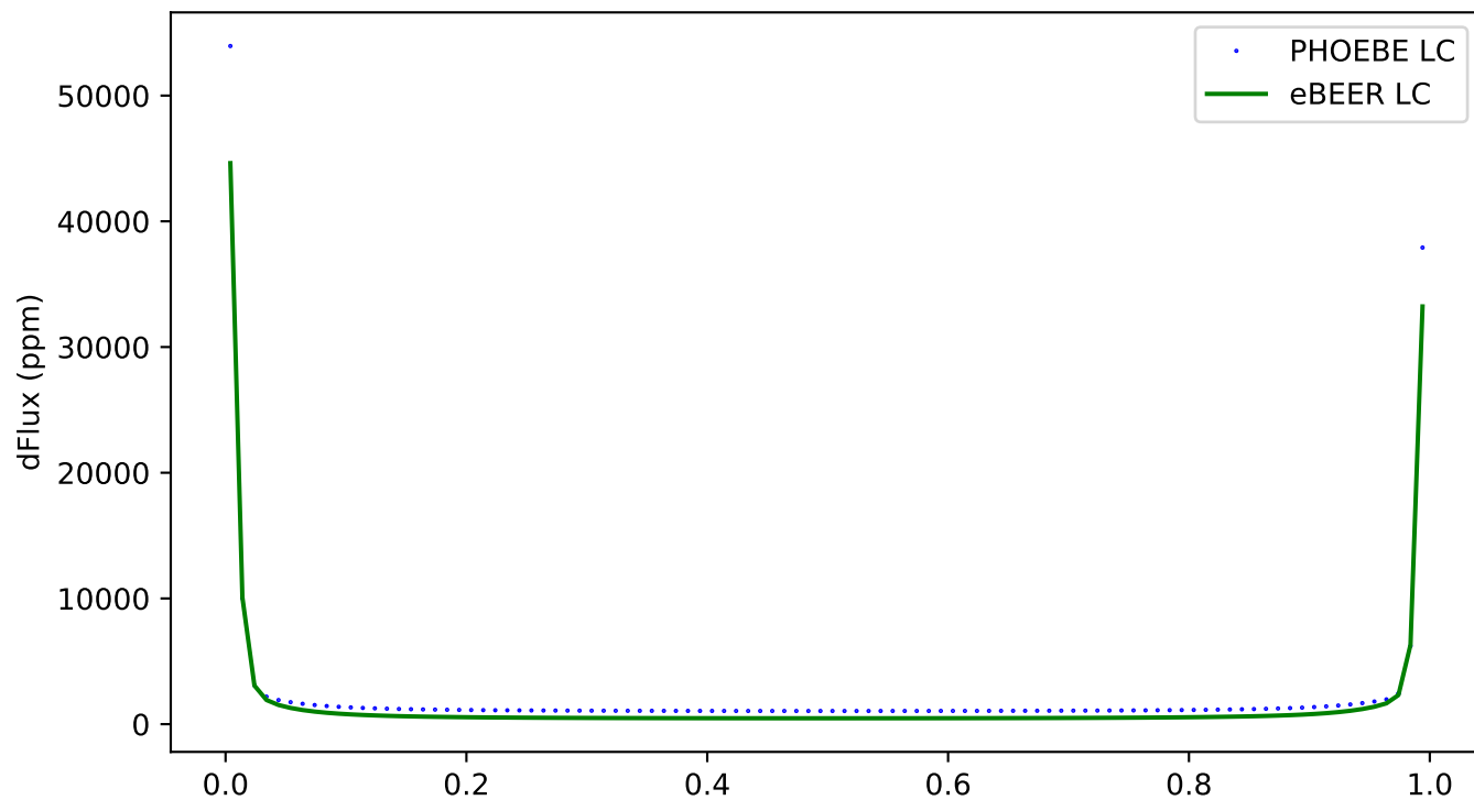
284 - ecc:0.8, incl:30, \omega :180, Porb:1, q:2
