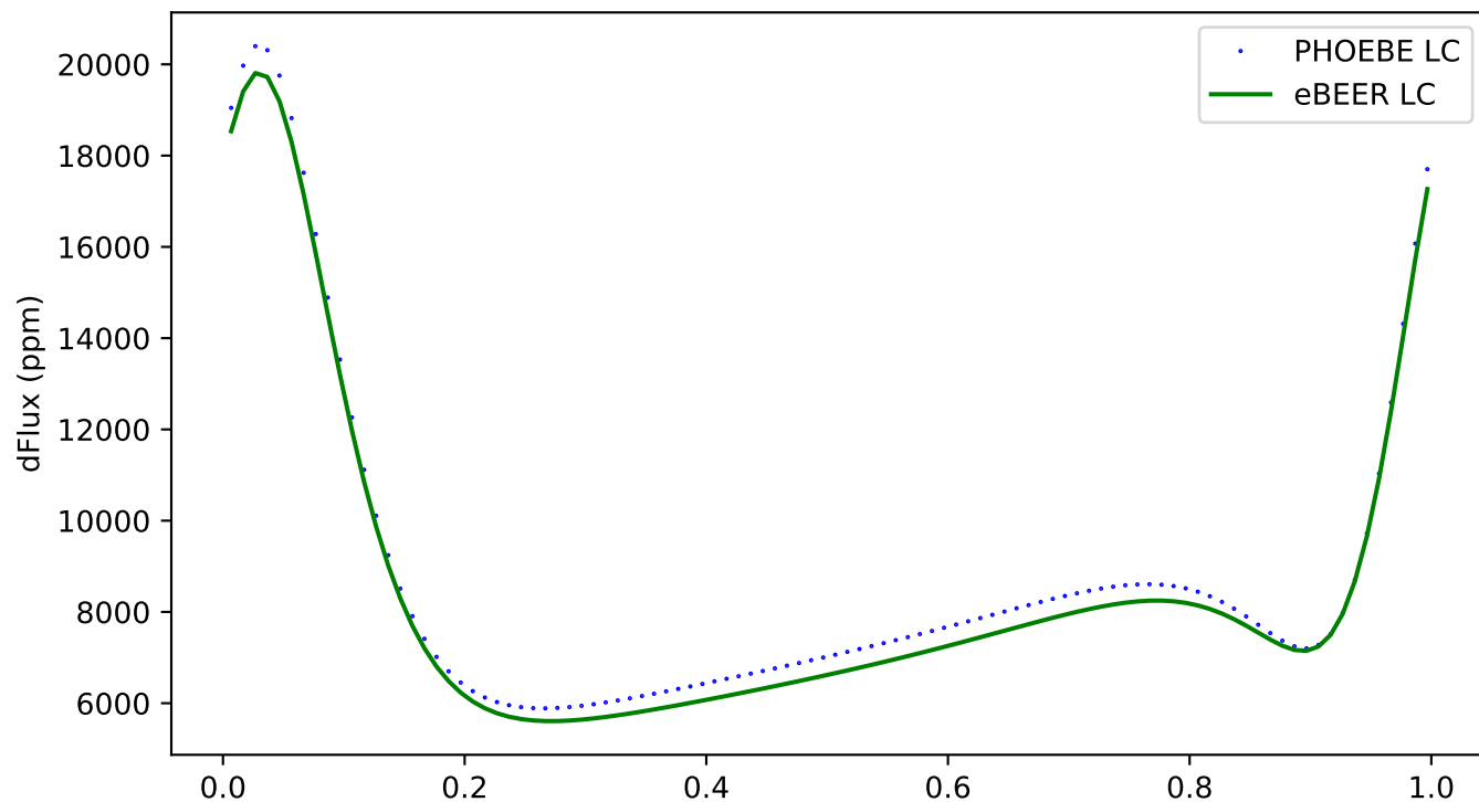
225 - ecc:0.3, incl:150, \omega :150, Porb:1, q:1
