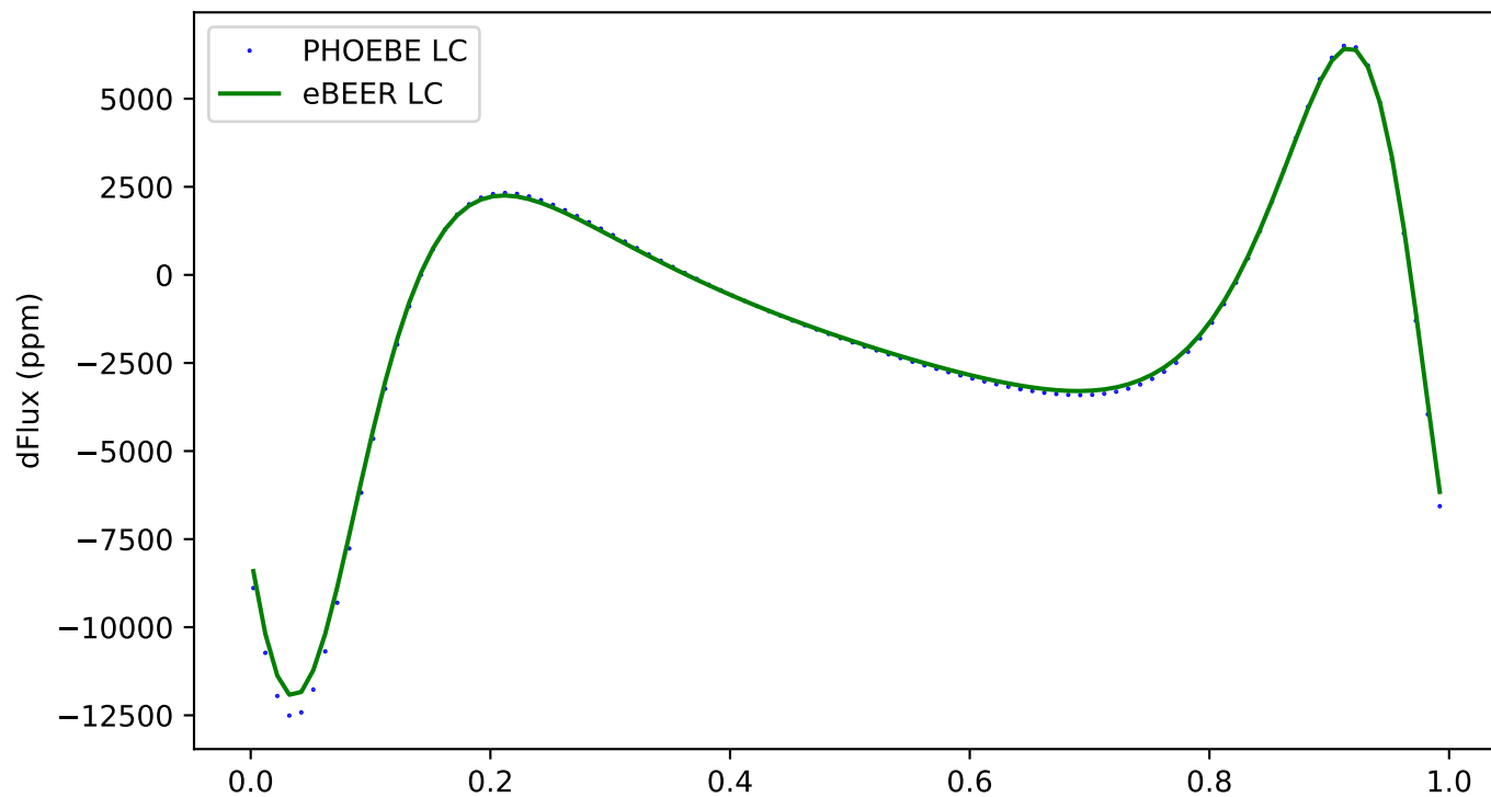
178 - ecc:0.3, incl:60, \omega :240, Porb:1, q:0.5
