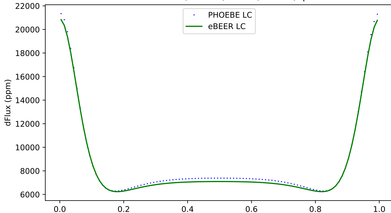
156 - ecc:0.3, incl:30, \omega :180, Porb:1, q:1
