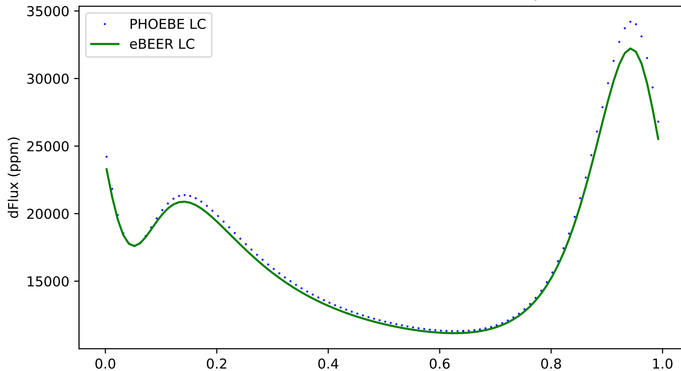
233 - ecc:0.3, incl:150, \omega :240, Porb:1, q:2
