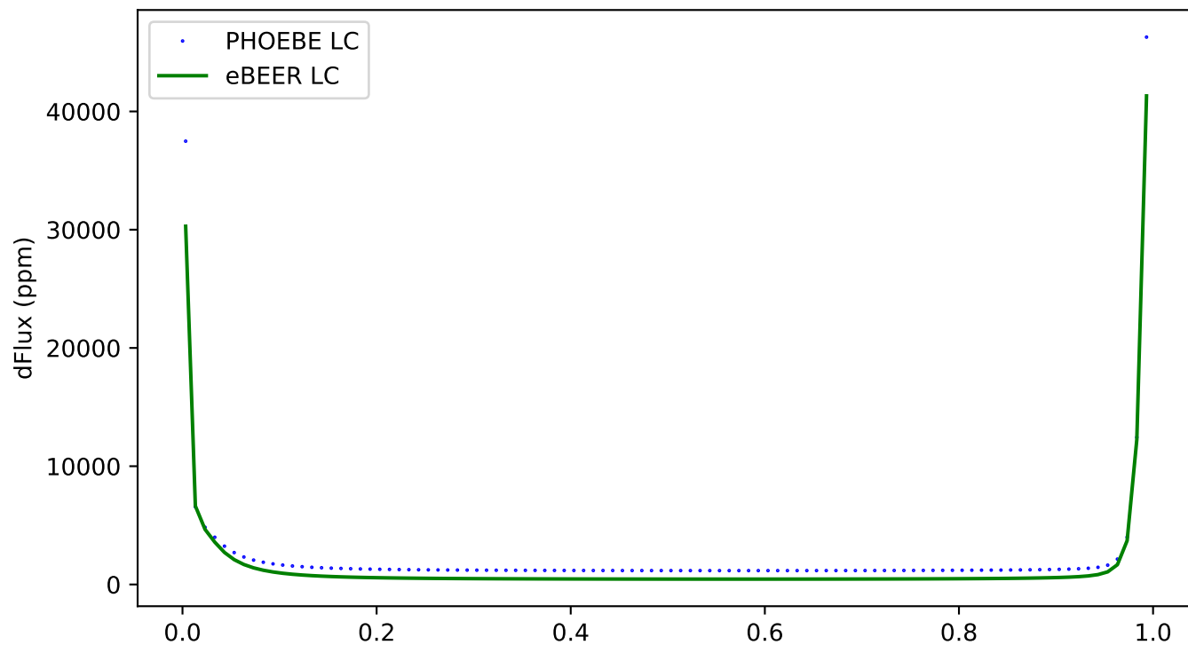
346 - ecc:0.8, incl:150, \omega :30, Porb:1, q:0.5
