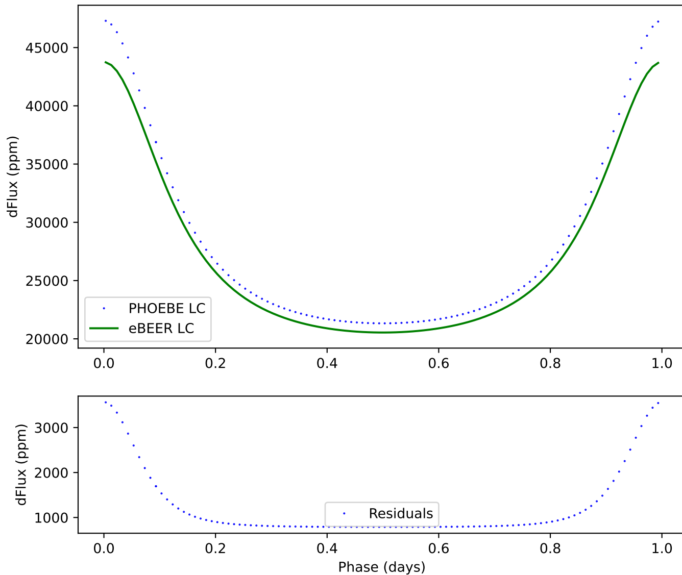
131 - ecc:0.3, incl:0, \omega :30, Porb:1, q:2
