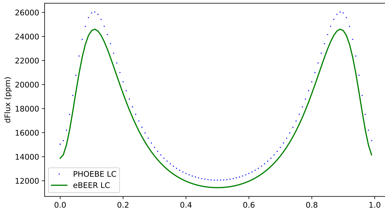
224 - ecc:0.3, incl:150, \omega :90, Porb:1, q:2
