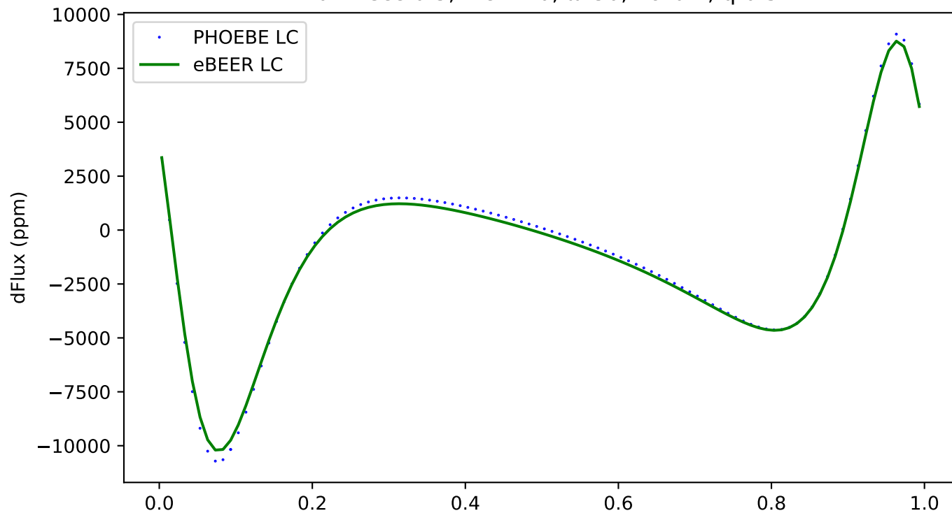
202 - ecc:0.3, incl:120, \omega :30, Porb:1, q:0.5
