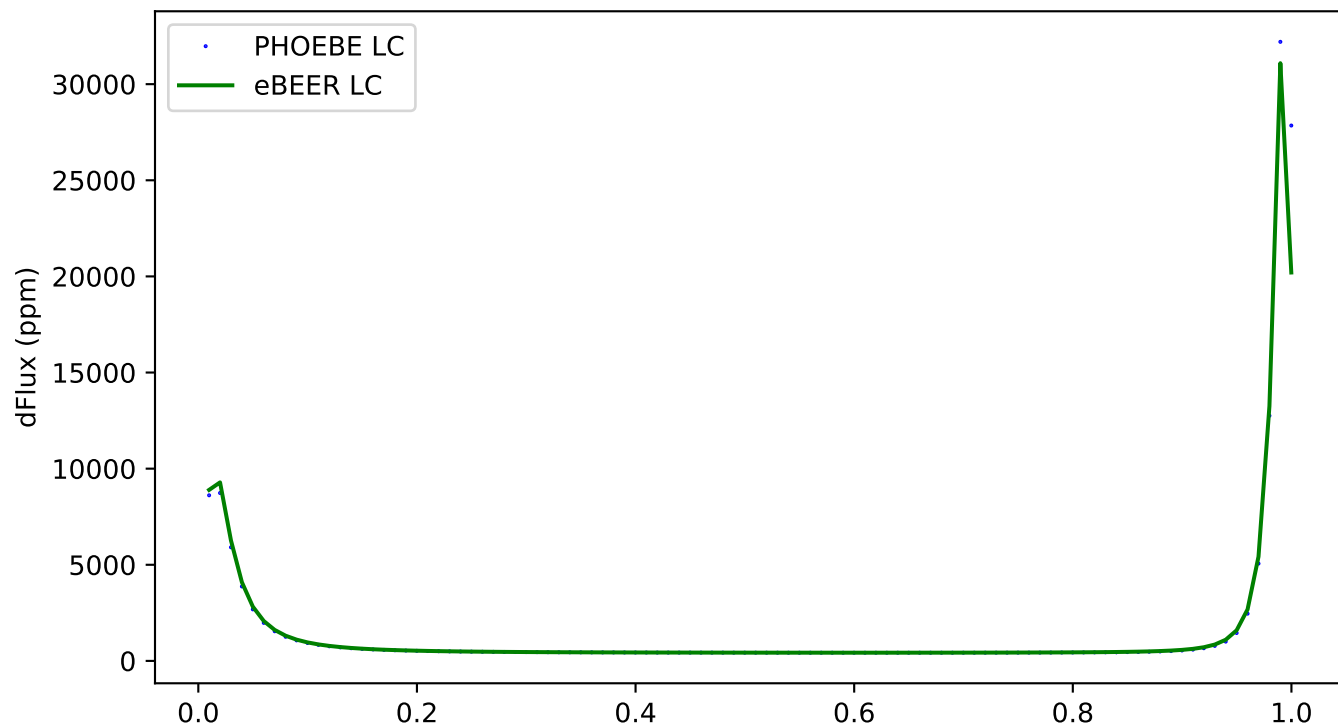
286 - ecc:0.8, incl:30, \omega :240, Porb:1, q:0.5
