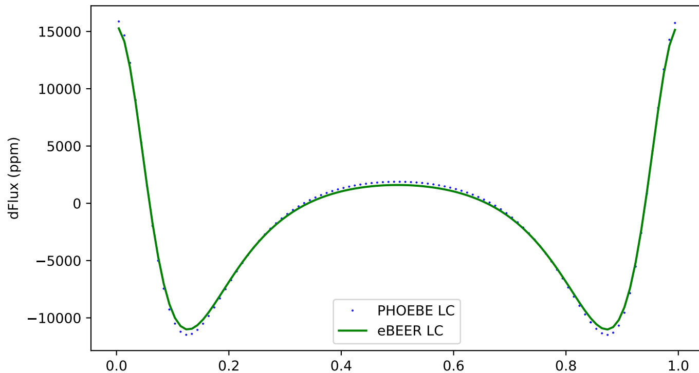
174 - ecc:0.3, incl:60, \omega :180, Porb:1, q:1
