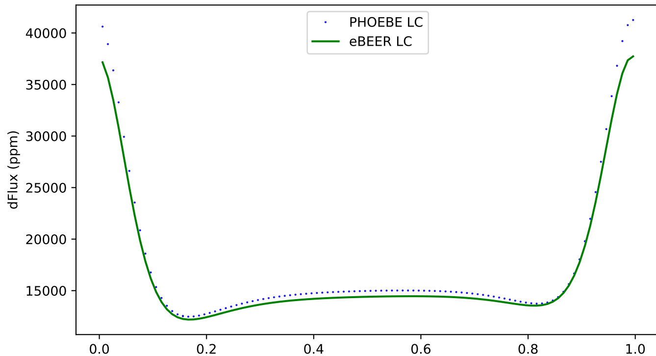
146 - ecc:0.3, incl:30, \omega :0, Porb:1, q:2
