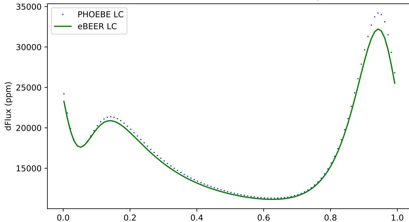
161 - ecc:0.3, incl:30, \omega :240, Porb:1, q:2
