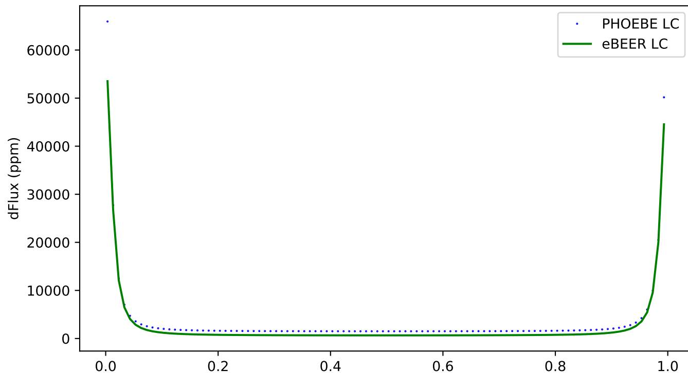
255 - ecc:0.8, incl:0, \omega :30, Porb:1, q:1
