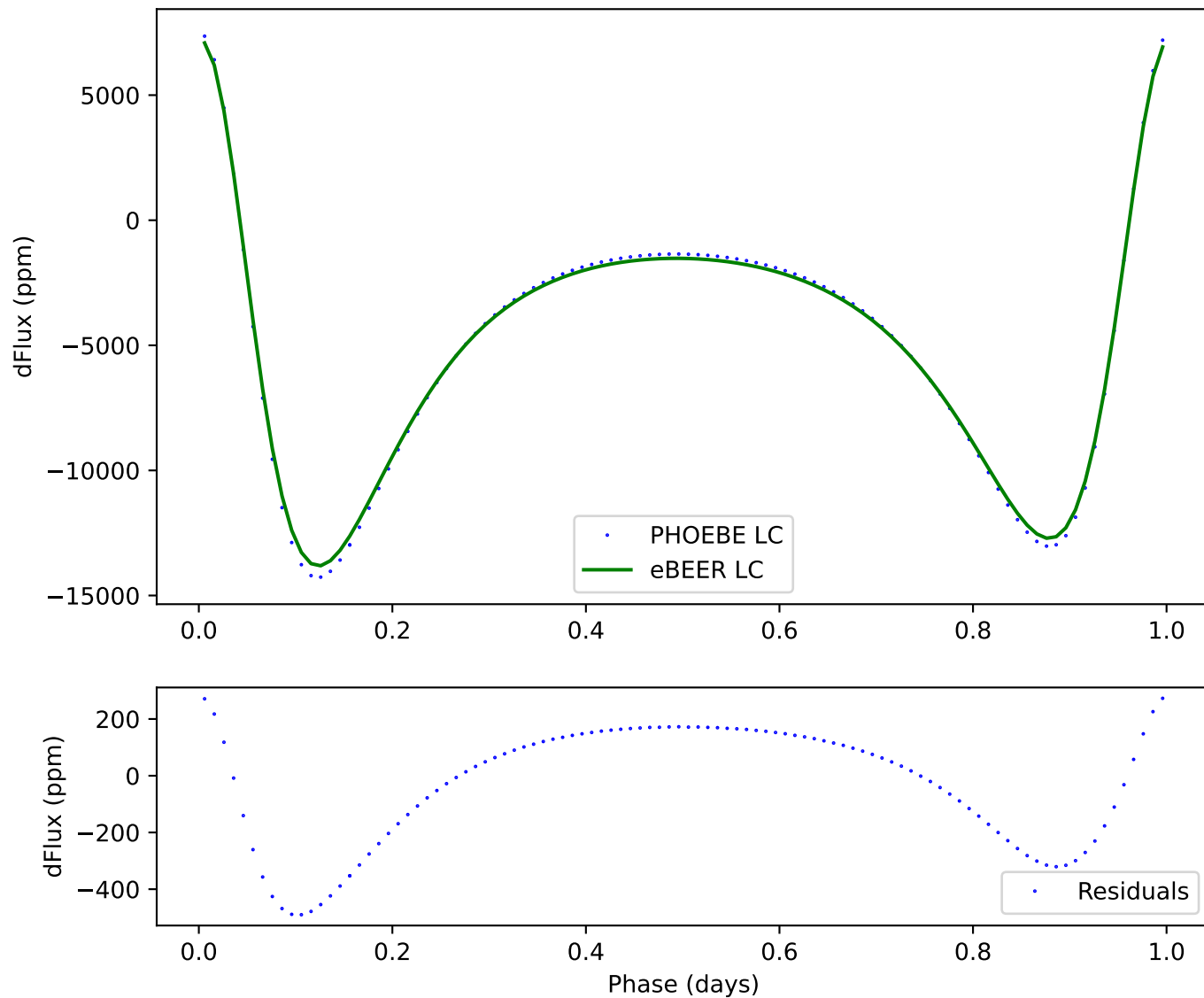
181 - ecc:0.3, incl:90, \omega :0, Porb:1, q:0.5
