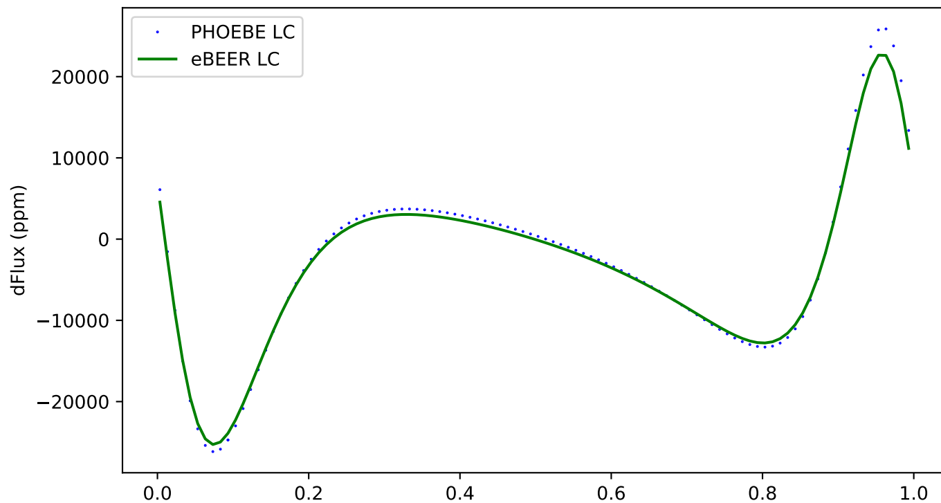
203 - ecc:0.3, incl:120, \omega :30, Porb:1, q:2
