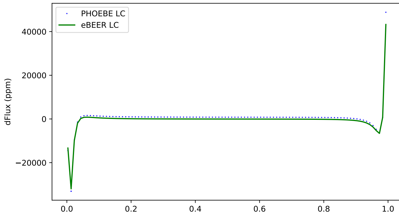
291 - ecc:0.8, incl:60, \omega :30, Porb:1, q:1
