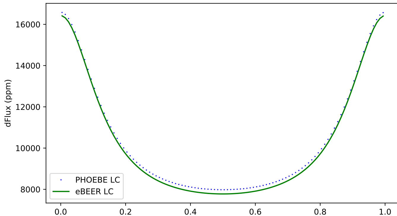
247 - ecc:0.3, incl:180, \omega :180, Porb:1, q:0.5
