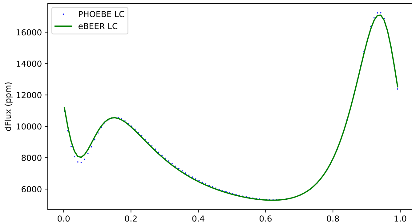
231 - ecc:0.3, incl:150, \omega :240, Porb:1, q:1
