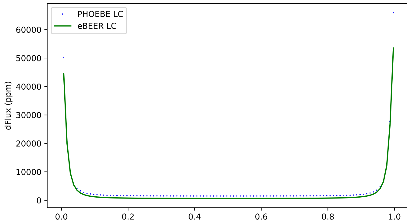
261 - ecc:0.8, incl:0, \omega :150, Porb:1, q:1
