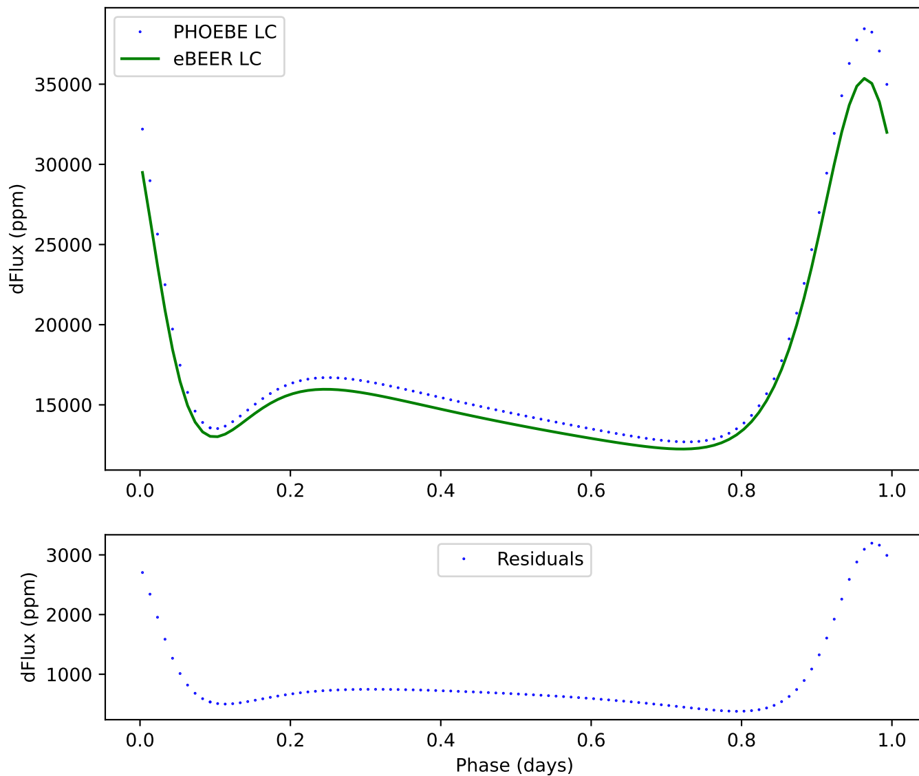
221 - ecc:0.3, incl:150, \omega :30, Porb:1, q:2
