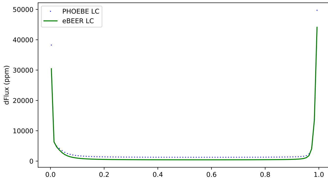
345 - ecc:0.8, incl:150, \omega :30, Porb:1, q:1
