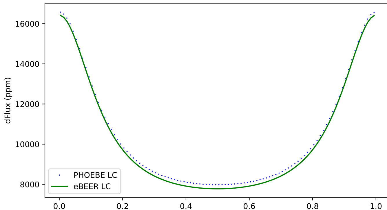
139 - ecc:0.3, incl:0, \omega :180, Porb:1, q:0.5
