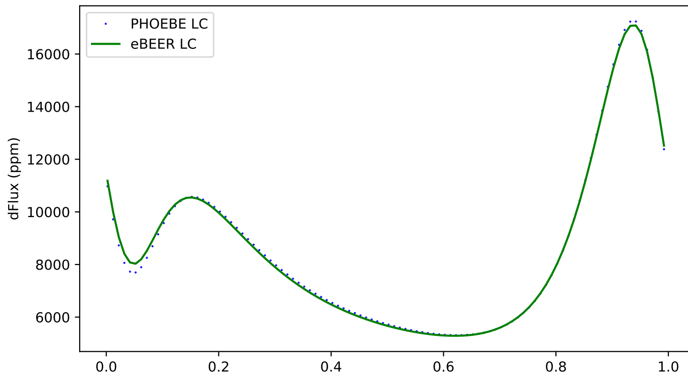
159 - ecc:0.3, incl:30, \omega :240, Porb:1, q:1
