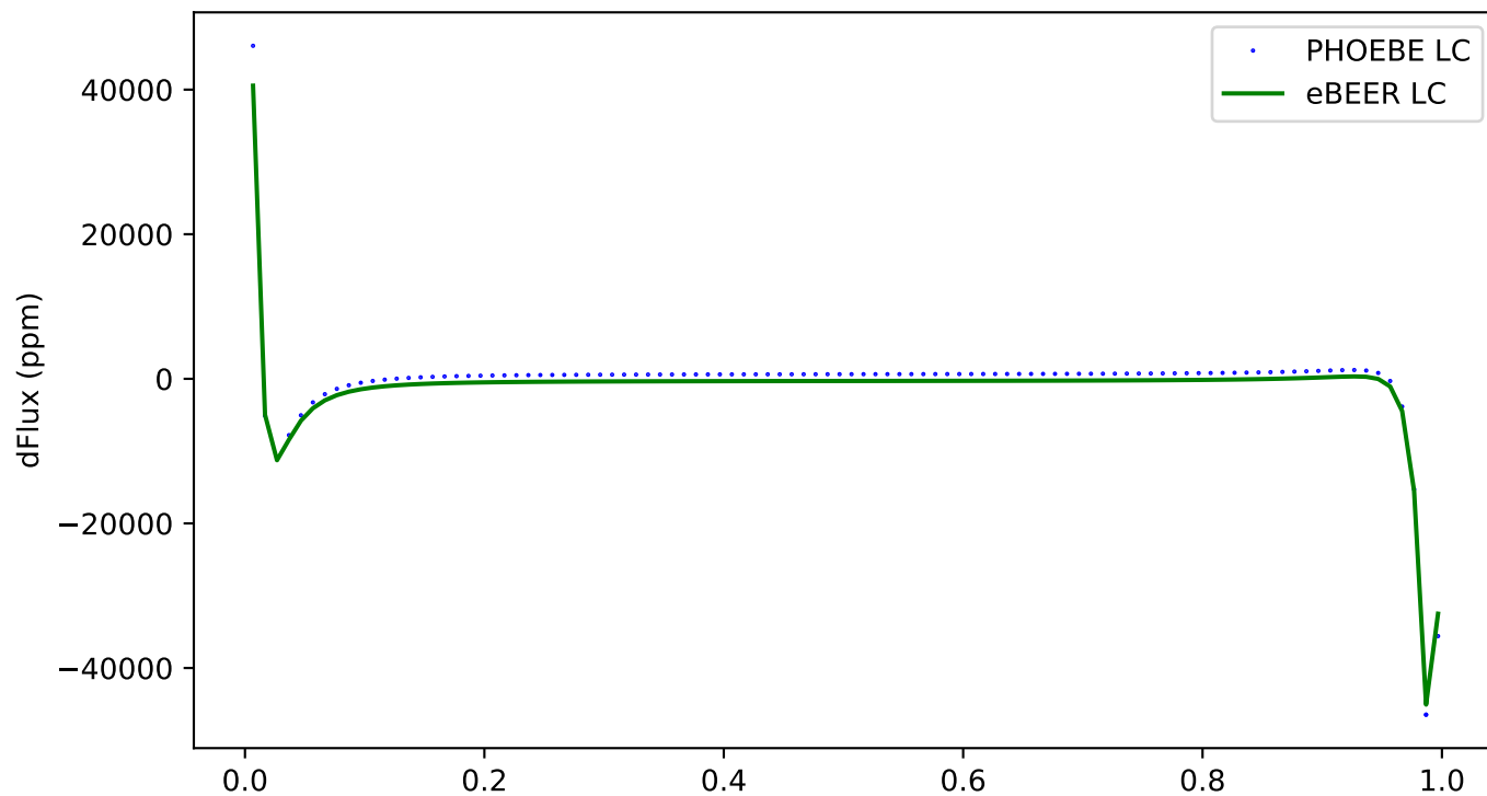
317 - ecc:0.8, incl:90, \omega :150, Porb:1, q:2
