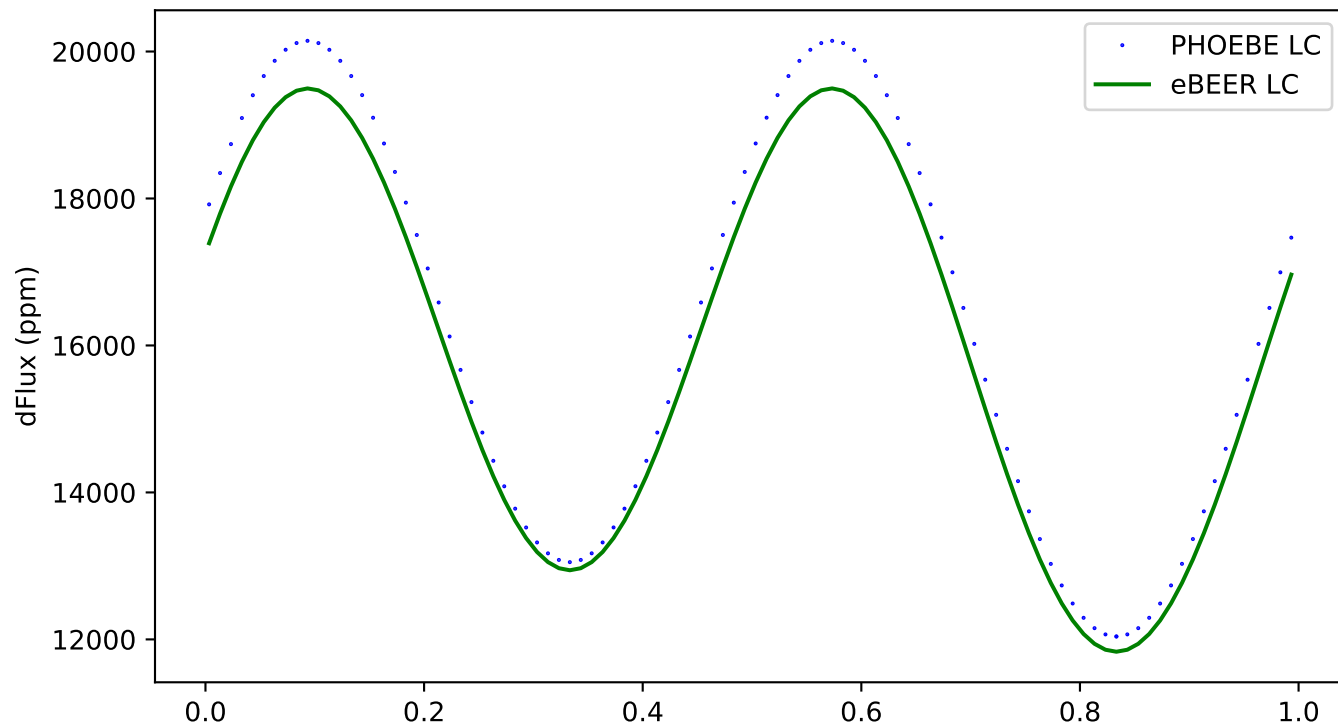
29 - ecc:0, incl:30, \omega :150, Porb:1, q:2
