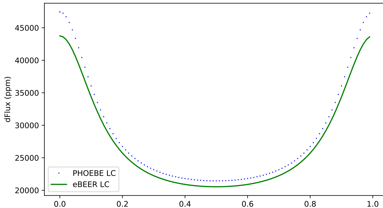
134 - ecc:0.3, incl:0, \omega :90, Porb:1, q:2
