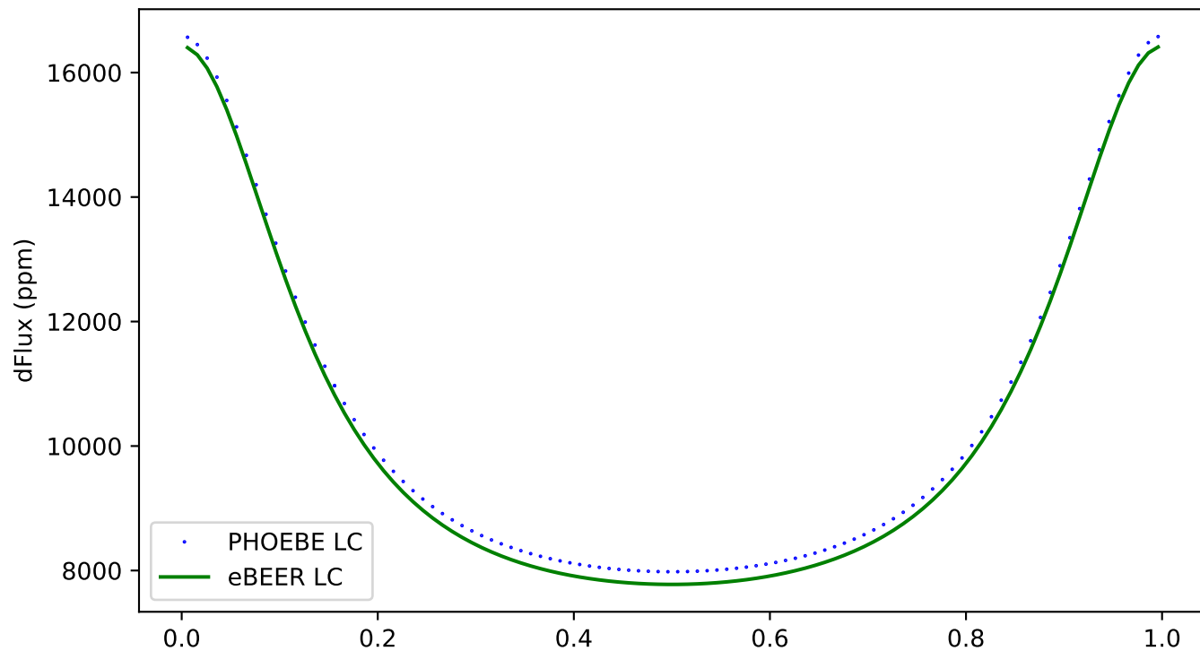
127 - ecc:0.3, incl:0, \omega :0, Porb:1, q:0.5
