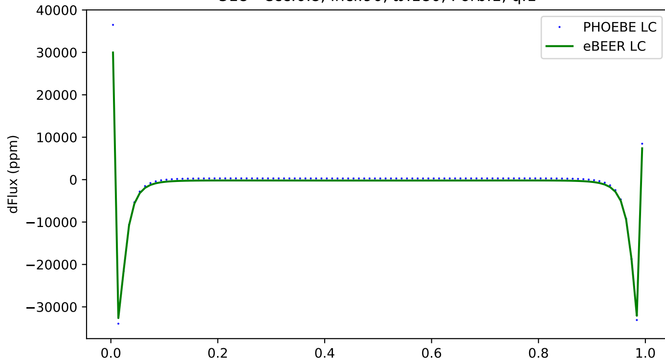
318 - ecc:0.8, incl:90, \omega :180, Porb:1, q:1
