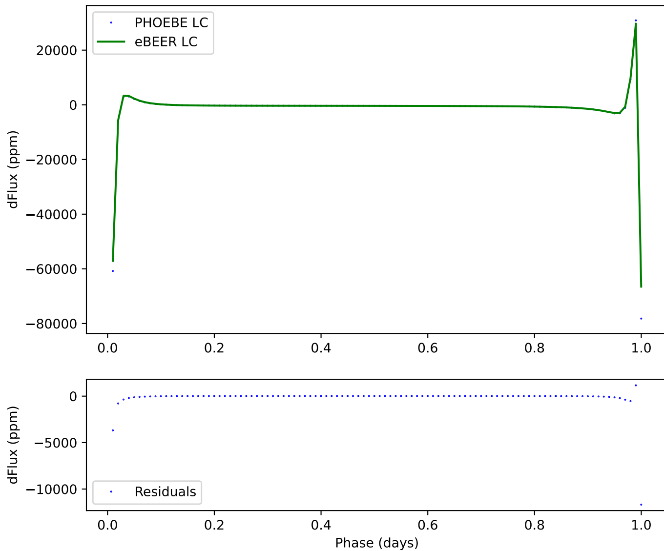
321 - ecc:0.8, incl:90, \omega :240, Porb:1, q:1
