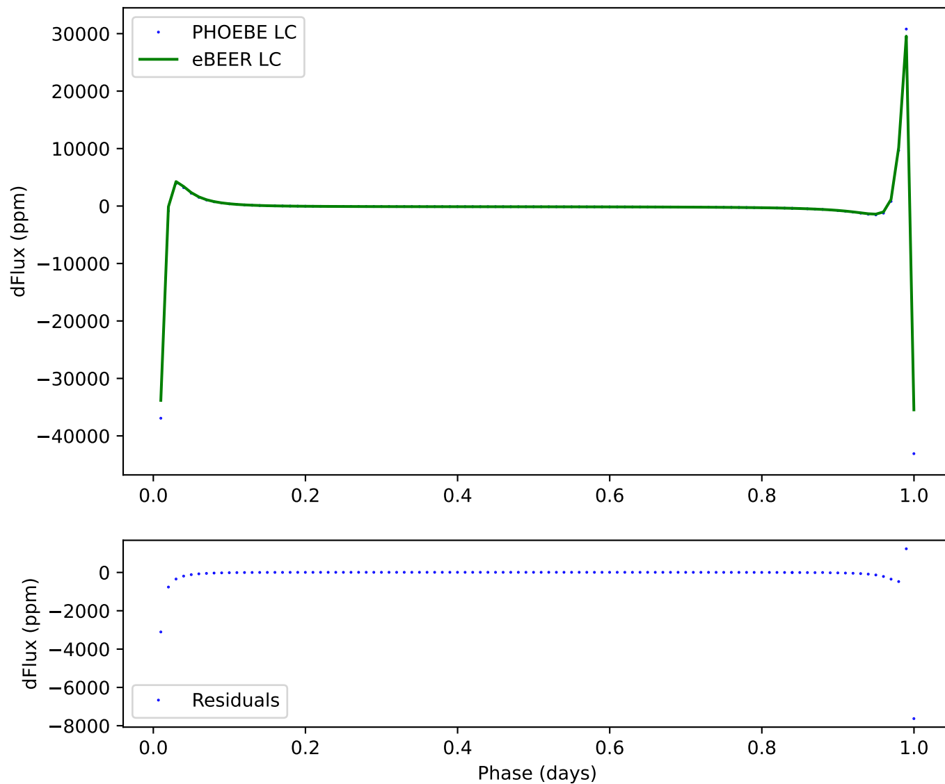
341 - ecc:0.8, incl:120, \omega :240, Porb:1, q:2
