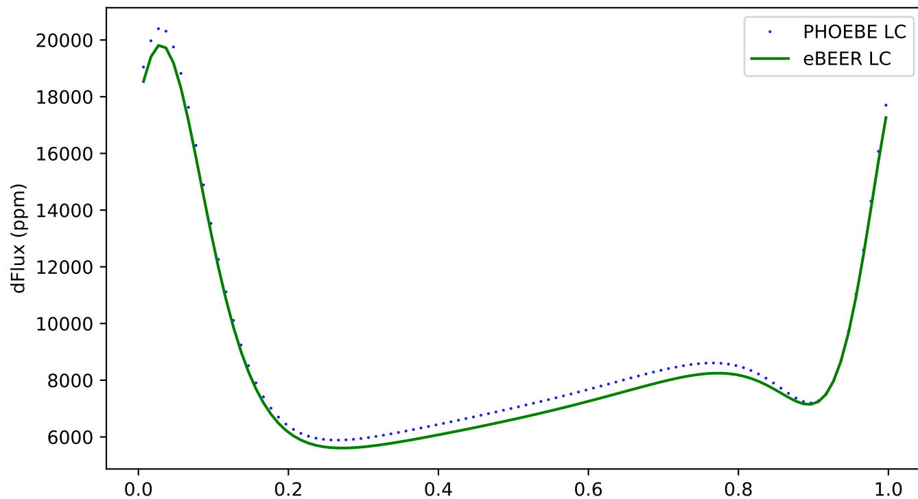
153 - ecc:0.3, incl:30, \omega :150, Porb:1, q:1
