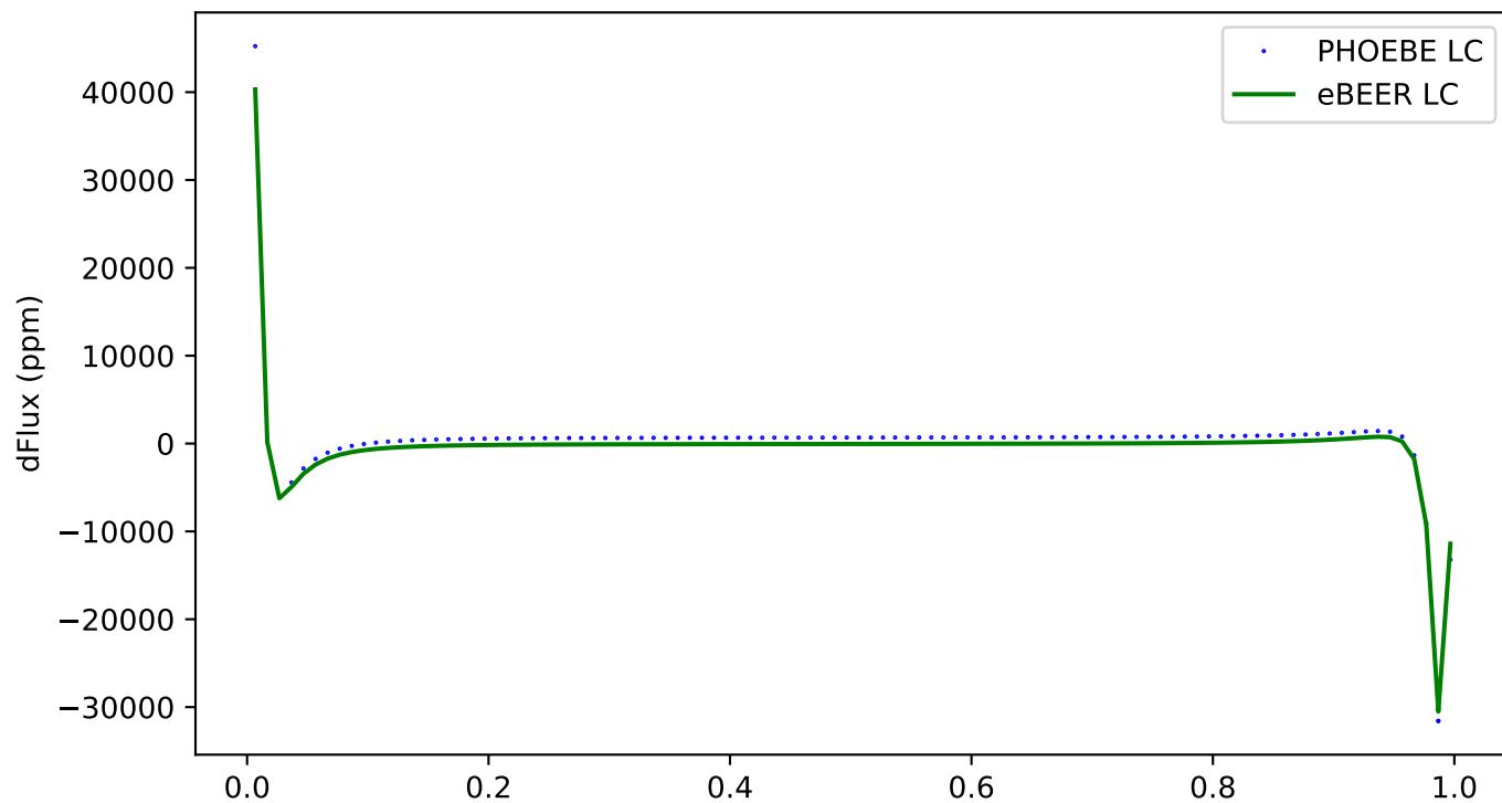
298 - ecc:0.8, incl:60, \omega :150, Porb:1, q:0.5
