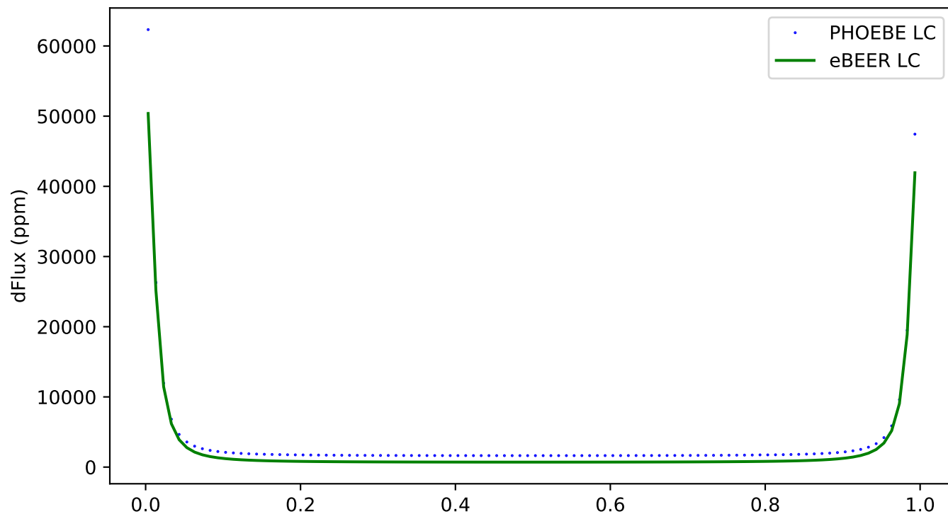
257 - ecc:0.8, incl:0, \omega :30, Porb:1, q:2
