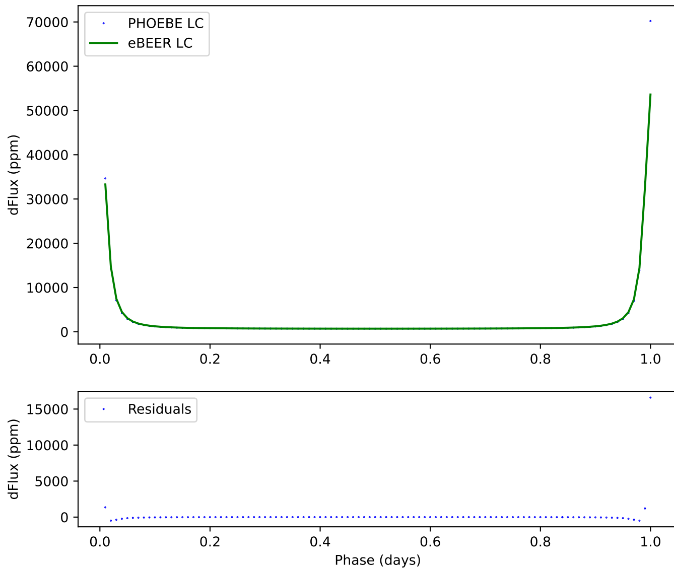
268 - ecc:0.8, incl:0, \omega :240, Porb:1, q:0.5
