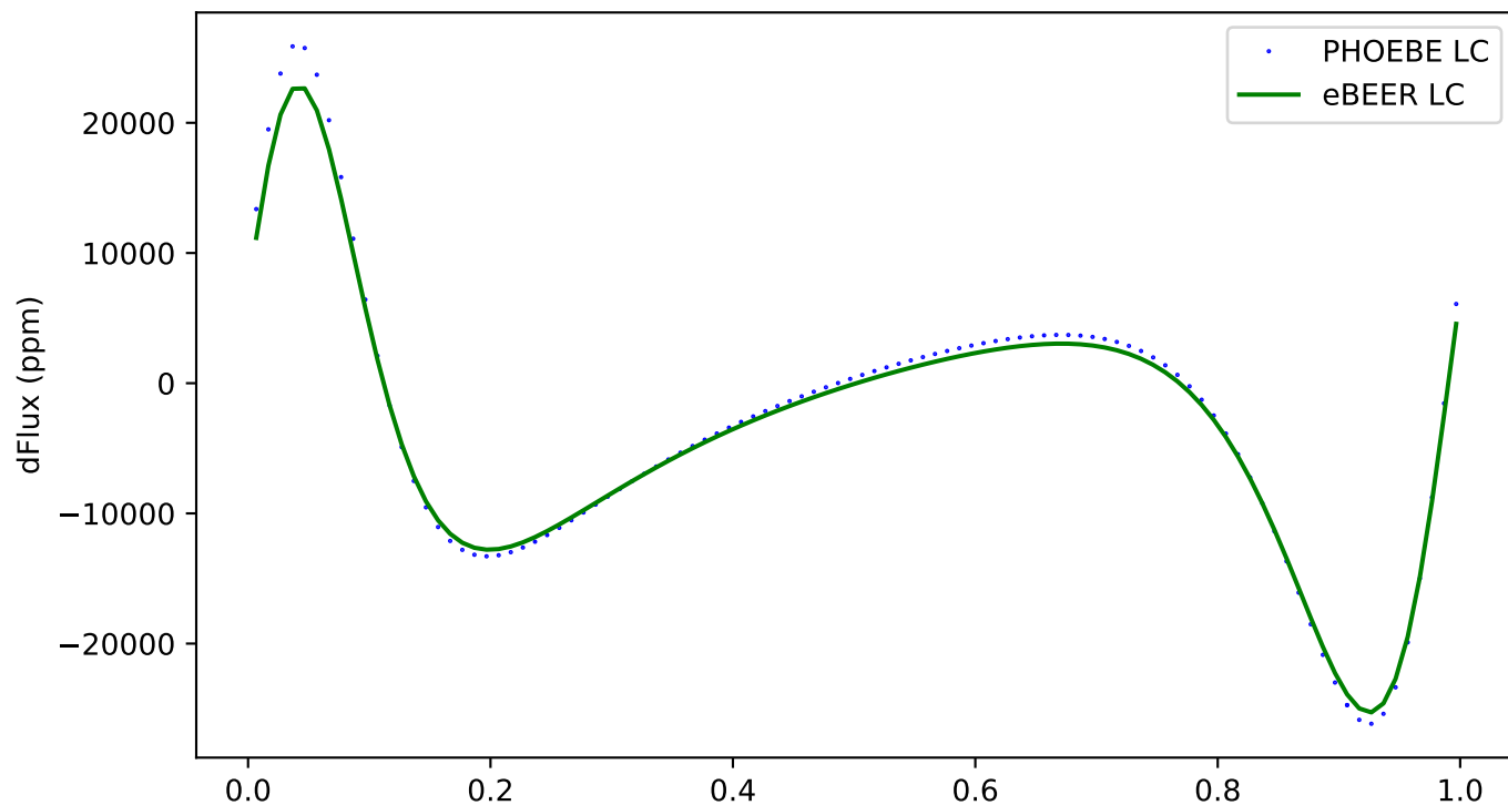
209 - ecc:0.3, incl:120, \omega :150, Porb:1, q:2
