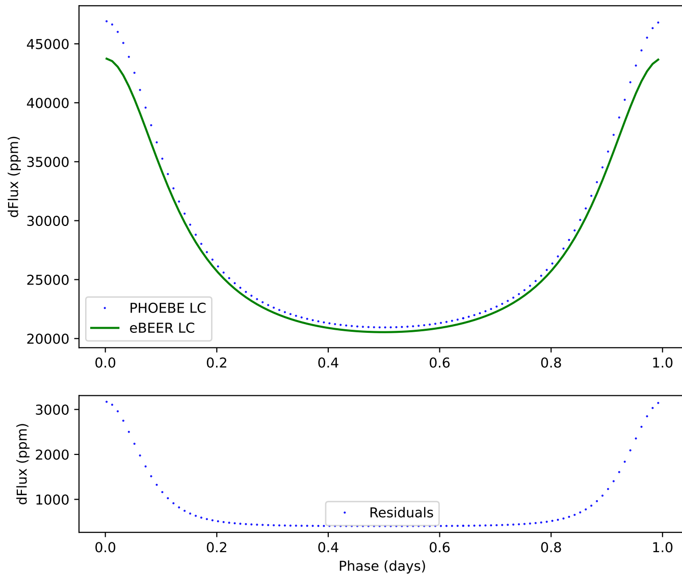
251 - ecc:0.3, incl:180, \omega :240, Porb:1, q:2
