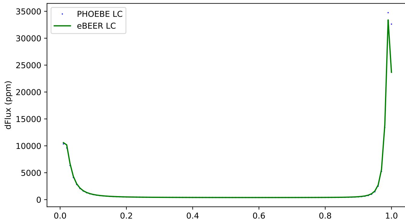
285 - ecc:0.8, incl:30, \omega :240, Porb:1, q:1
