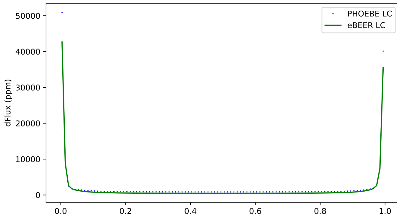
283 - ecc:0.8, incl:30, \omega :180, Porb:1, q:0.5
