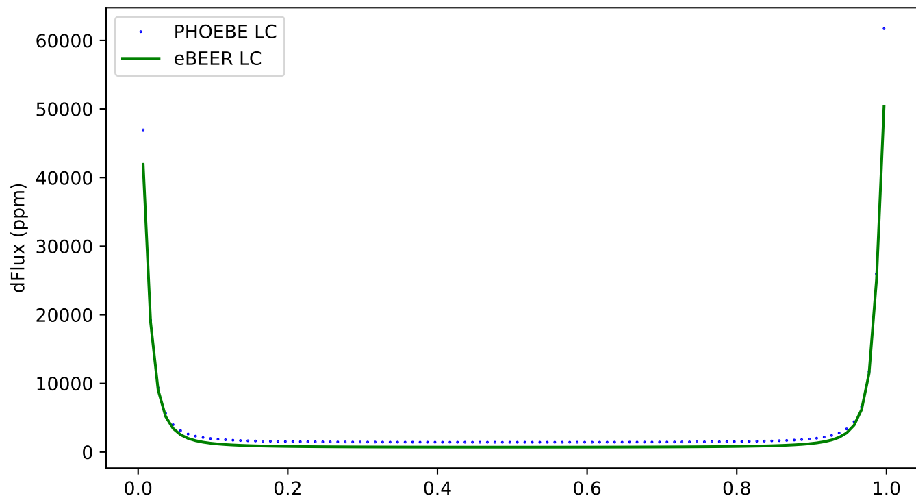
262 - ecc:0.8, incl:0, \omega :150, Porb:1, q:0.5
