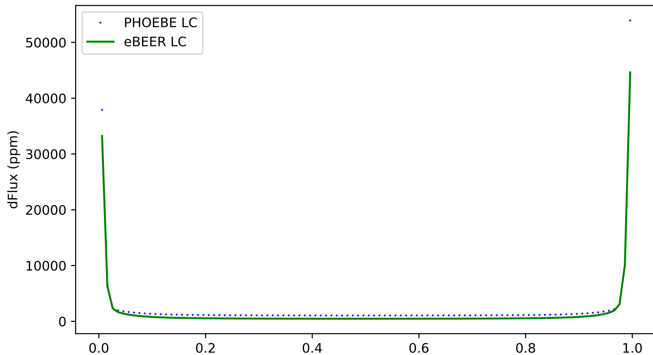
272 - ecc:0.8, incl:30, \omega :0, Porb:1, q:2
