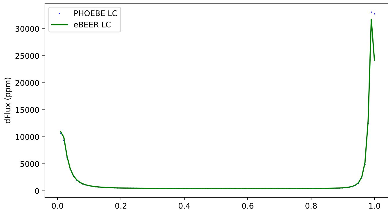
359 - ecc:0.8, incl:150, \omega :240, Porb:1, q:2
