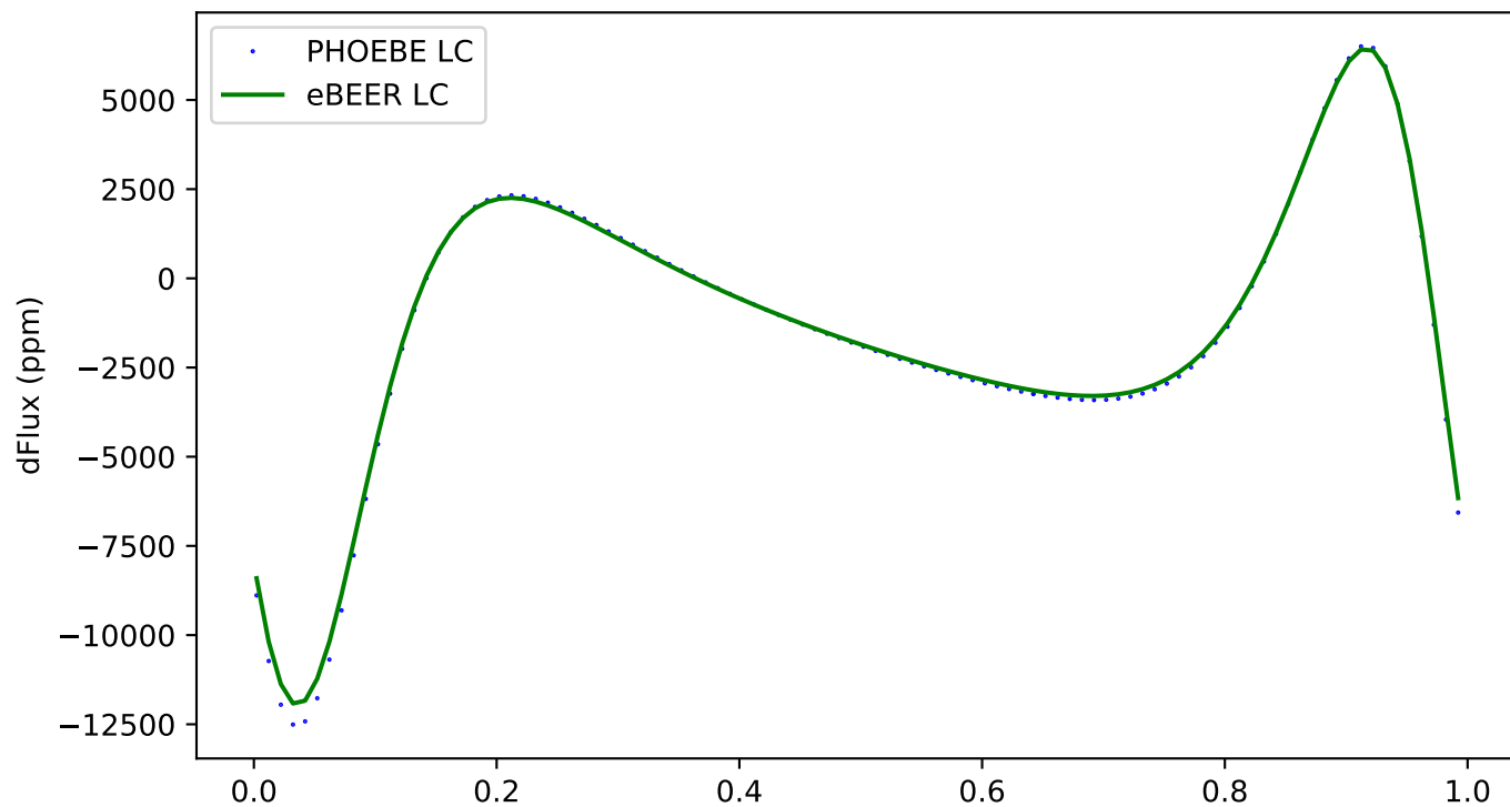
214 - ecc:0.3, incl:120, \omega :240, Porb:1, q:0.5
