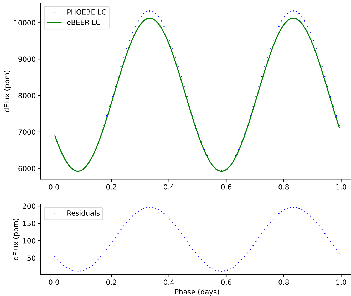
33 - ecc:0, incl:30, \omega :240, Porb:1, q:1
