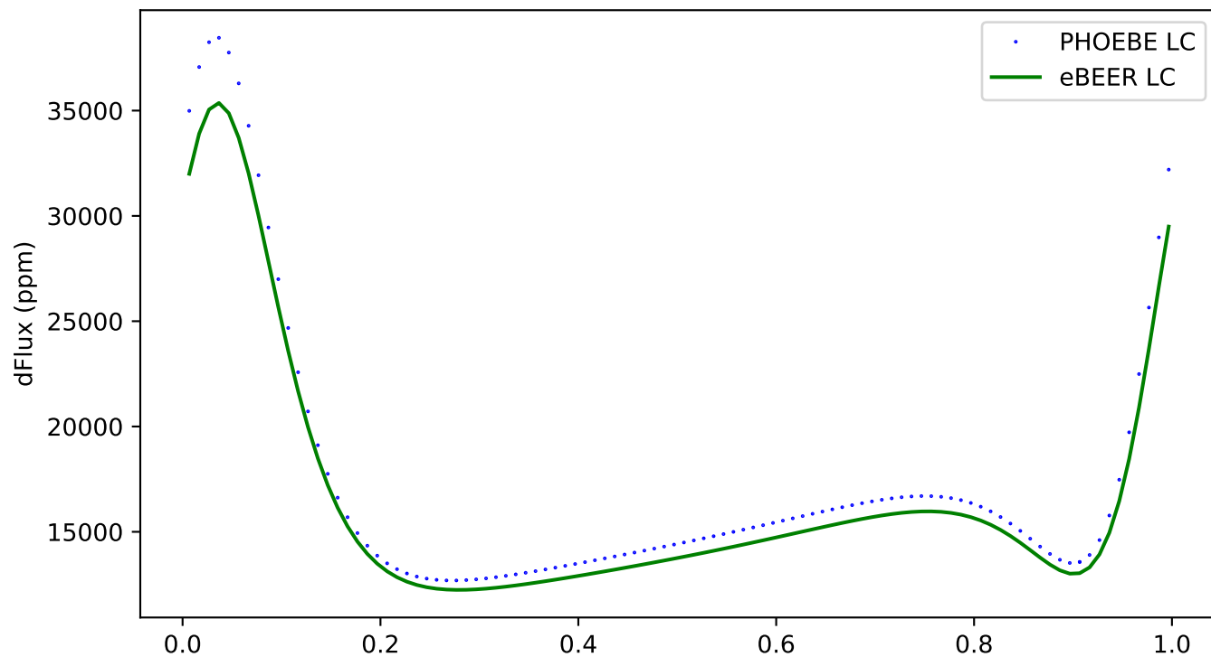
155 - ecc:0.3, incl:30, \omega :150, Porb:1, q:2
