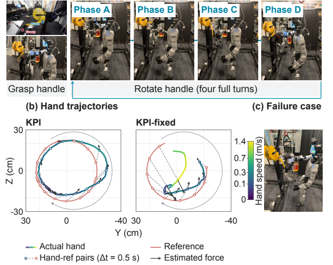
Fig. 5. Winch operation. (a) Handle acquisition and four phases of a revolution. (b) KPI and KPI-fixed’s hand trajectories. (c) MCC failure case.
