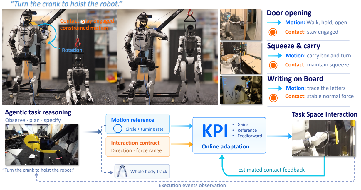
Fig. 1. KPI : a promptable kernel for physical interaction. KPI uses motion references, interaction contracts, and estimated contact feedback to adapt the arm controller, while an unmodified whole-body tracker controls the legs and waist. From one instruction, a humanoid turns a hand-winch to hoist a second robot. Further agentic demonstrations include door opening and box carrying; surface-interaction experiments include board writing.
