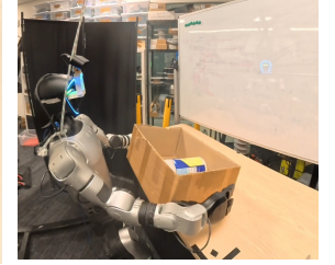
Fig. 7. Box transport and load robustness. (a) The five stages of transport and placement. (b) Maximum liftable load category. (c) Insufficient hand–box contact prevents lifting.
