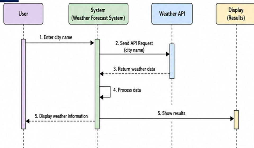
Figure: Sequence Diagram of Weather Forecast System
