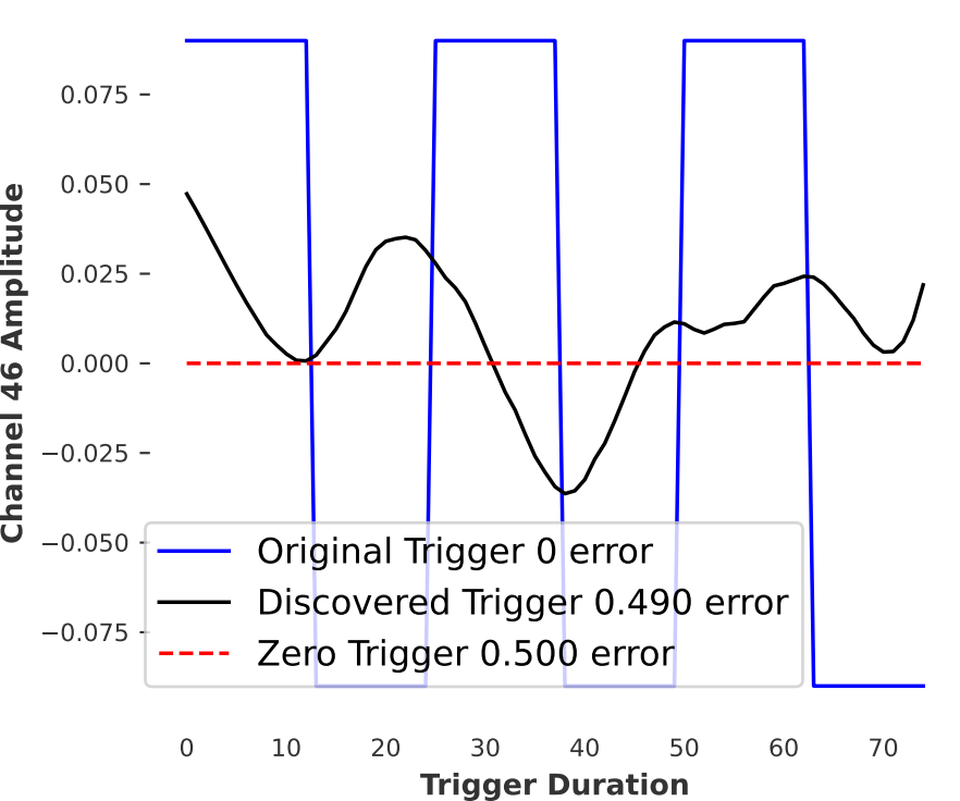
Discovered Trigger - Channel 46
