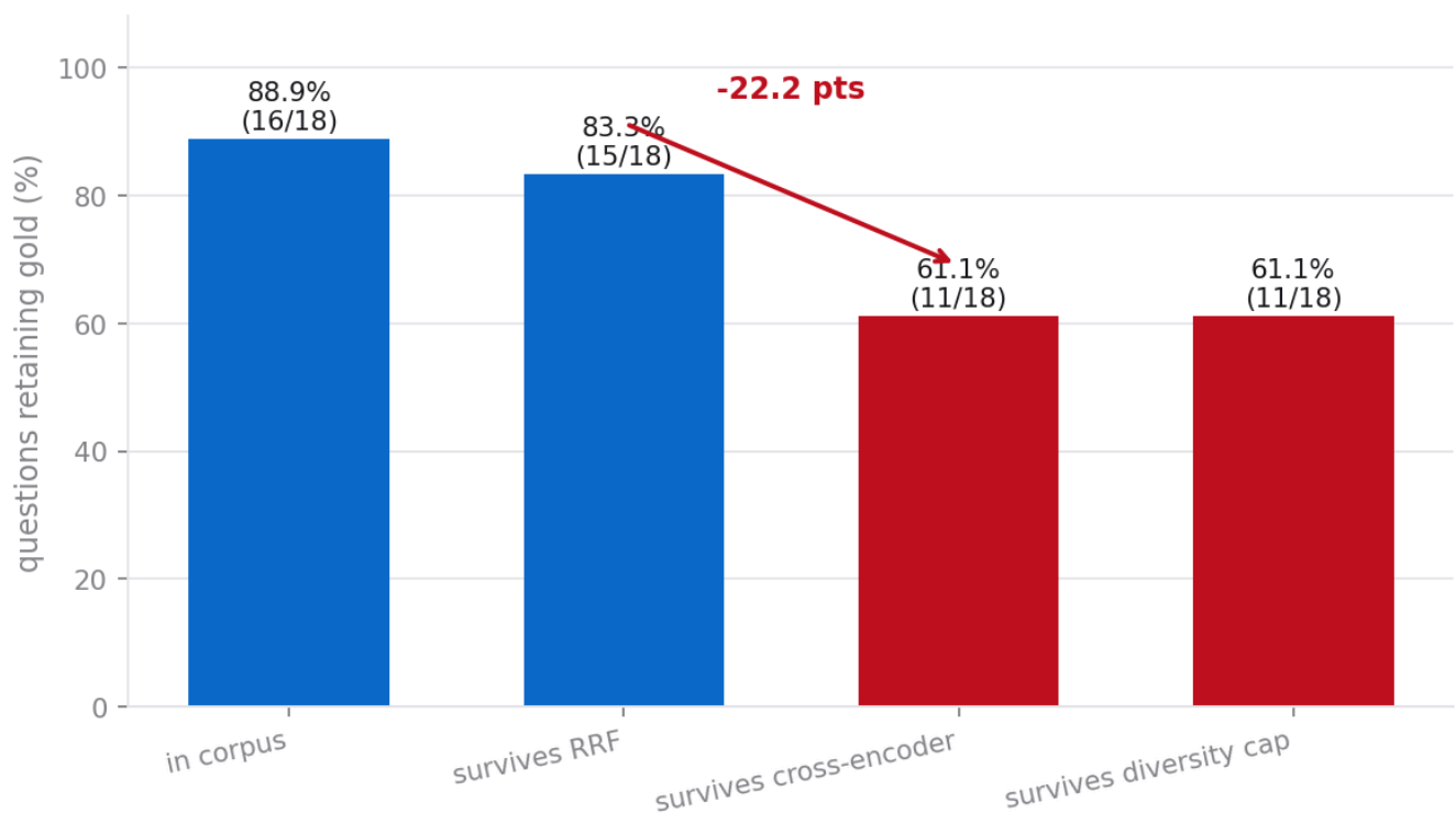
Where retrieval recall is lost
