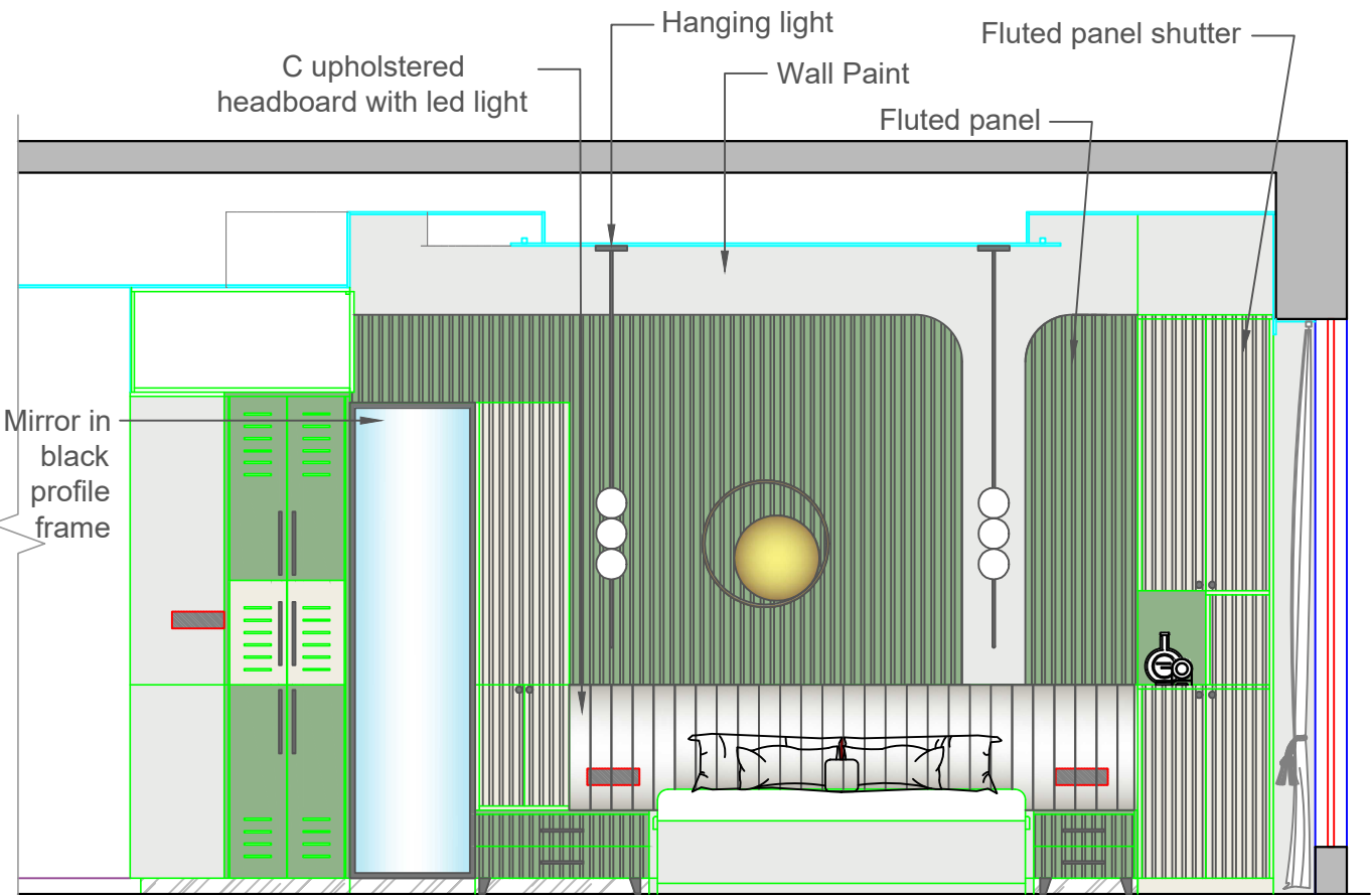
SECTION D-D'
