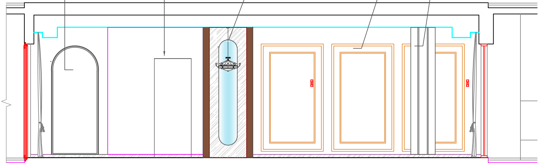
SECTION B-B'
