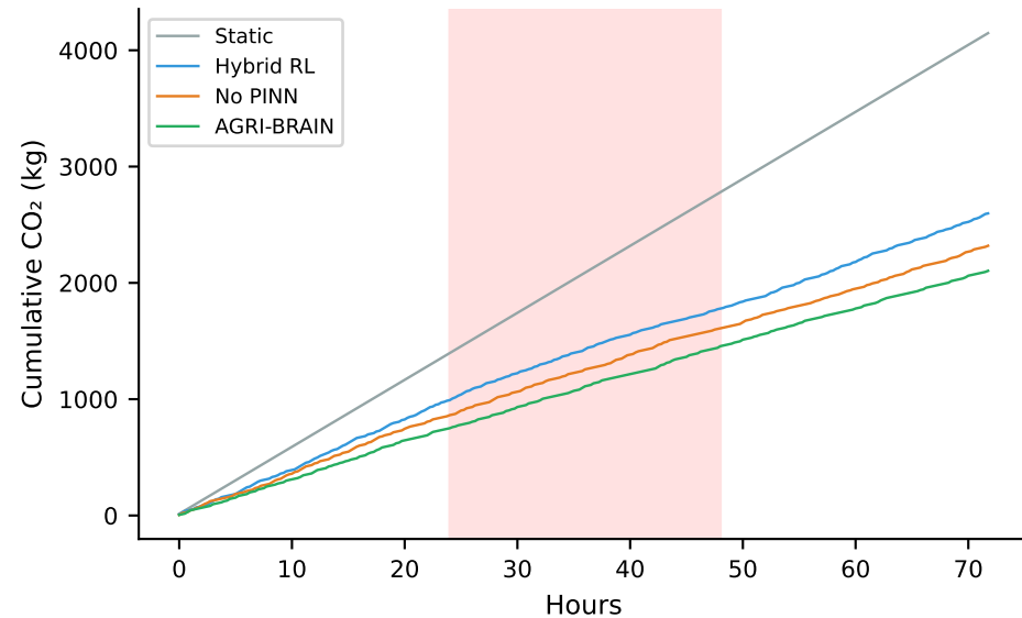
(a) Cumulative Carbon — Heatwave
