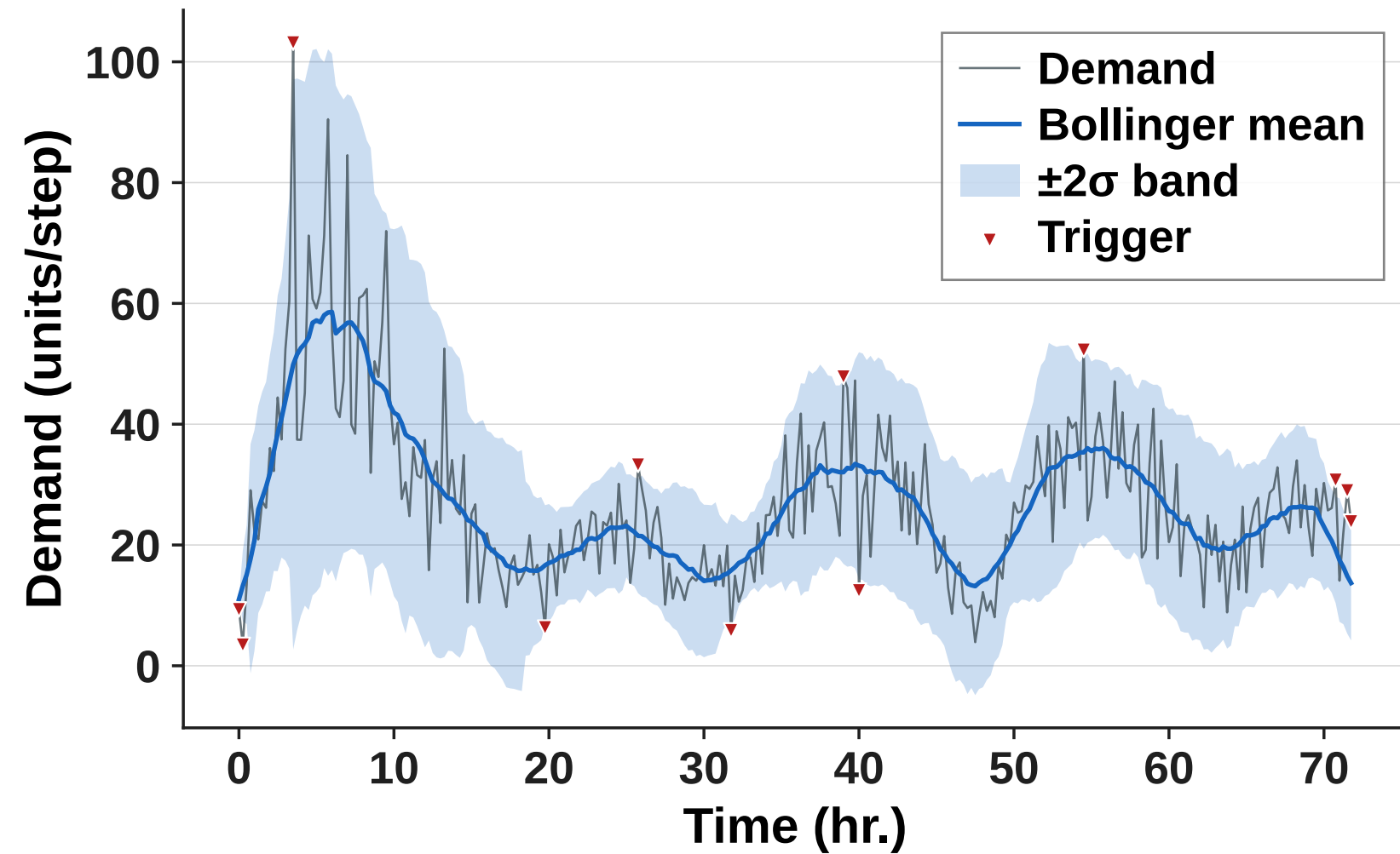
(a) Demand with Bollinger Triggers
