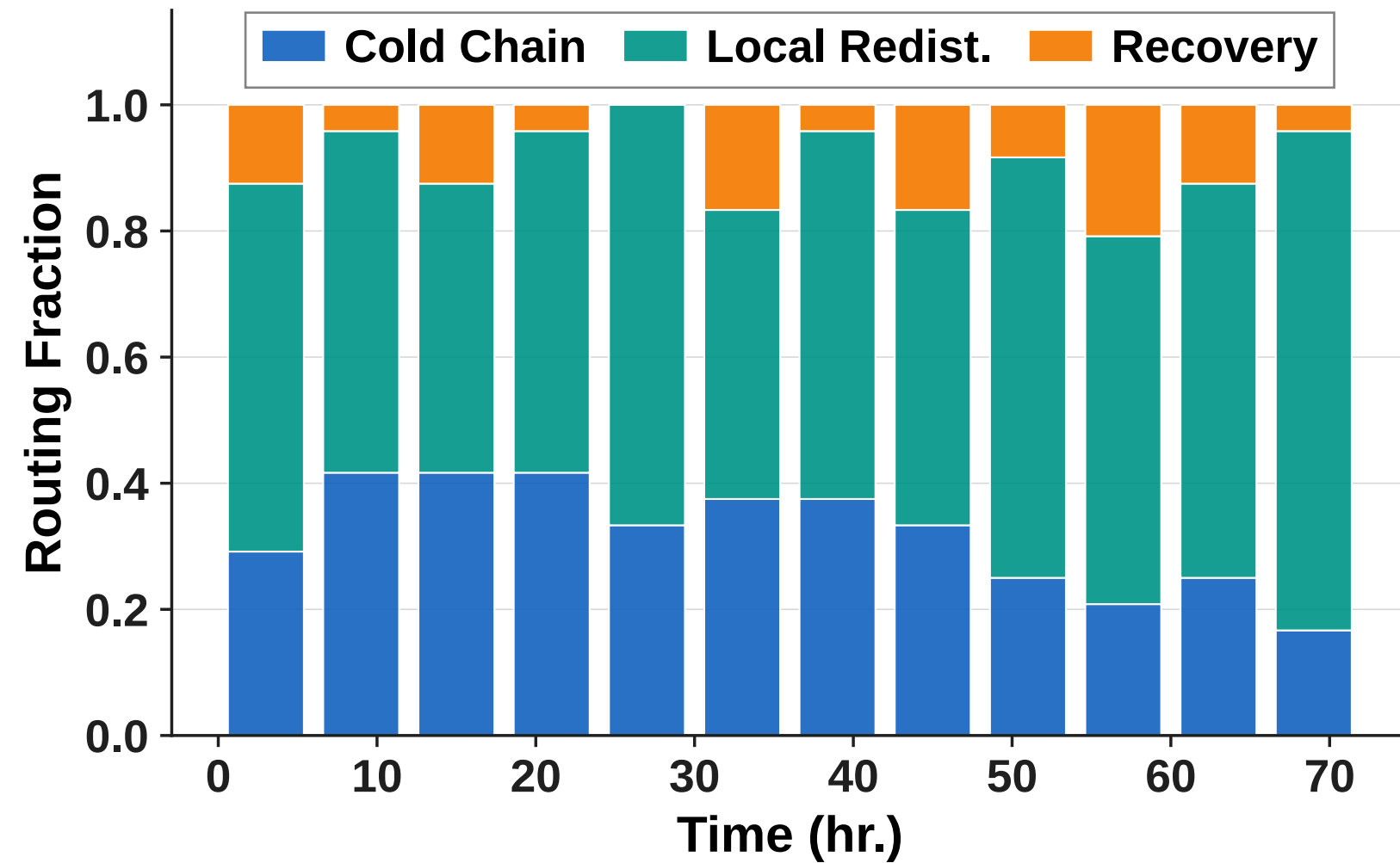
(b) Routing Distribution over Time
