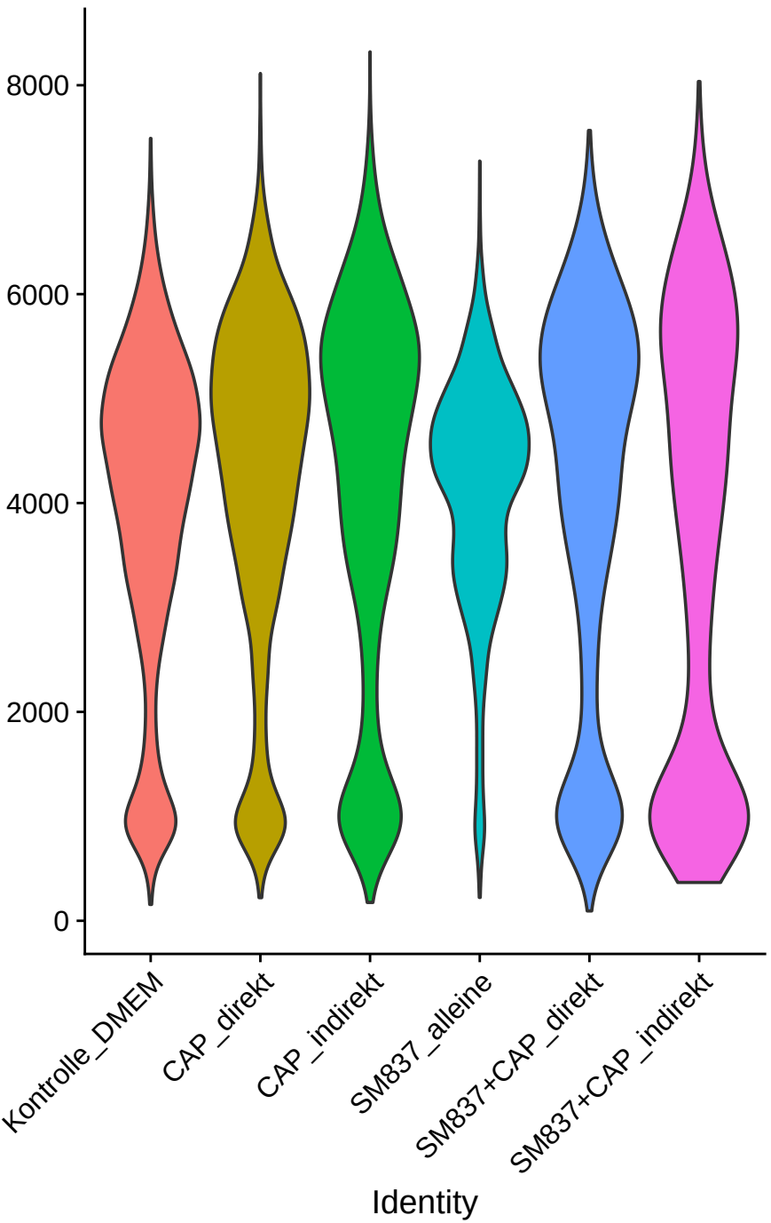
nFeature_RNA
