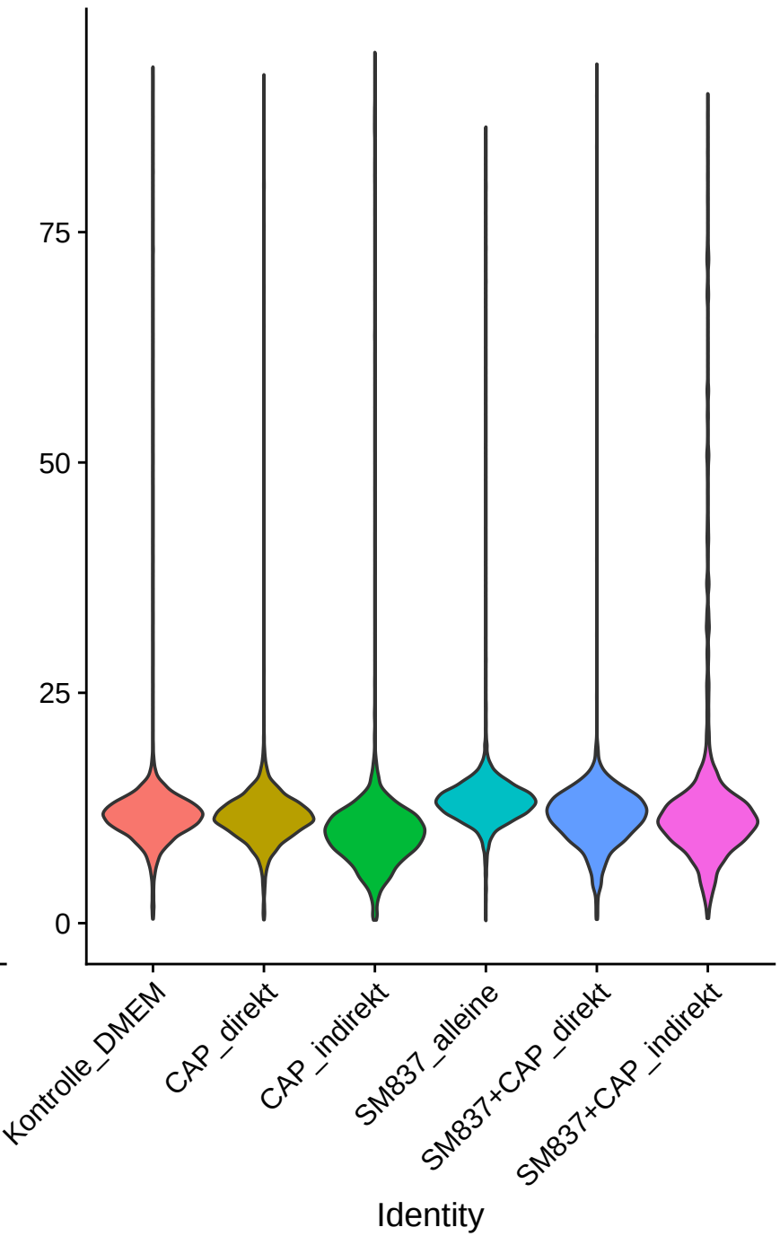
percent.mt
