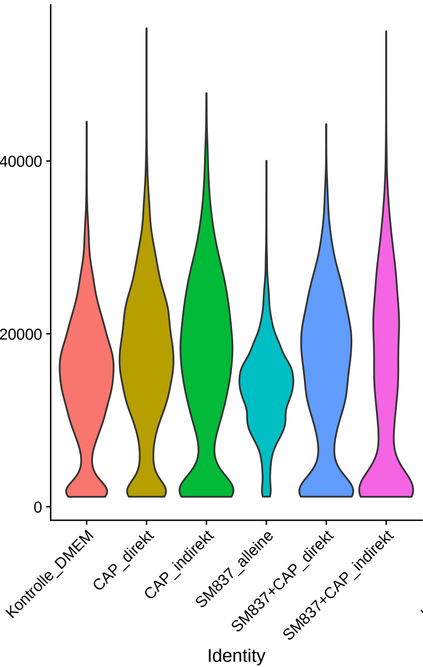
nCount_RNA
