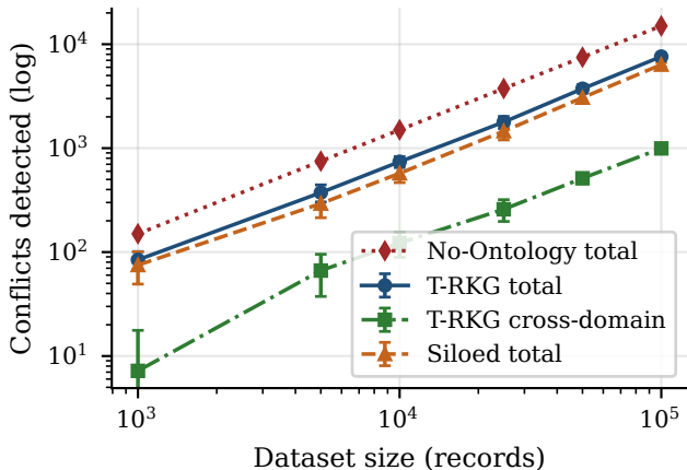
Conflict detection across scales (10 seeds, mean \pm \sigma )
