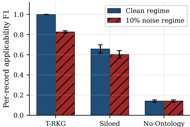
Applicability F1: baseline gap and T-RKG robustness
